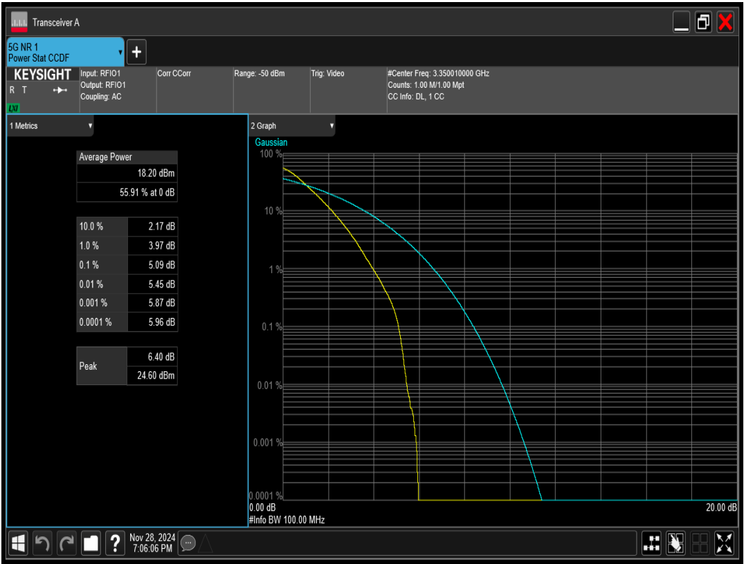
n78 SCS=30kHz DFT_BPSK BW=100MHz Channel=623334 RB=270@0
