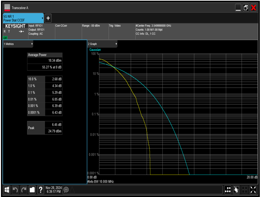
n78 SCS=30kHz DFT_BPSK BW=10MHz Channel=636666 RB=24@0
