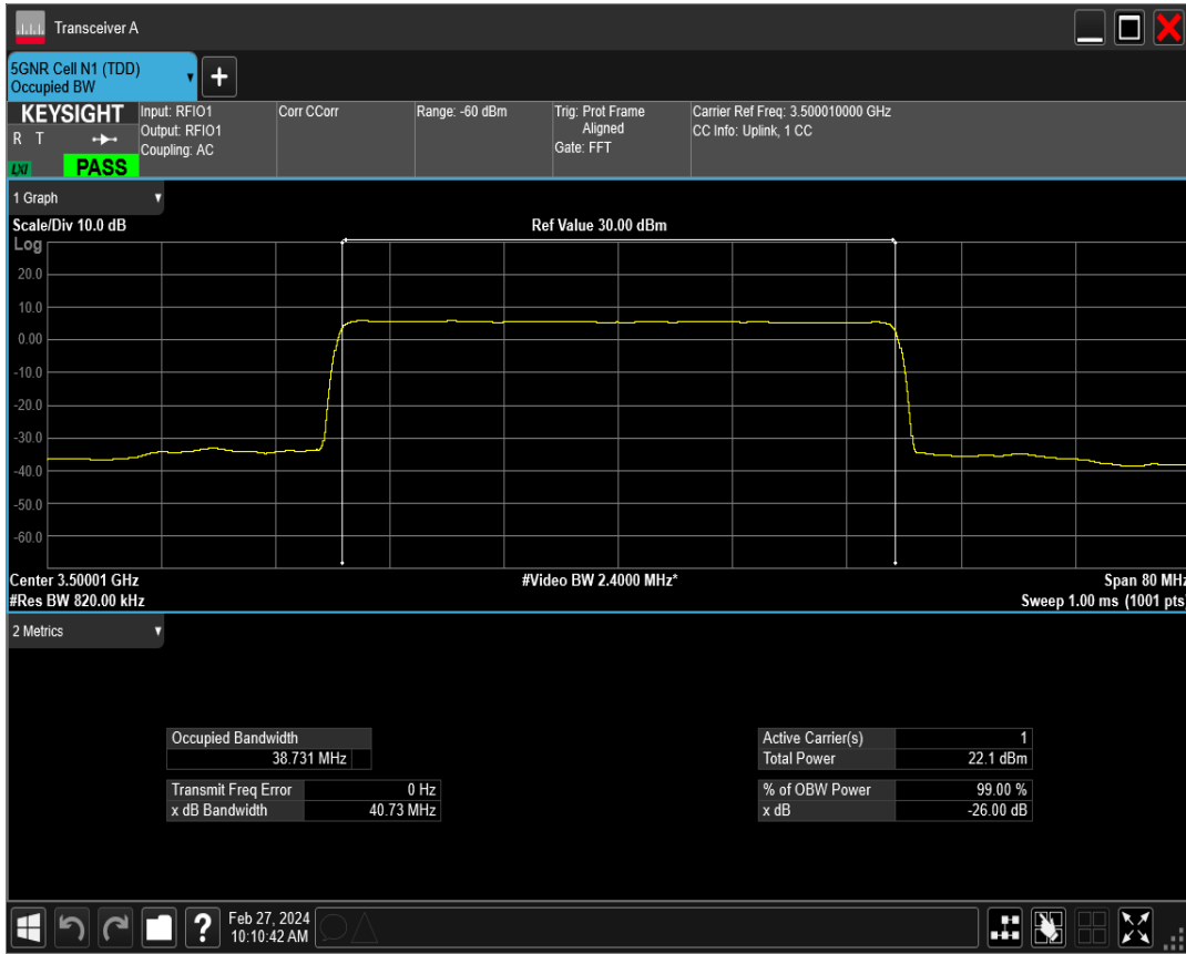
n77(3450-3550) SCS=15kHz CP_QPSK BW=40MHz Channel=633334 RB=216@0
