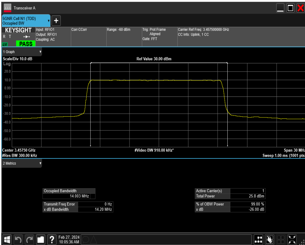
n77(3450-3550) SCS=15kHz DFT_QAM16 BW=15MHz Channel=630500 RB=75@0
