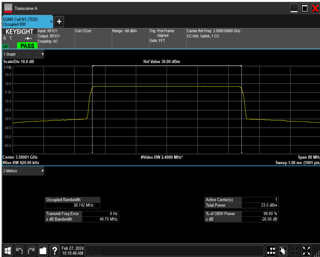
n77(3450-3550) SCS=15kHz DFT_BPSK BW=40MHz Channel=635332 RB=216@0
