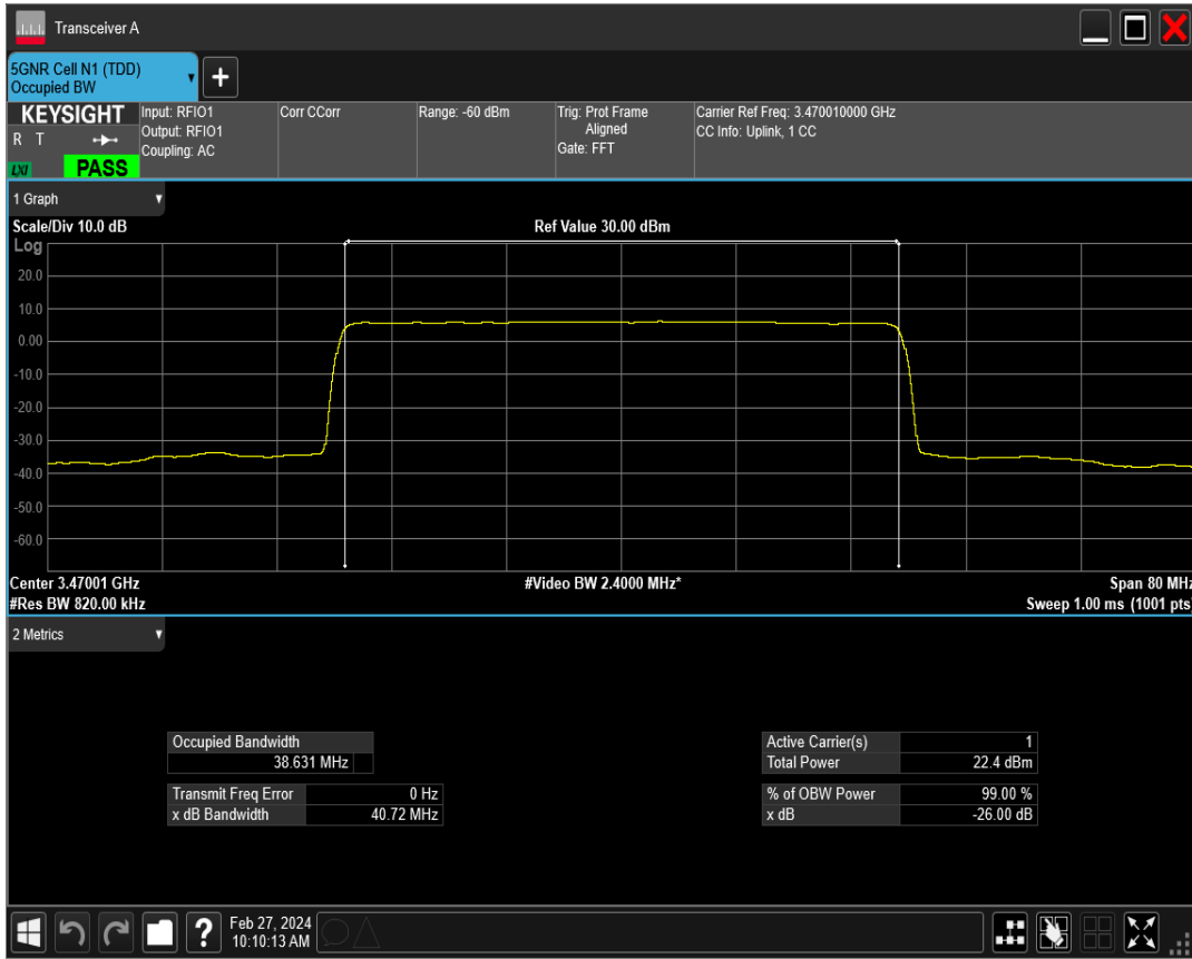
n77(3450-3550) SCS=15kHz CP_QPSK BW=40MHz Channel=631334 RB=216@0
