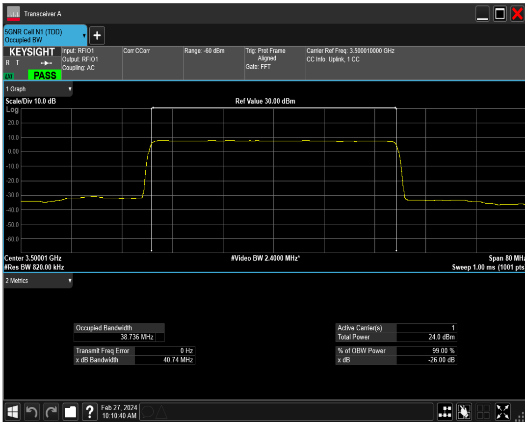
n77(3450-3550) SCS=15kHz DFT_QAM256 BW=40MHz Channel=633334 RB=216@0
