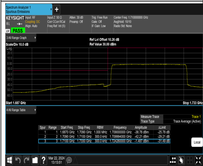
Band66-20MHz-64QAM-132572-1RB#99
