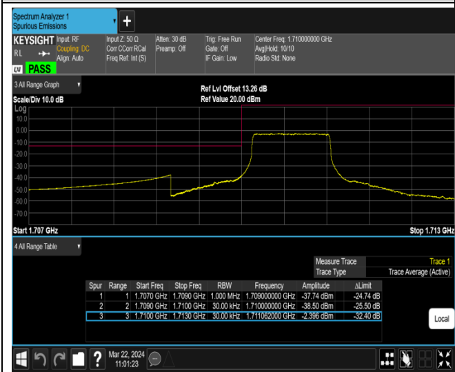
Band66-1.4MHz-64QAM-132665-1RB#5
