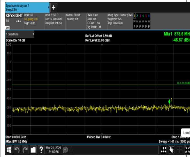
Band7-5MHz-QPSK-21100-1RB#0-Range1:30~1000MHz
