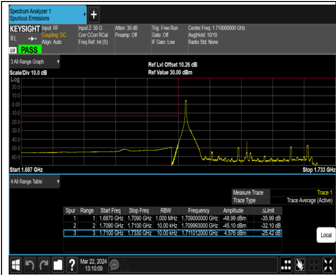
Band66-20MHz-64QAM-132072-100RB#0
