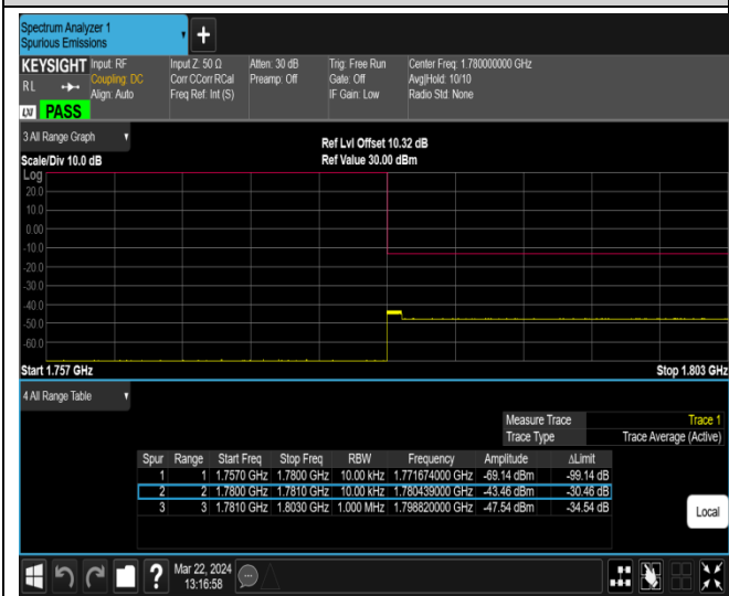
Band66-20MHz-64QAM-132072-1RB#0
