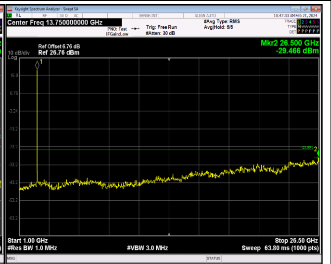
Band7-20MHz-64QAM-21350-1RB#0-Range2:1000~2
