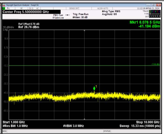
Band12-1.4MHz-64QAM-23095-1RB#0-Range2:1000
