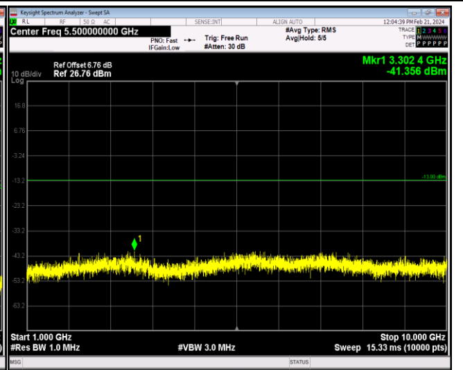
Band12-10MHz-64QAM-23060-1RB#0-Range2:1000~
