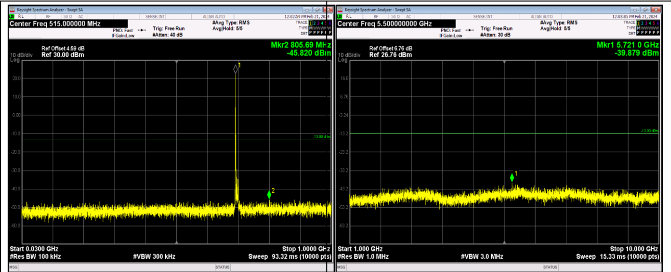
Band12-10MHz-16QAM-23095-1RB#0-Range1:30 ~1000MHz
