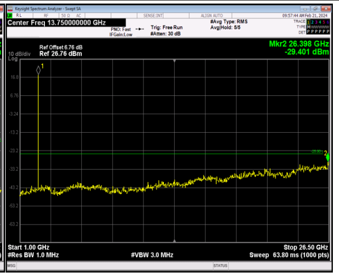
Band7-5MHz-64QAM-21425-1RB#0-Range2:1000~26500MHz
