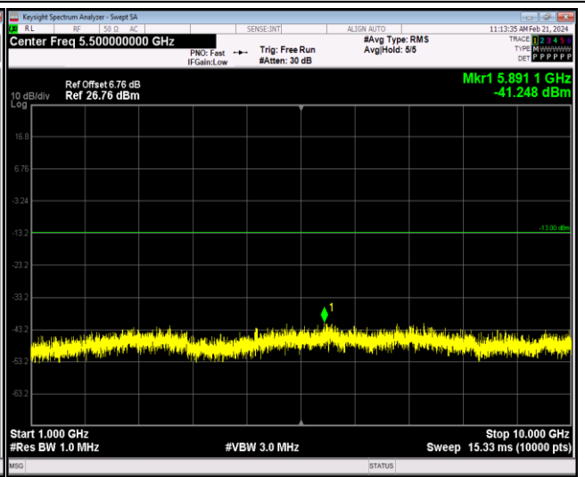
Band12-1.4MHz-64QAM-23017-1RB#0-Range2:1000 ~10000MHz
