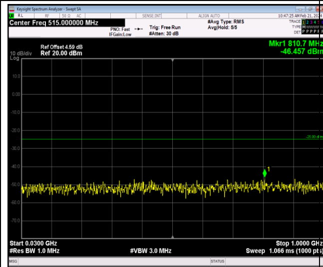
Band7-20MHz-64QAM-21350-1RB#0-Range1:30~
