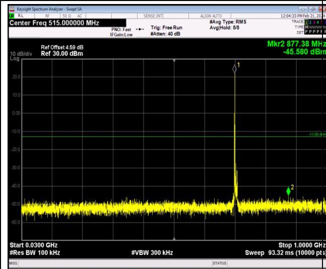
Band12-10MHz-64QAM-23060-1RB#0-Range1:30
