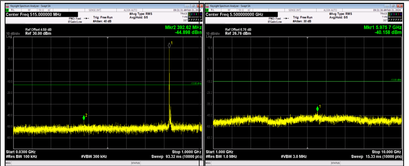
Band5-10MHz-64QAM-20600-1RB#0-Range1:30~1000MHz
