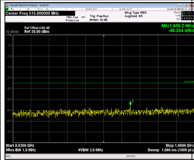
Band7-20MHz-64QAM-21100-1RB#0-Range1:30~1000MHz
