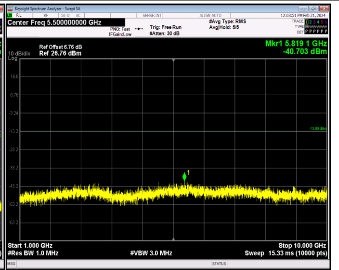
Band12-10MHz-16QAM-23130-1RB#0-Range2:1000~ 10000MHz
