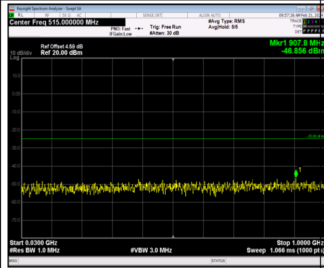
Band7-5MHz-64QAM-21425-1RB#0-Range1:30~1000MHz
