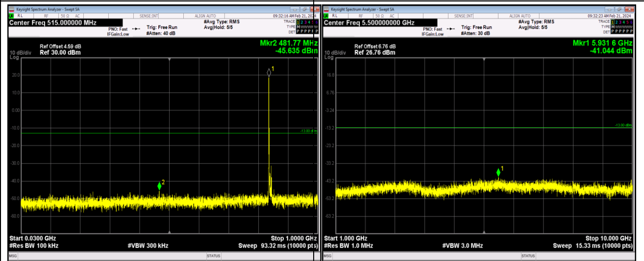
Band7-5MHz-QPSK-20775-1RB#0-Range1:30~1000MHz
