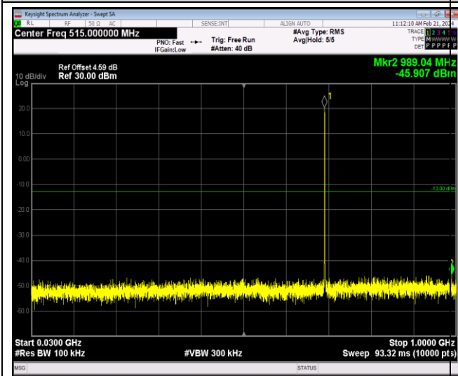
Band12-1.4MHz-64QAM-23095-1RB#0-Range1:30
