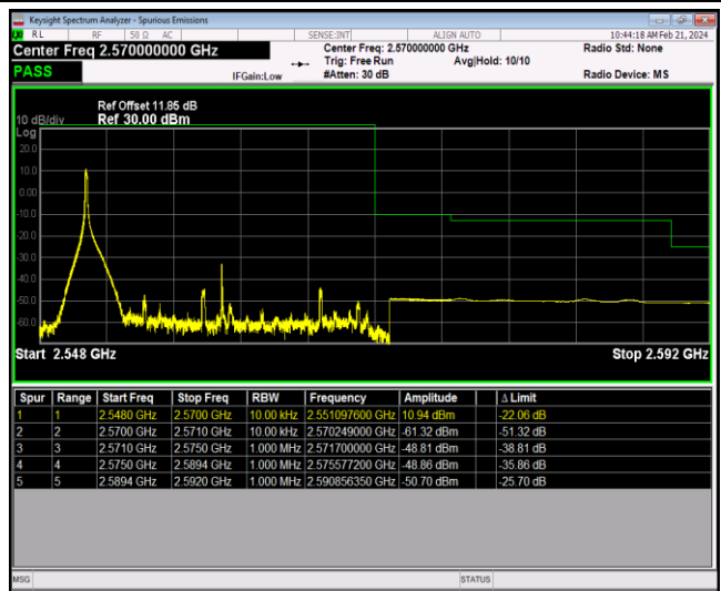
Band7-20MHz-64QAM-21350-100RB#0
