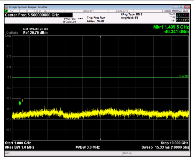
Band17-10MHz-16QAM-23790-1RB#0-Range2:1000~10000MHz
