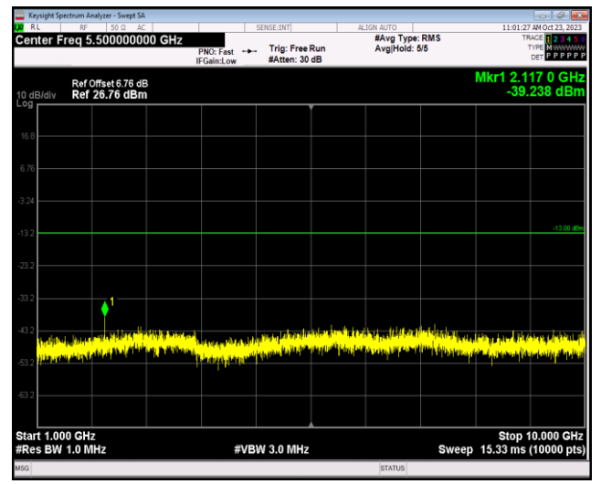
Band17-10MHz-16QAM-23800-1RB#0-Range2:1000~10000MHz
