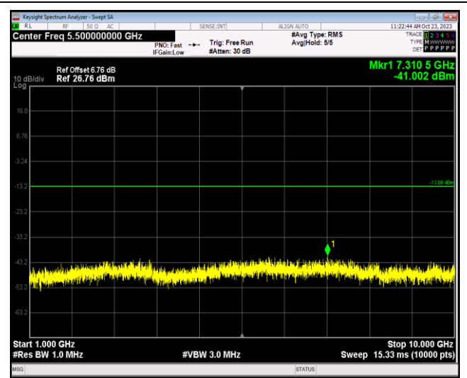
Band26-1.4MHz-QPSK-27033-1RB#0-Range2:1000~10000MHz
