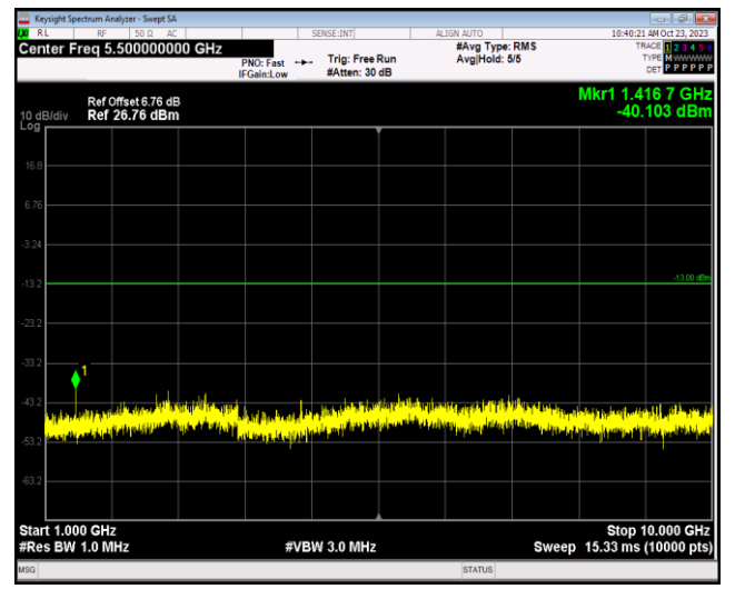
Band17-5MHz-QPSK-23825-1RB#0-Range2:1000~10000MHz
