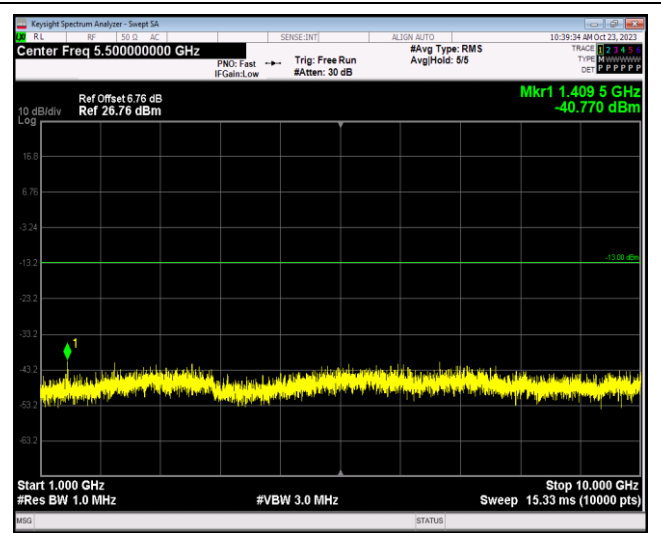
Band17-5MHz-QPSK-23790-1RB#0-Range2:1000~10000MHz
