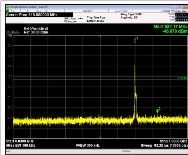
Band17-10MHz-64QAM-23780-1RB#0-Range1:30~1000MHz
