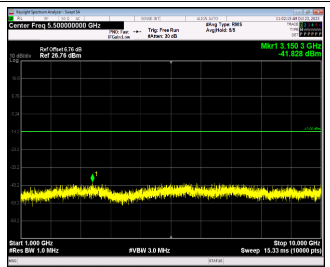
Band17-10MHz-64QAM-23780-1RB#0-Range2:1000~10000MHz
