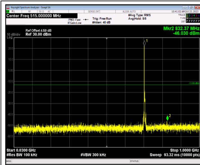
Band17-5MHz-16QAM-23755-1RB#0-Range1:30~1000MHz
