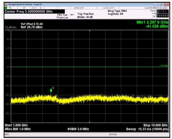
Band26-1.4MHz-QPSK-26915-1RB#0-Range2:1000~10000MHz
