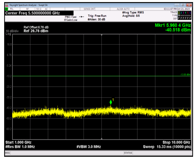
Band26-1.4MHz-QPSK-26783-1RB#0-Range2:1000~10000MHz
