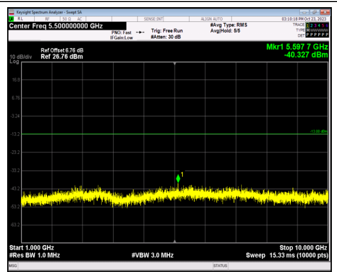
Band26-1.4MHz-QPSK-26740-1RB#0-Range2:1000~10000MHz
