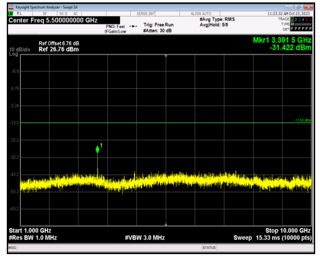
Band26-1.4MHz-16QAM-26697-1RB#0-Range2:1000~10000MHz
