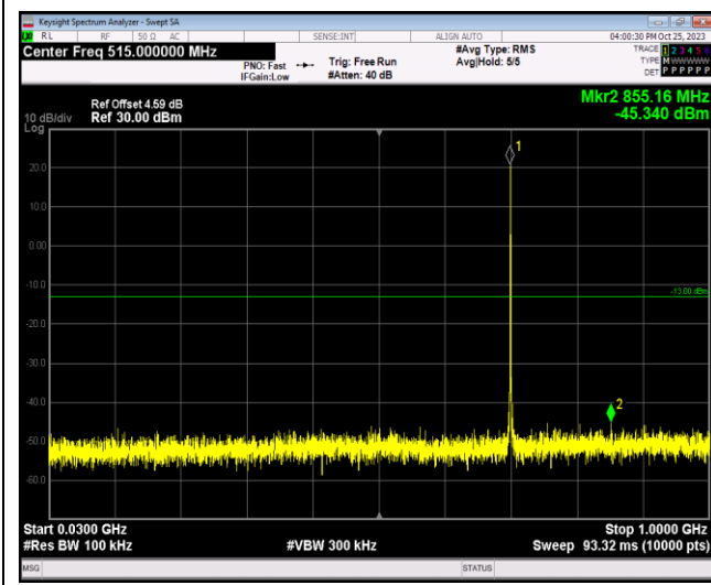
Band12-1.4MHz-64QAM-23173-1RB#0-Range1:30 ~1000MHz
