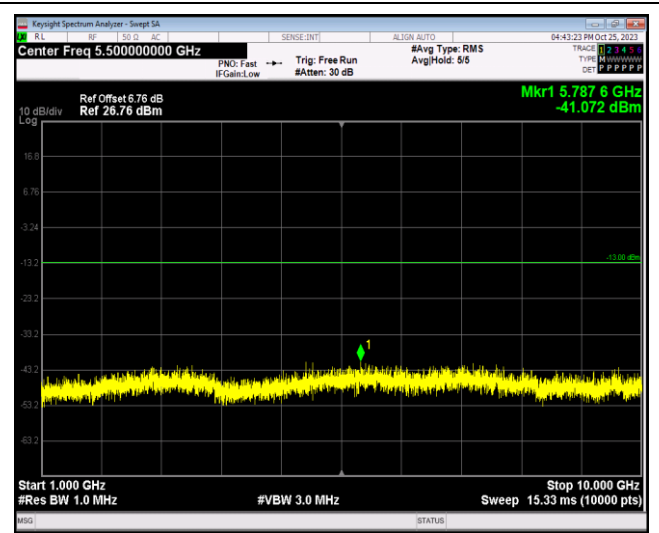
Band12-10MHz-64QAM-23130-1RB#0-Range2:1000~10000MHz
