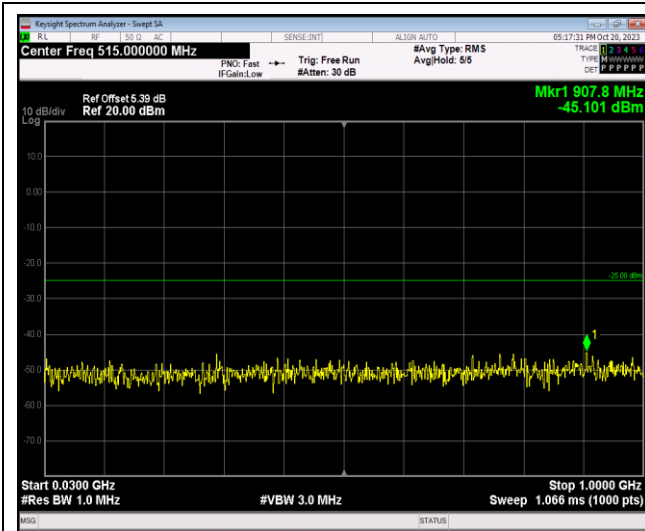
Band7-20MHz-64QAM-20850-1RB#0-Range1:30~1000MHz
