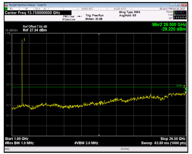
Band7-20MHz-64QAM-21100-1RB#0-Range2:1000~26500MHz
