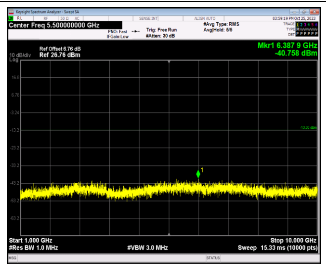
Band12-1.4MHz-QPSK-23095-1RB#0-Range2:1000~10000MHz
