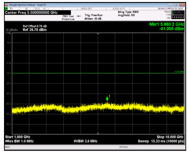
Band13-5MHz-QPSK-23205-1RB#0-Range2:1000~10000MHz
