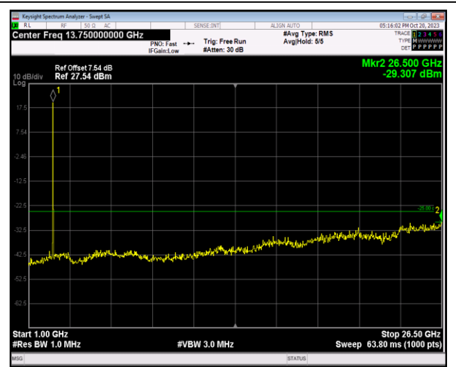
Band7-20MHz-16QAM-21100-1RB#0-Range2:1000~26500MHz
