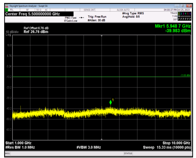
Band12-1.4MHz-64QAM-23173-1RB#0-Range2:1000 ~10000MHz
