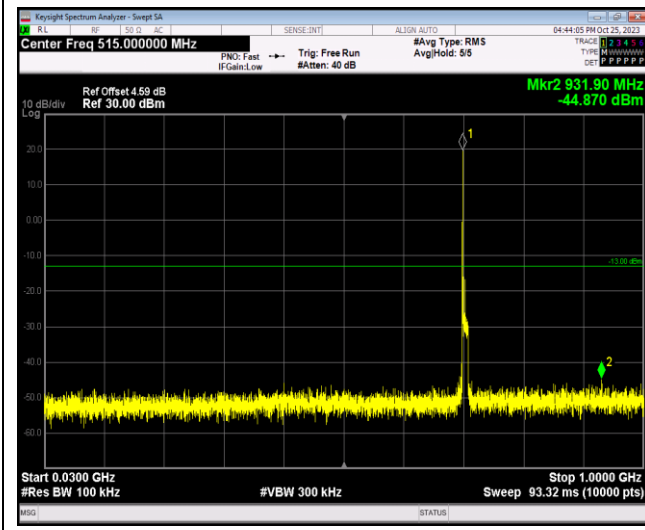
Band13-5MHz-QPSK-23205-1RB#0-Range1:30~1000MHz
