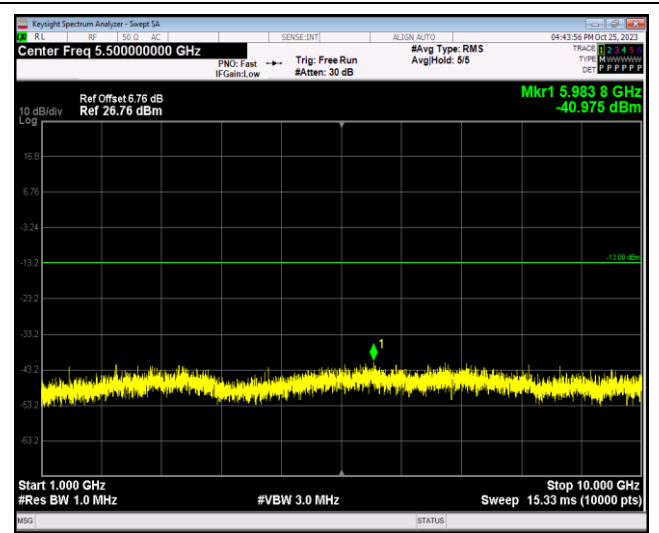
Band12-10MHz-64QAM-23060-1RB#0-Range2:1000~10000MHz
