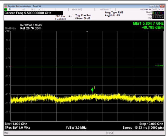
Band12-1.4MHz-64QAM-23095-1RB#0-Range2:1000 ~10000MHz
