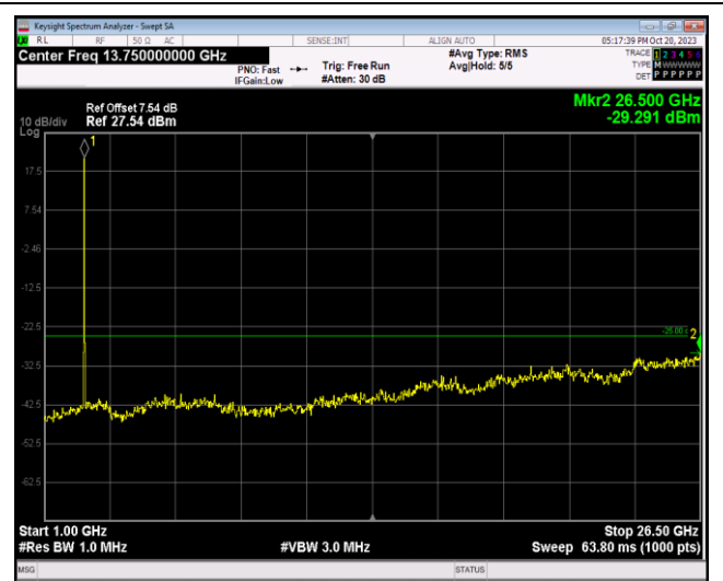
Band7-20MHz-64QAM-20850-1RB#0-Range2:1000~26500MHz
