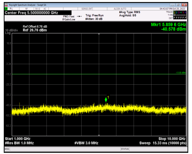
Band12-10MHz-16QAM-23130-1RB#0-Range2:1000~10000MHz
