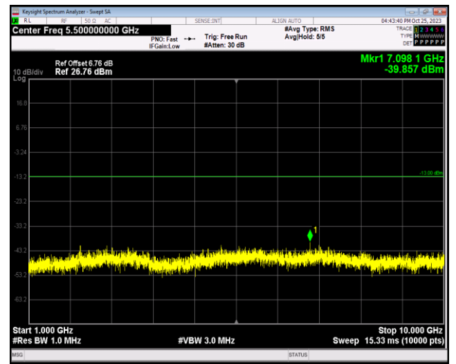
Band12-10MHz-16QAM-23060-1RB#0-Range2:1000~10000MHz
