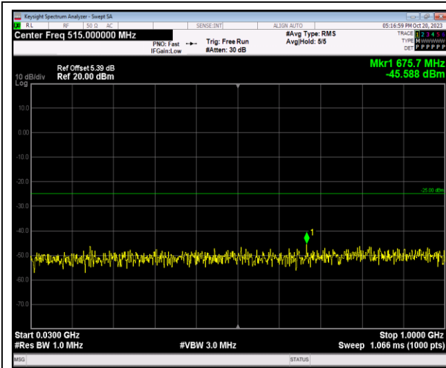
Band7-20MHz-64QAM-21350-1RB#0-Range1:30~1000MHz
