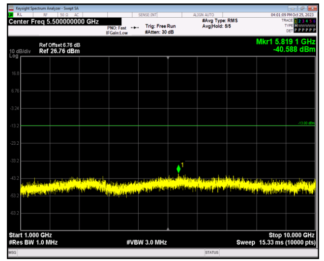
Band12-1.4MHz-64QAM-23017-1RB#0-Range2:1000 ~10000MHz
