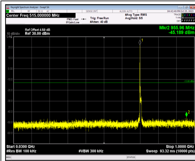
Band12-10MHz-64QAM-23060-1RB#0-Range1:30~1000MHz
