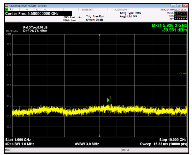
Band12-10MHz-64QAM-23095-1RB#0-Range2:1000~10000MHz
