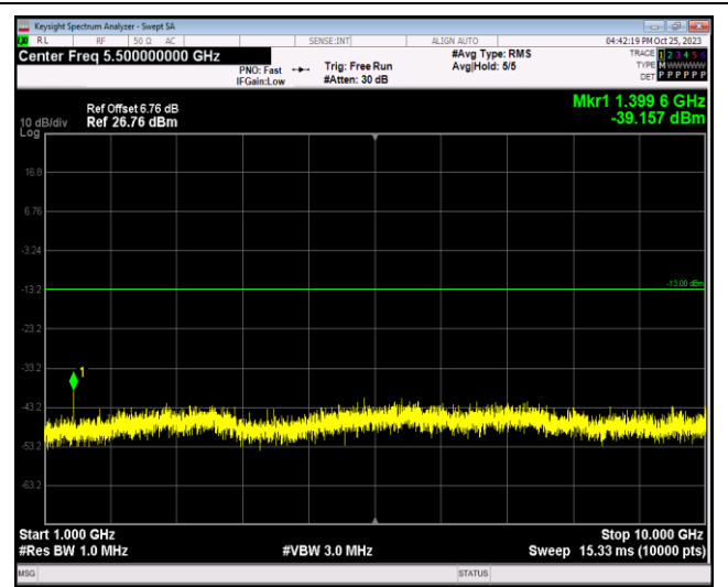
Band12-10MHz-16QAM-23095-1RB#0-Range2:1000~10000MHz
