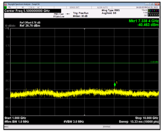
Band12-1.4MHz-QPSK-23173-1RB#0-Range2:1000~10000MHz
