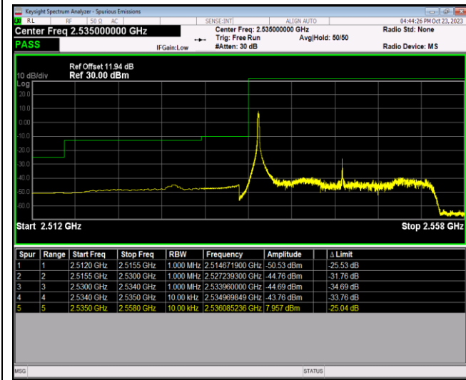
Band41-20MHz-16QAM-40140-100RB#0
