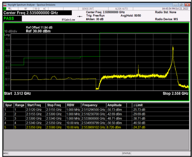
Band41-20MHz-16QAM-41140-1RB#0
