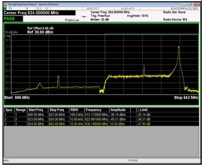
Band26-15MHz-64QAM-26965-1RB#0
