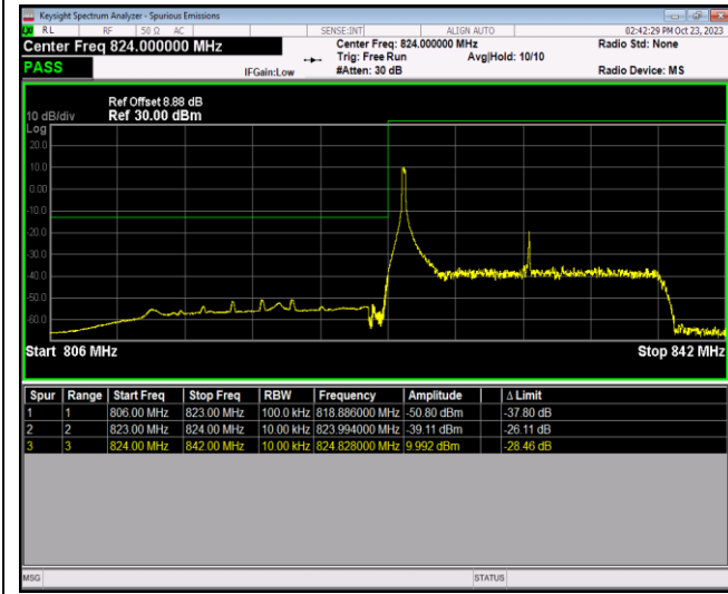
Band26-15MHz-64QAM-26865-75RB#0
