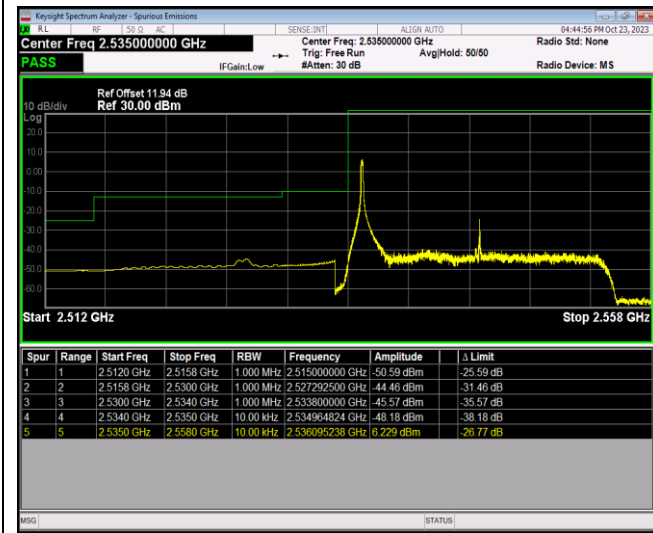
Band41-20MHz-64QAM-40140-100RB#0
