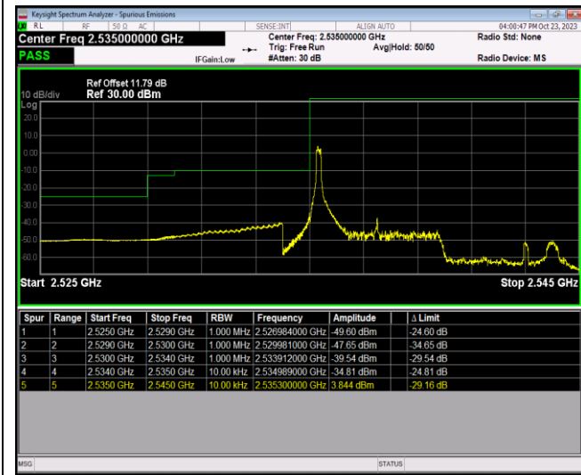
Band41-5MHz-16QAM-40065-25RB#0
