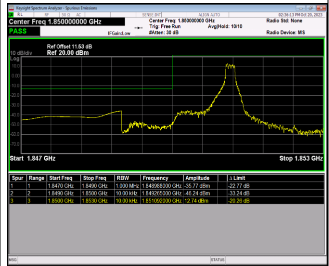
Band2-1.4MHz-64QAM-18607-6RB#5
