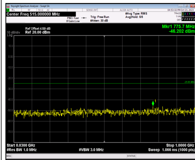
Band41-20MHz-QPSK-40640-1RB#0-Range1:30~1000MHz
