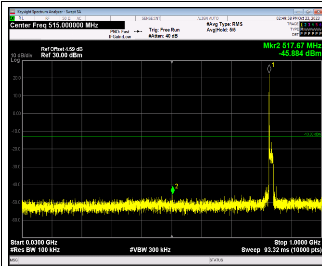
Band26-15MHz-QPSK-26965-1RB#0-Range1:30~1000MHz
