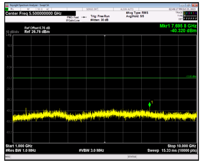
Band26-15MHz-QPSK-26915-1RB#0-Range2:1000~10000MHz
