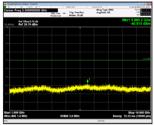
Band26-1.4MHz-64QAM-26915-1RB#0-Range2:1000 ~10000MHz
