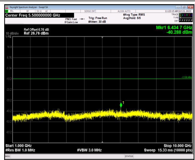
Band26-1.4MHz-64QAM-27033-1RB#0-Range2:1000 ~10000MHz
