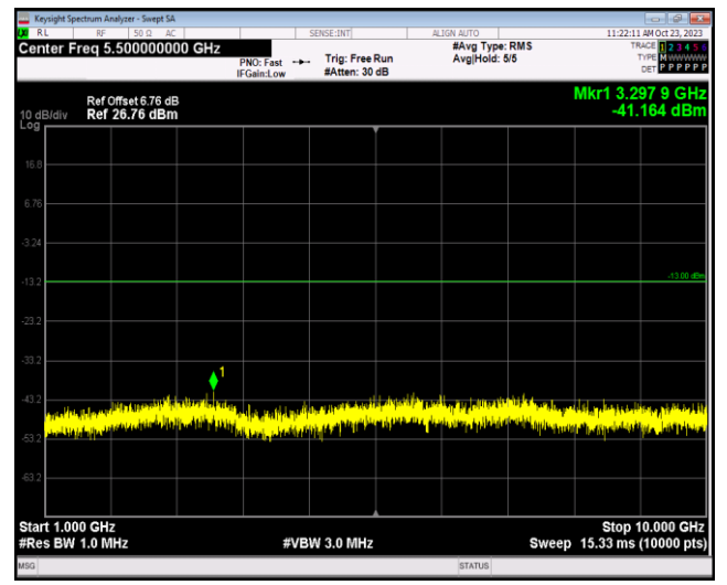
Band26-1.4MHz-16QAM-26915-1RB#0-Range2:1000 ~10000MHz
