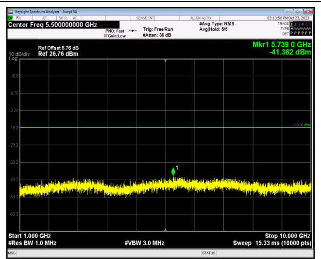
Band26-1.4MHz-64QAM-26740-1RB#0-Range2:1000 ~10000MHz
