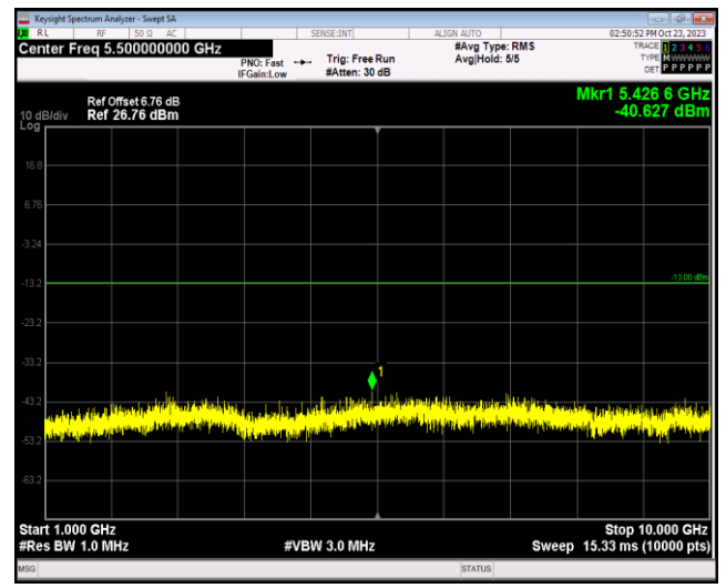
Band26-15MHz-16QAM-26865-1RB#0-Range2:1000~10000MHz
