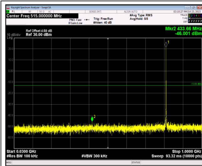
Band26-1.4MHz-16QAM-26740-1RB#0-Range1:30 ~1000MHz
