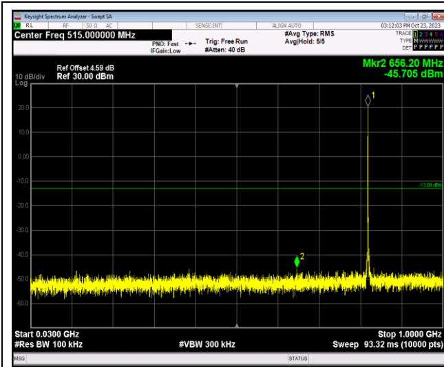
Band26-1.4MHz-16QAM-26797-1RB#0-Range1:30 ~1000MHz
