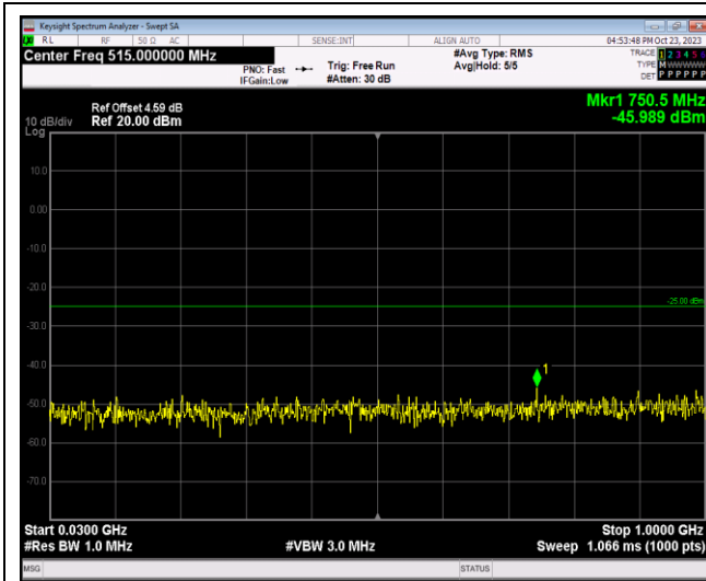
Band41-20MHz-16QAM-40640-1RB#0-Range1:30~1000MHz
