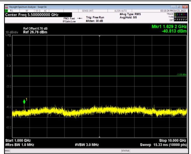
Band26-1.4MHz-16QAM-26740-1RB#0-Range2:1000 ~10000MHz
