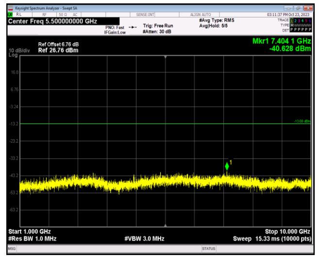
Band26-1.4MHz-64QAM-26783-1RB#0-Range2:1000 ~10000MHz
