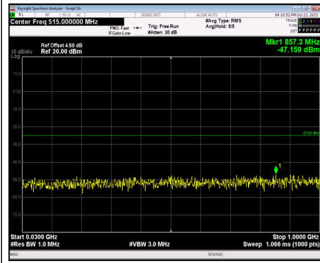
Band41-5MHz-64QAM-41215-1RB#0-Range1:30~1000MHz
