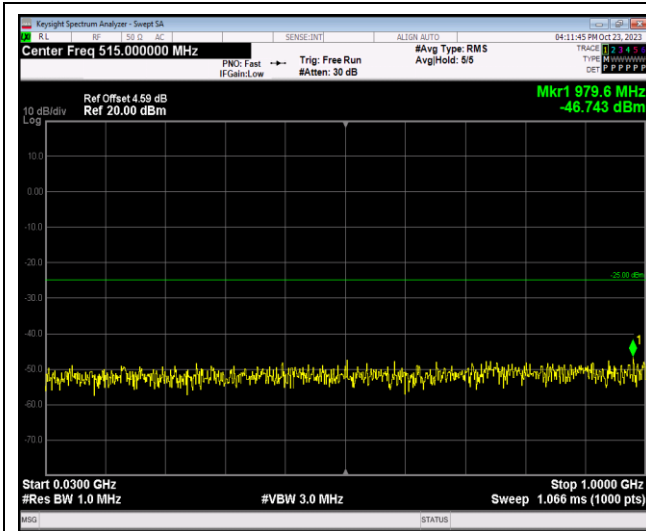
Band41-20MHz-QPSK-40140-1RB#0-Range1:30~1000MHz
