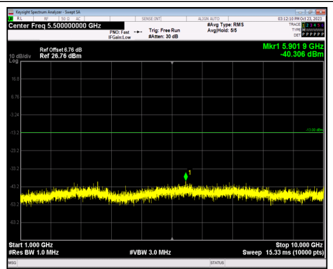
Band26-1.4MHz-16QAM-26797-1RB#0-Range2:1000 ~10000MHz
