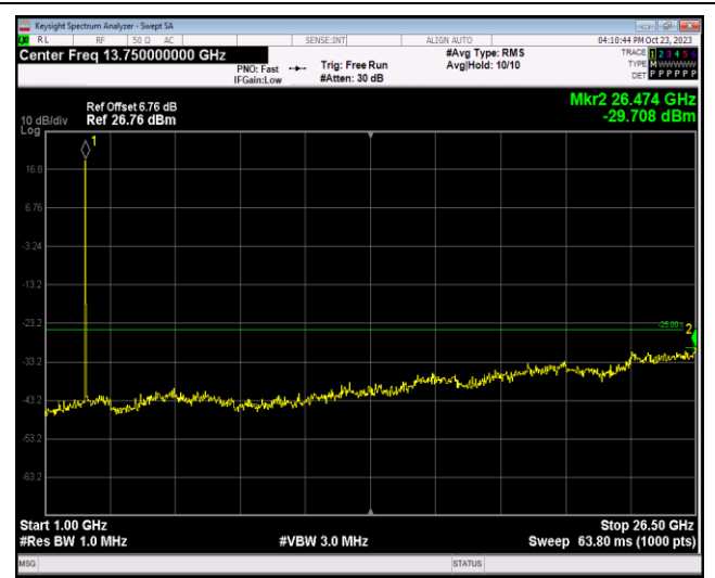
Band41-5MHz-16QAM-41215-1RB#0-Range2:1000~26500MHz
