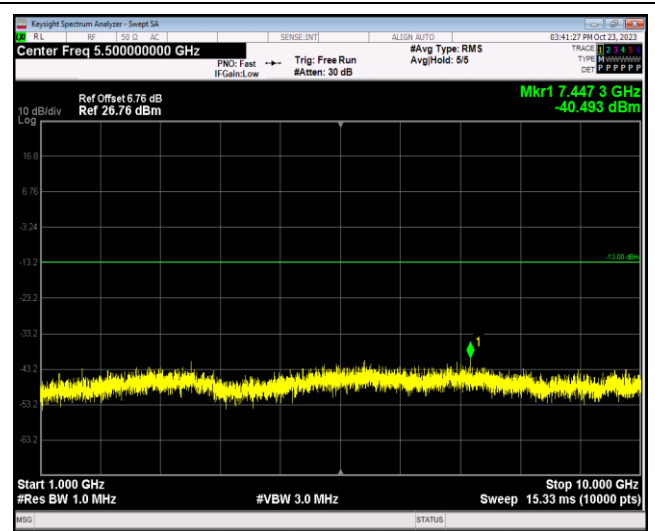
Band26-10MHz-16QAM-26740-1RB#0-Range2:1000~10000MHz
