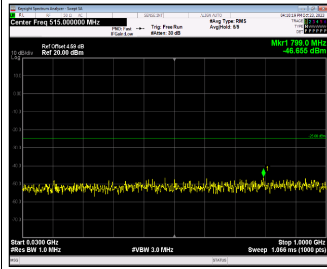
Band41-5MHz-QPSK-41215-1RB#0-Range1:30~1000MHz
