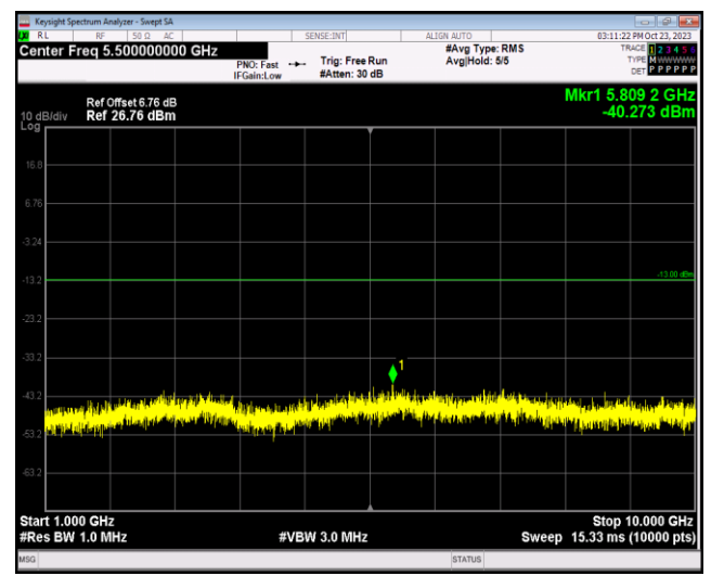
Band26-1.4MHz-16QAM-26783-1RB#0-Range2:1000 ~10000MHz
