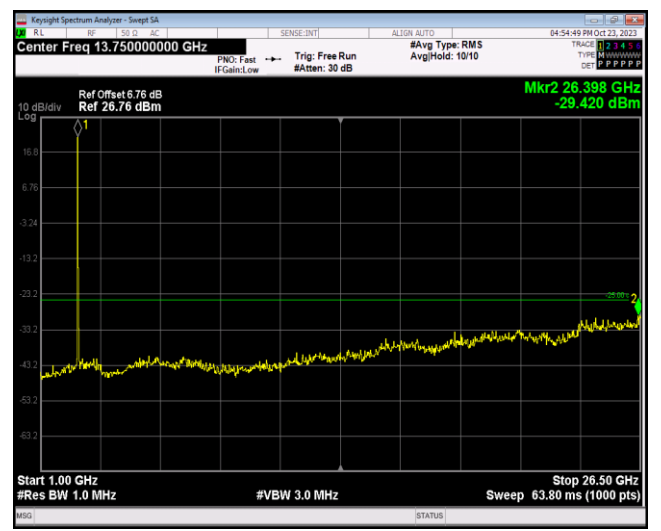
Band41-20MHz-16QAM-41140-1RB#0-Range2:1000~26500MHz
