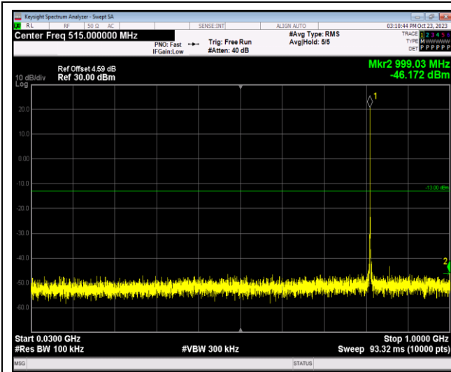
Band26-1.4MHz-64QAM-26740-1RB#0-Range1:30 ~1000MHz
