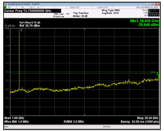
Band41-5MHz-64QAM-41215-1RB#0-Range2:1000~26500MHz
