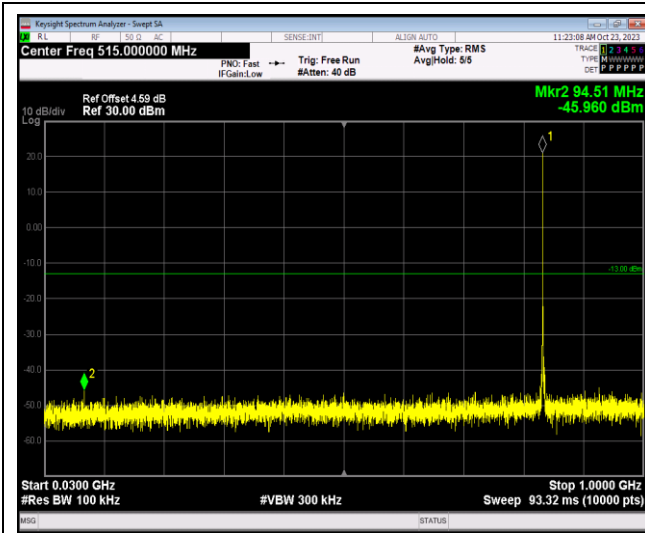
Band26-1.4MHz-64QAM-27033-1RB#0-Range1:30 ~1000MHz
