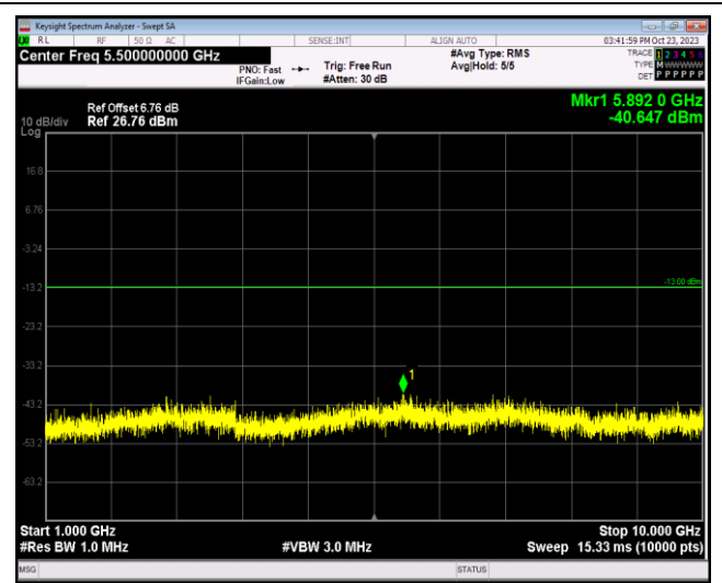
Band26-15MHz-QPSK-26865-1RB#0-Range2:1000~10000MHz
