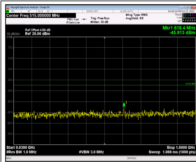
Band41-5MHz-QPSK-40640-1RB#0-Range1:30~1000MHz
