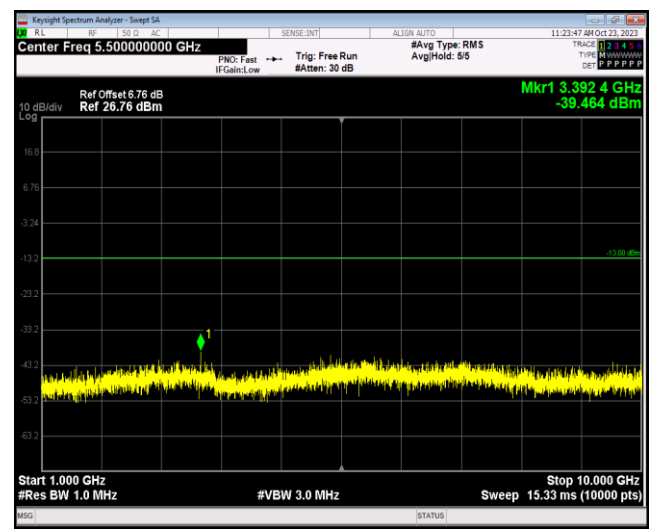
Band26-1.4MHz-64QAM-26697-1RB#0-Range2:1000 ~10000MHz
