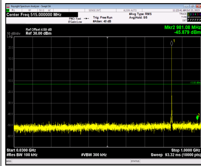
Band26-1.4MHz-64QAM-26697-1RB#0-Range1:30 ~1000MHz
