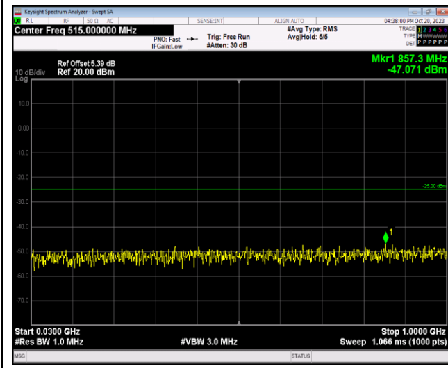
Band7-5MHz-16QAM-21100-1RB#0-Range1:30~1000MHz
