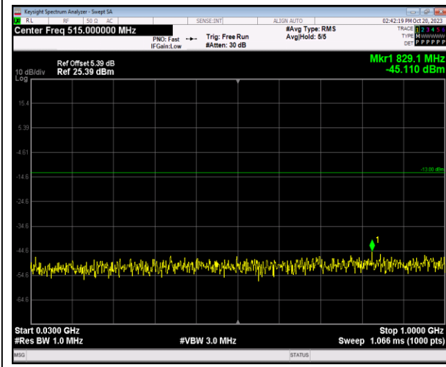
Band2-1.4MHz-64QAM-19193-1RB#0-Range1:30~1000MHz
