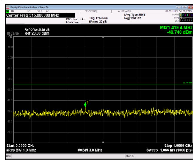
Band7-5MHz-QPSK-21100-1RB#0-Range1:30~100 OMHz
