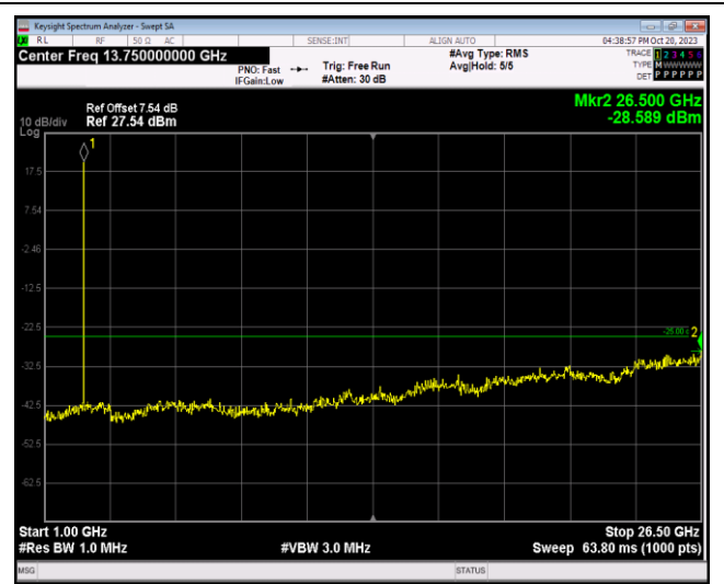
Band7-5MHz-16QAM-21425-1RB#0-Range2:1000~26500MHz
