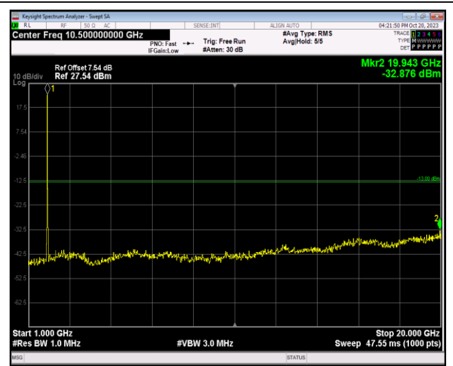
Band2-20MHz-64QAM-19100-1RB#0-Range2:1000~20000MHz
