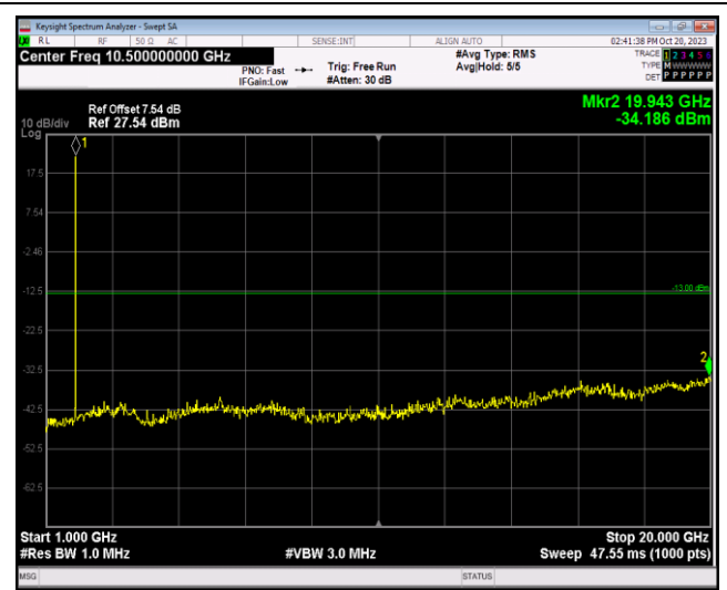
Band2-1.4MHz-64QAM-18900-1RB#0-Range2:1000~20000MHz
