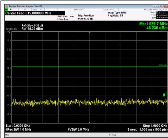
Band2-20MHz-64QAM-18700-1RB#0-Range1:30~1000MHz
