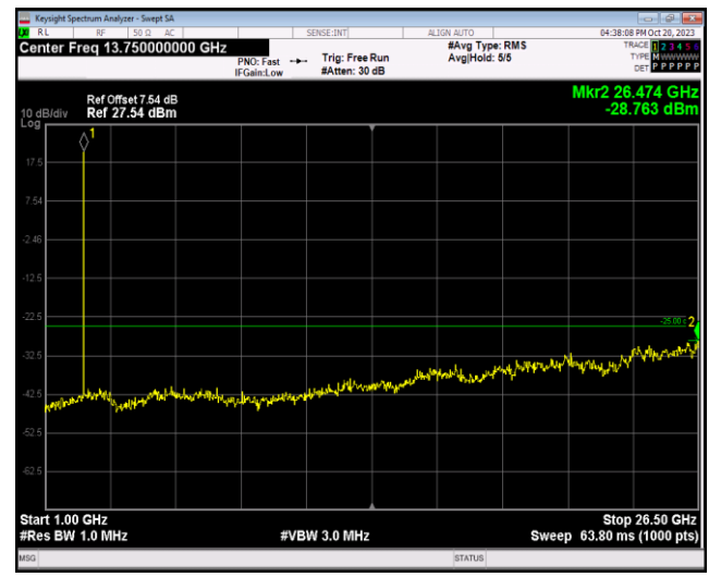
Band7-5MHz-16QAM-21100-1RB#0-Range2:1000~26500MHz
