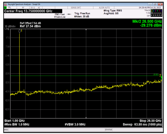
Band7-5MHz-64QAM-20775-1RB#0-Range2:1000~26500MHz
