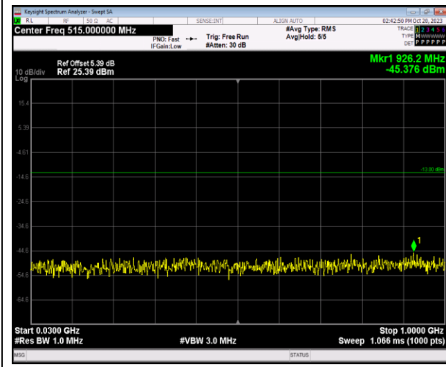
Band2-1.4MHz-64QAM-18607-1RB#0-Range1:30~1000MHz
