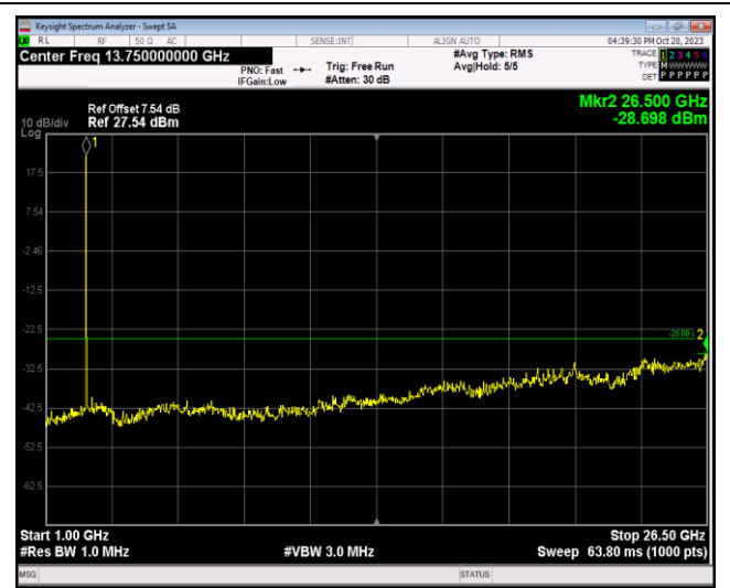
Band7-5MHz-16QAM-20775-1RB#0-Range2:1000~26500MHz
