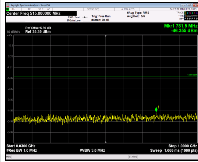
Band7-5MHz-QPSK-20775-1RB#0-Range1:30~1000MHz
