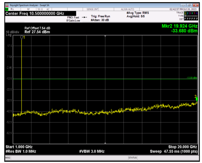
Band2-1.4MHz-64QAM-18607-1RB#0-Range2:1000~20000MHz
