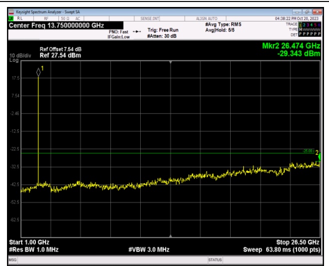
Band7-5MHz-64QAM-21100-1RB#0-Range2:1000~26500MHz
