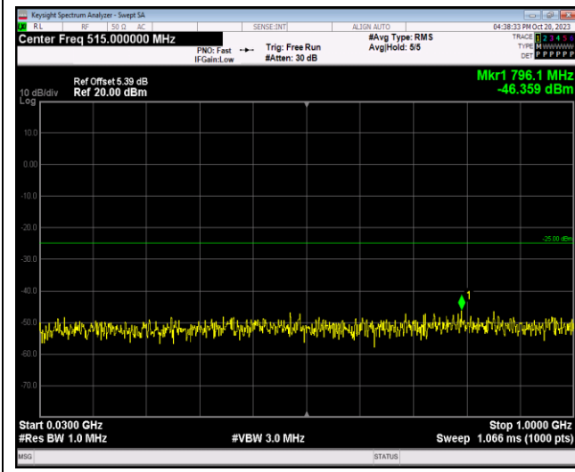
Band7-5MHz-QPSK-21425-1RB#0-Range1:30~100 OMHz
