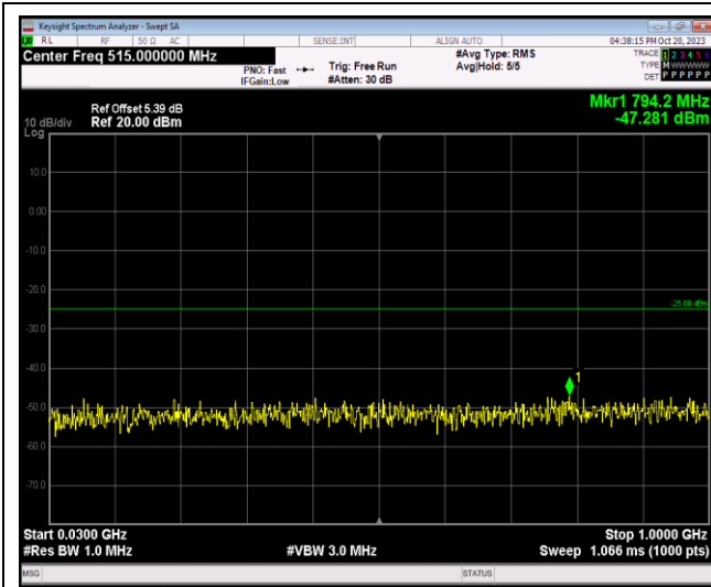
Band7-5MHz-64QAM-21100-1RB#0-Range1:30~1000MHz
