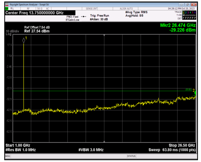
Band7-5MHz-64QAM-21425-1RB#0-Range2:1000~26500MHz
