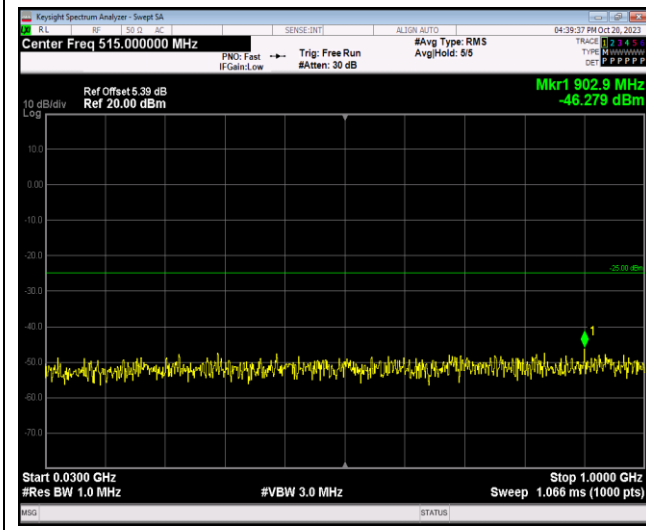
Band7-5MHz-64QAM-20775-1RB#0-Range1:30~1000MHz
