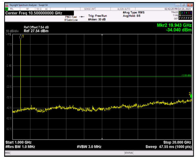
Band2-1.4MHz-64QAM-19193-1RB#0-Range2:1000~20000MHz
