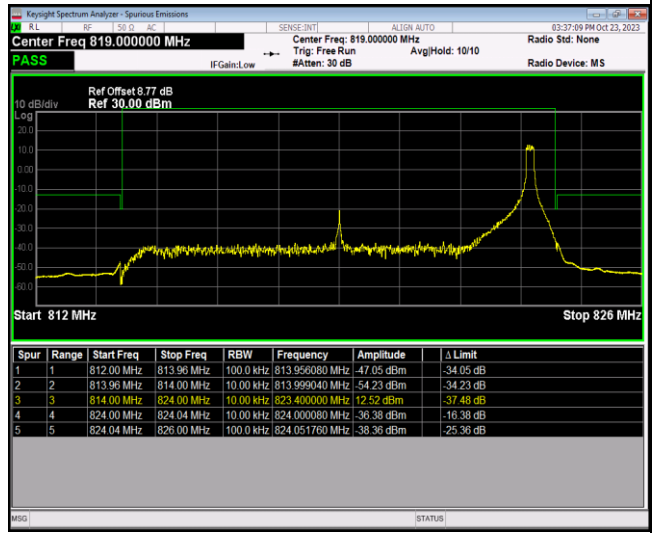
Band26-10MHz-64QAM-26740-1RB#0
