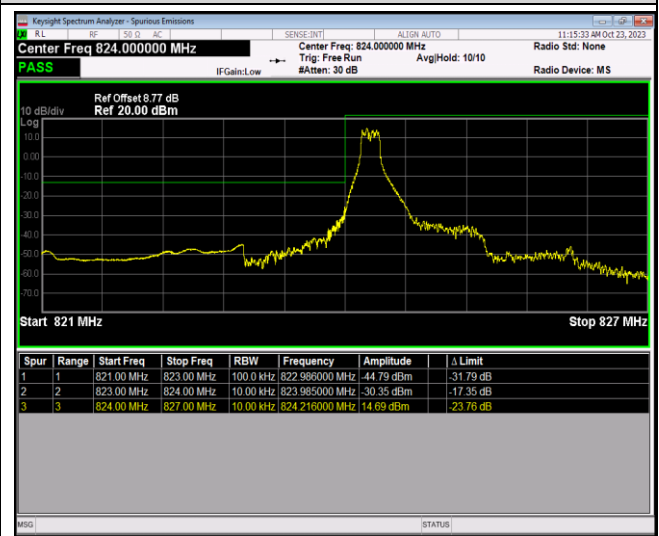
Band26-1.4MHz-QPSK-26797-6RB#0
