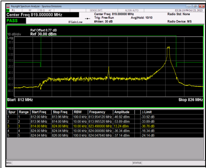
Band26-10MHz-16QAM-26740-1RB#0
