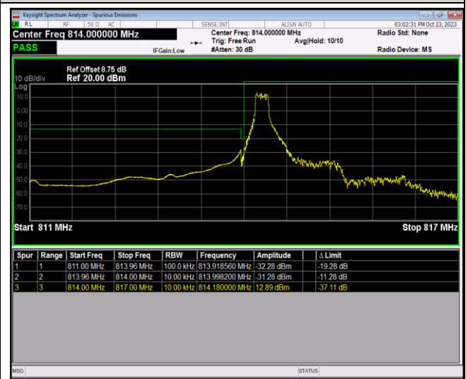
Band26-1.4MHz-16QAM-26697-6RB#0
