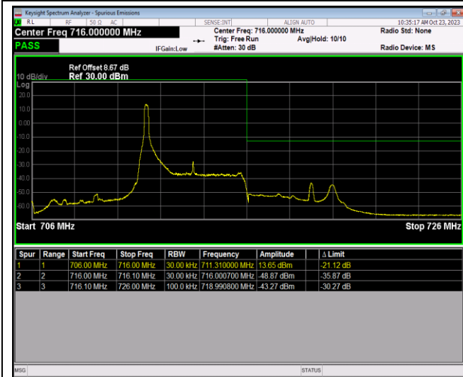
Band17-5MHz-64QAM-23825-25RB#0
