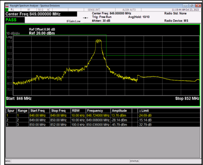
Band26-1.4MHz-64QAM-26697-1RB#0
