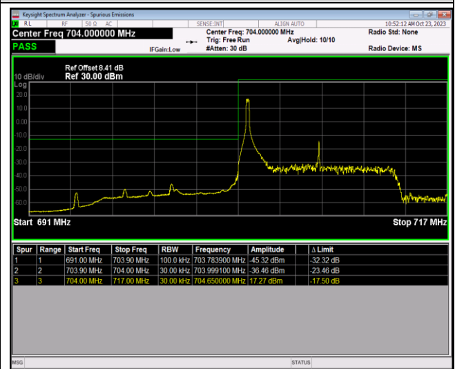
Band17-10MHz-QPSK-23780-50RB#0
