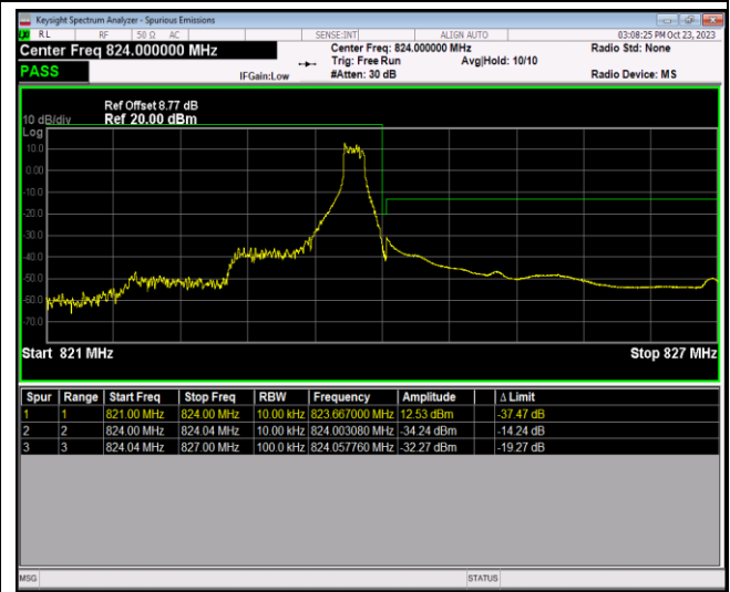
Band26-1.4MHz-64QAM-26797-1RB#0
