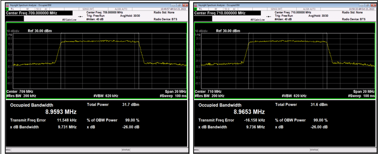
Band17-10MHz-16QAM-23800-50RB#0
