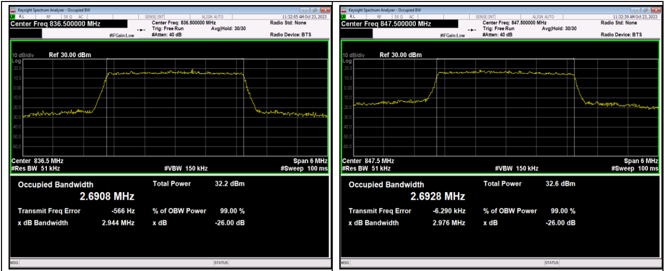
Band26-3MHz-16QAM-26705-15RB#0
