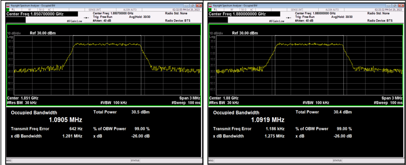
Band2-1.4MHz-64QAM-19193-6RB#0
