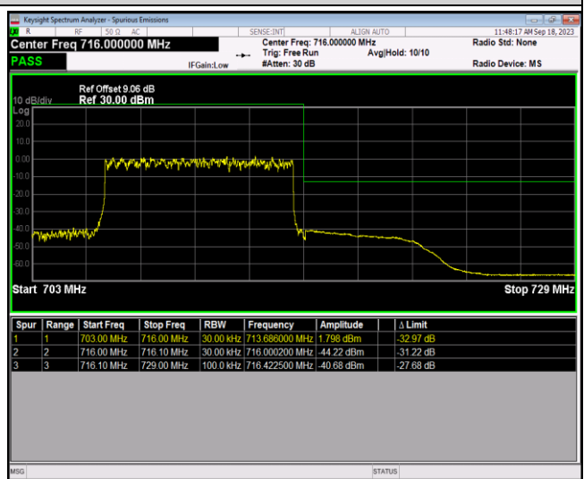
Band17-10MHz-16QAM-23780-1RB#49
