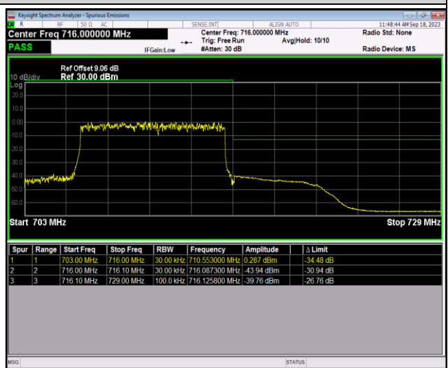
Band17-10MHz-64QAM-23780-1RB#49
