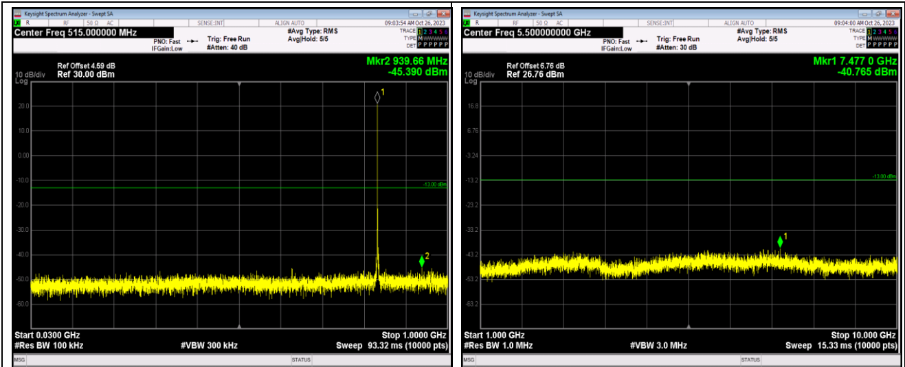
Band26-1.4MHz-QPSK-27033-1RB#0-Range1:30~1000MHz
