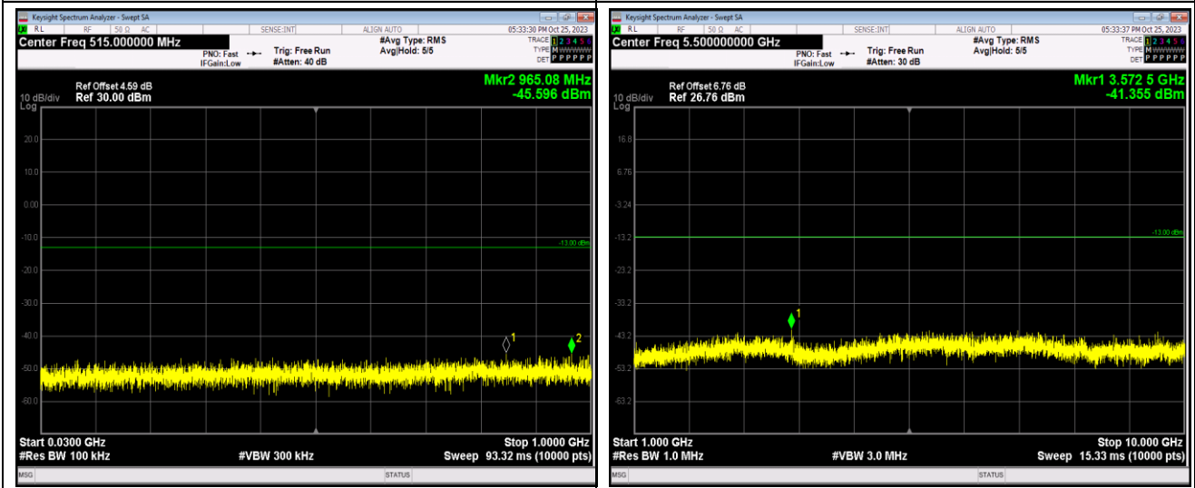
Band13-5MHz-64QAM-23205-1RB#0-Range1:30~1000MHz
