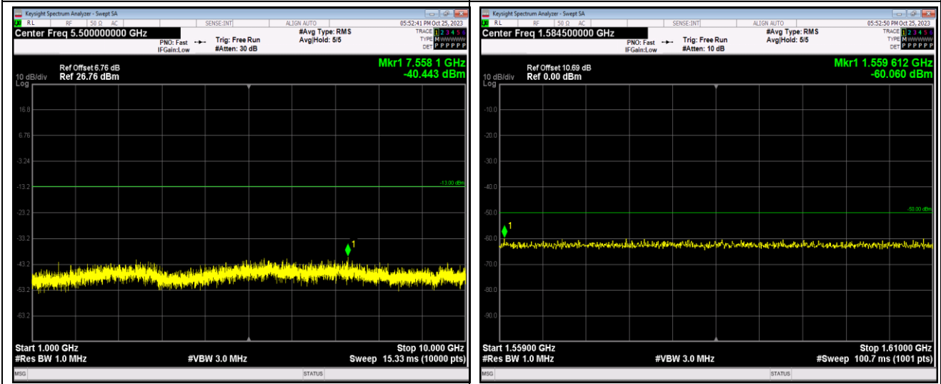
Band13-10MHz-QPSK-23230-1RB#0-Range2:1000 ~10000MHz
