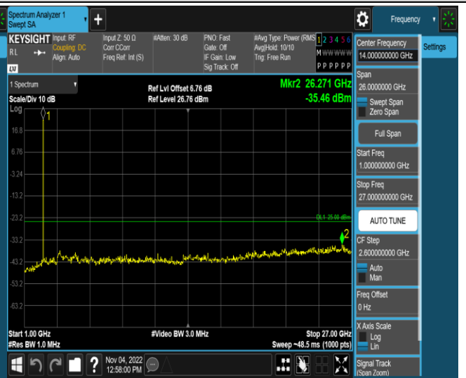
Band41-5MHz-16QAM-40620-1RB#0-Range2:1000~27000MHz
