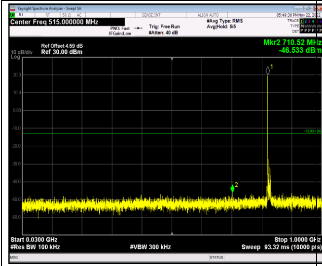
Band5-10MHz-64QAM-20525-1RB#0-Range1:30~1000MHz
