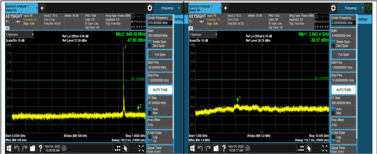
Band5-10MHz-64QAM-20450-1RB#0-Range1:30~1000MHz
