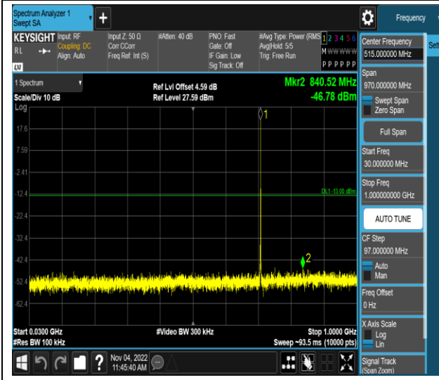
Band12-1.4MHz-16QAM-23173-1RB#0-Range1:30 ~1000MHz
