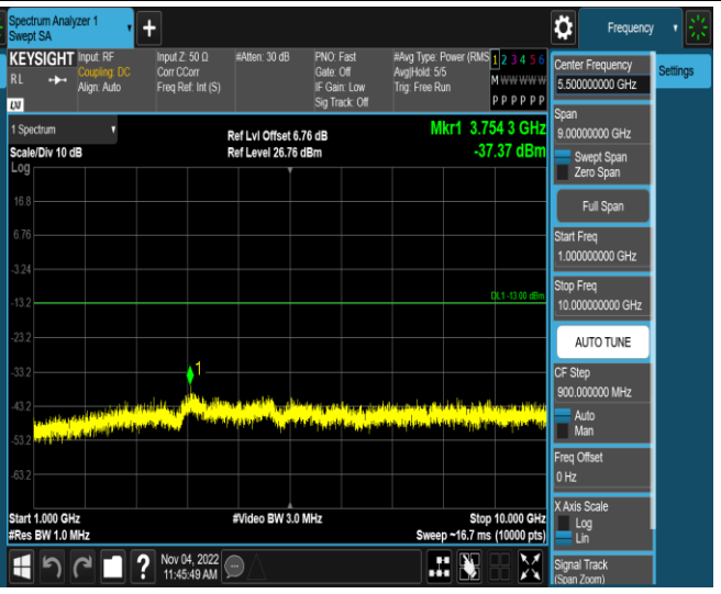
Band12-1.4MHz-16QAM-23173-1RB#0-Range2:1000 ~10000MHz
