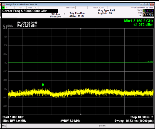
Band5-10MHz-64QAM-20525-1RB#0-Range2:1000~10000MHz
