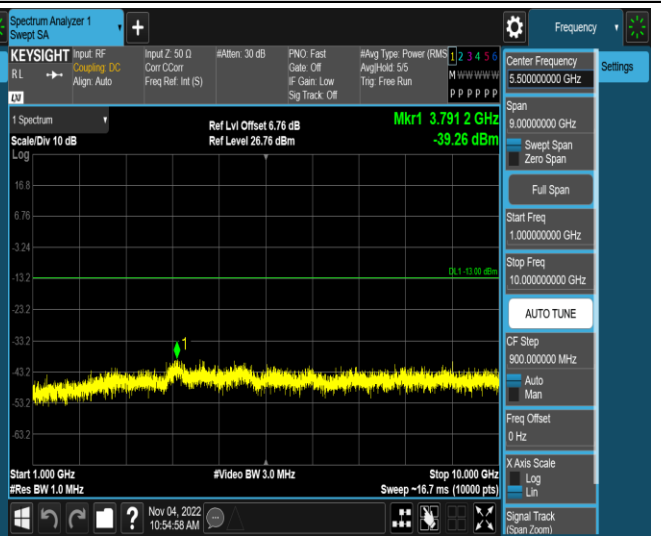
Band5-10MHz-QPSK-20600-1RB#0-Range2:1000~10000MHz
