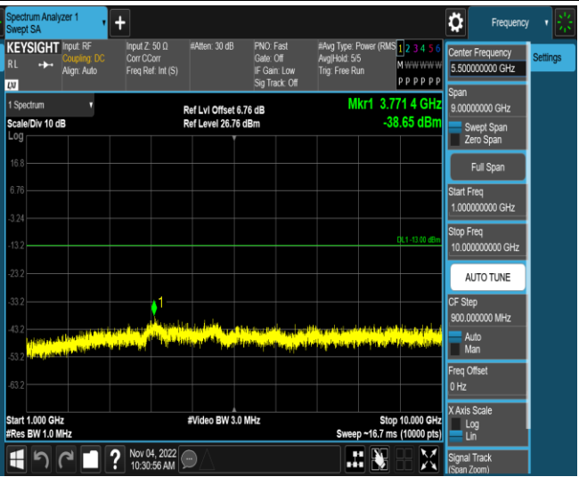
Band5-1.4MHz-QPSK-20525-1RB#0-Range2:1000~10000MHz
