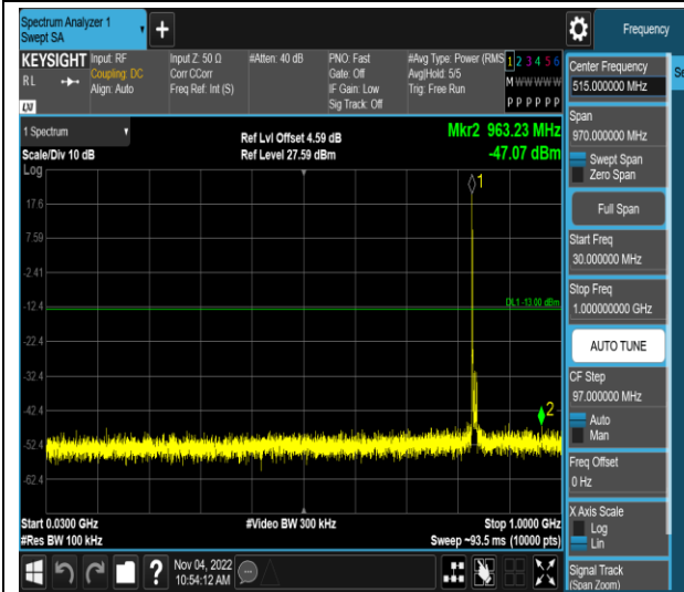
Band5-10MHz-QPSK-20600-1RB#0-Range1:30~1000MHz
