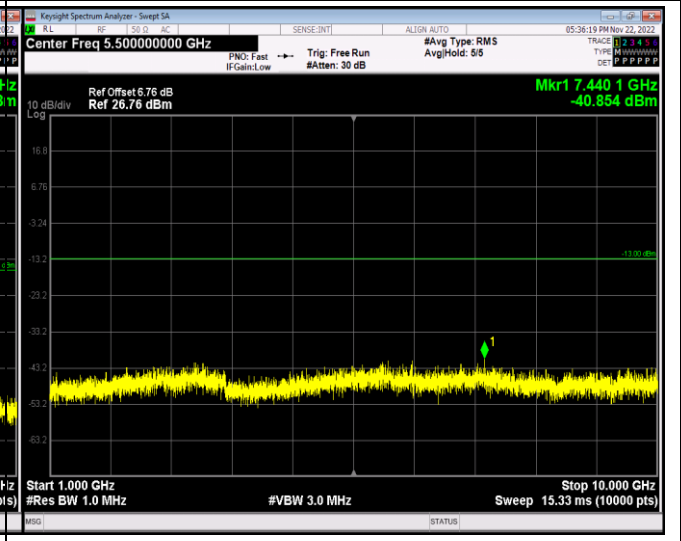
Band5-1.4MHz-64QAM-20407-1RB#0-Range2:1000~10000MHz
