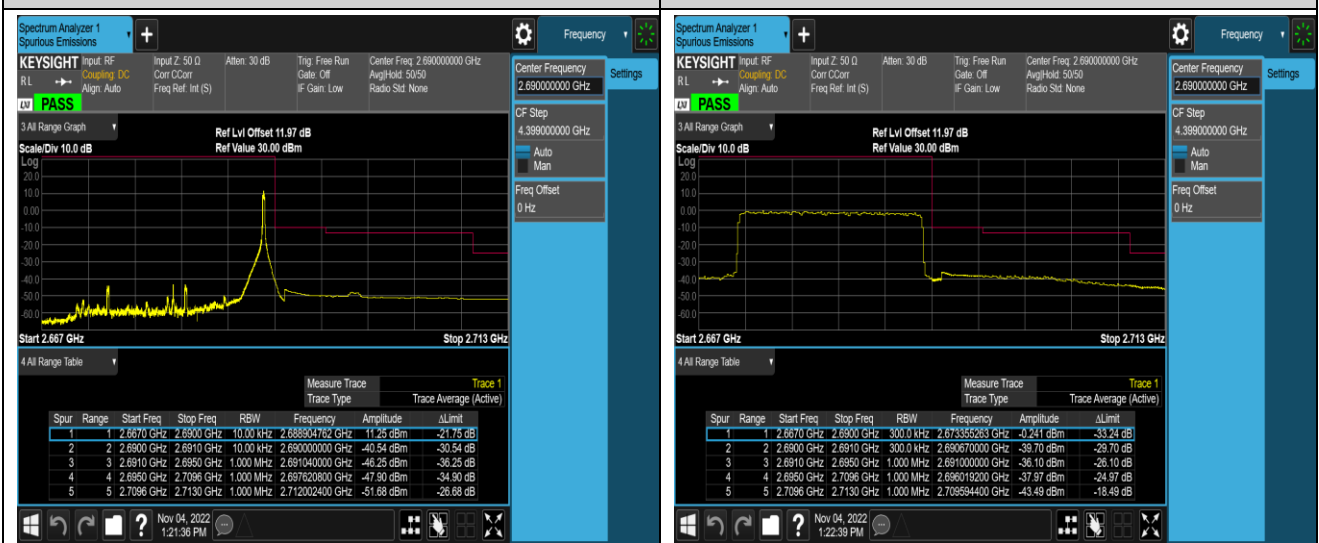
Band41-20MHz-16QAM-39750-1RB#0
