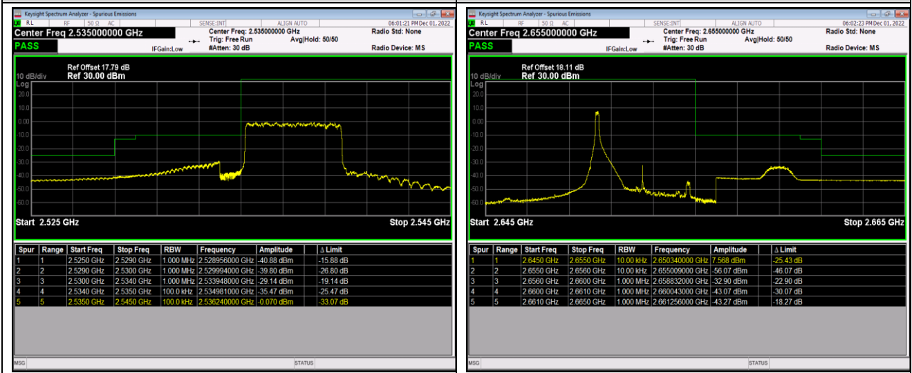
Band41-5MHz-16QAM-41215-1RB#24
