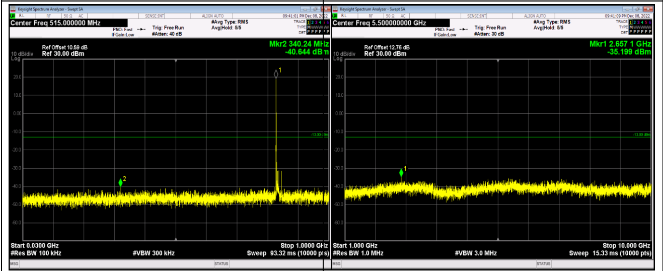
Band5-10MHz-64QAM-20525-1RB#0-Range1:30~1000MHz
