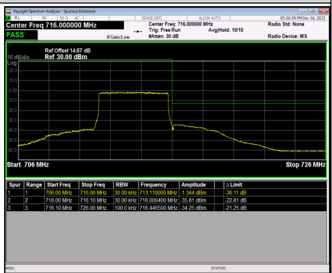
Band17-10MHz-QPSK-23780-1RB#49
