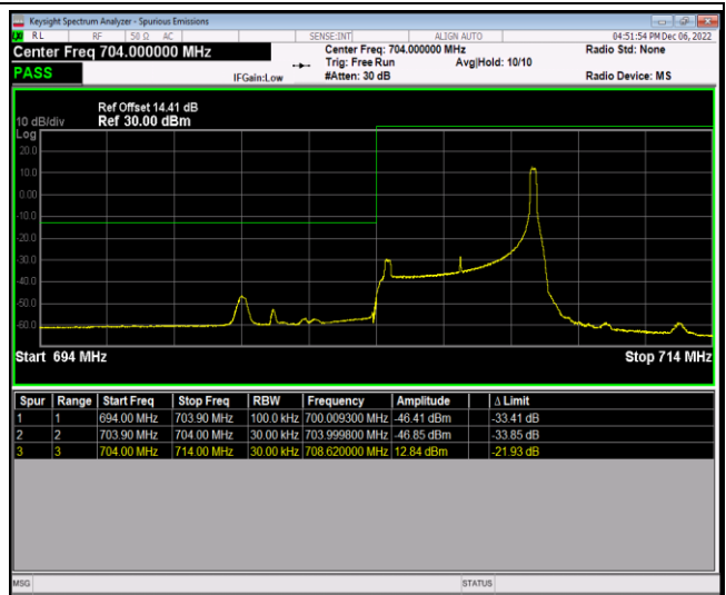
Band17-5MHz-64QAM-23825-1RB#0
