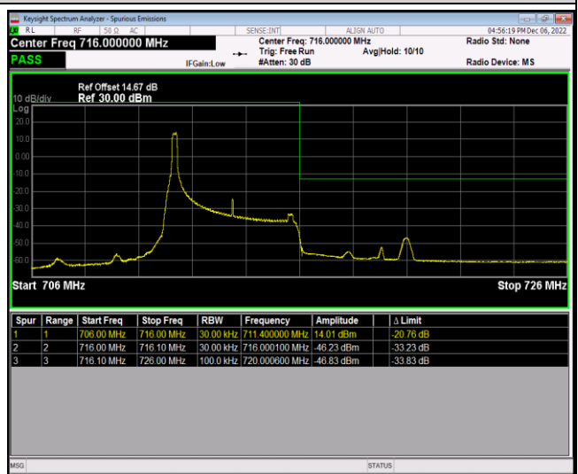
Band17-5MHz-64QAM-23825-25RB#0
