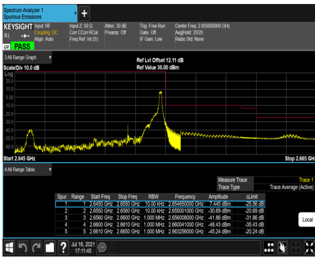
Band41-5MHz-16QAM-41215-1RB#24
