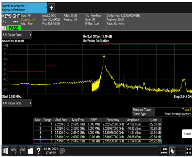
Band41-5MHz-16QAM-40065-25RB#0
