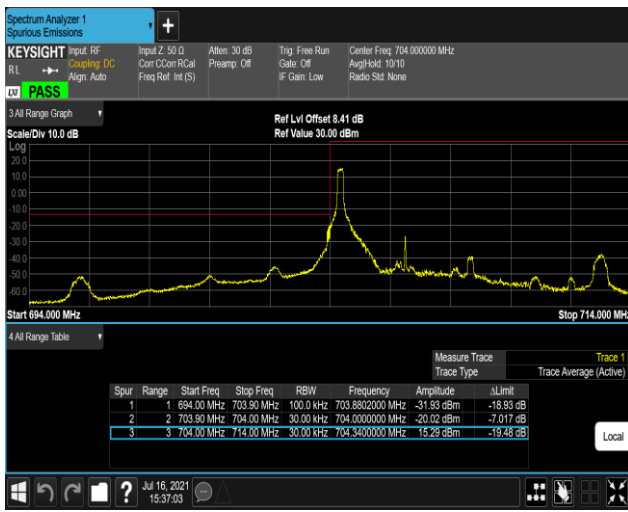
Band17-5MHz-QPSK-23755-25RB#0
