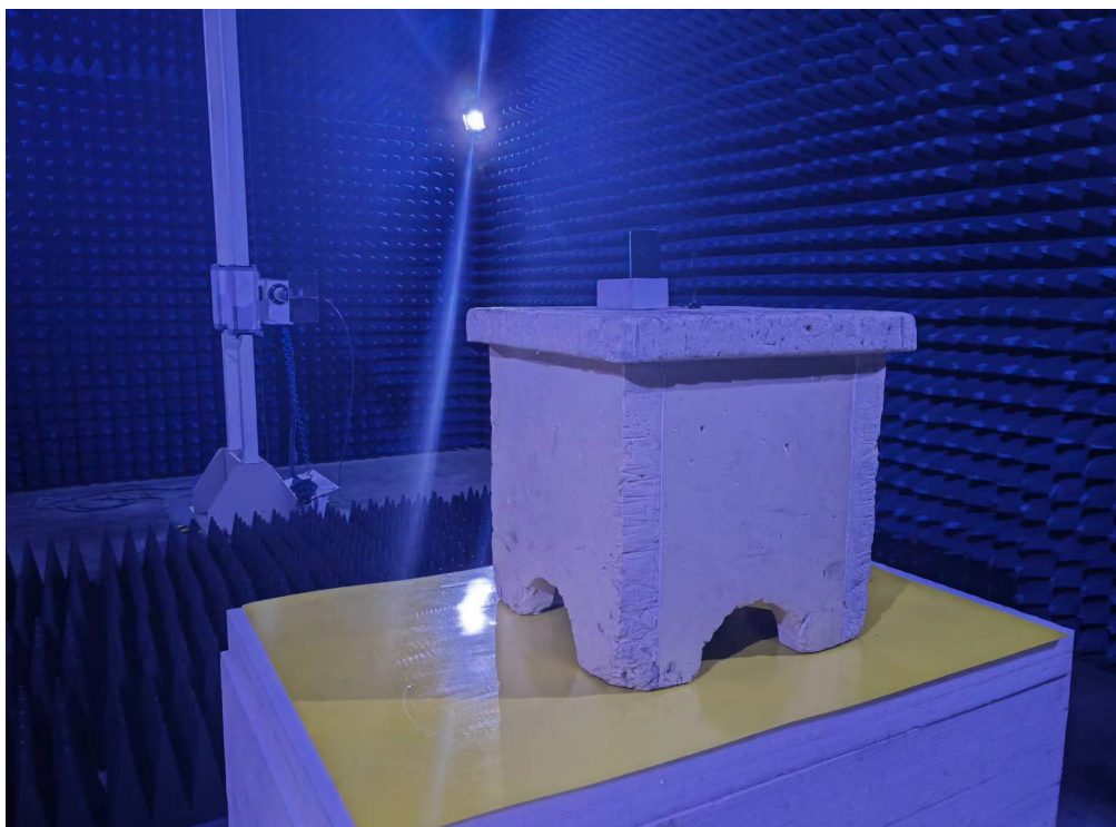
Photo of Radiated Emission Measurement (Above 1 GHz)
