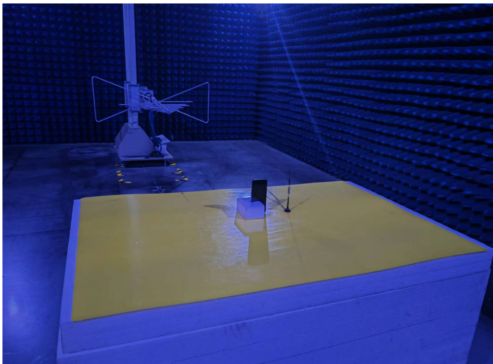
Photo of Radiated Emission Measurement (Below 1 GHz)
