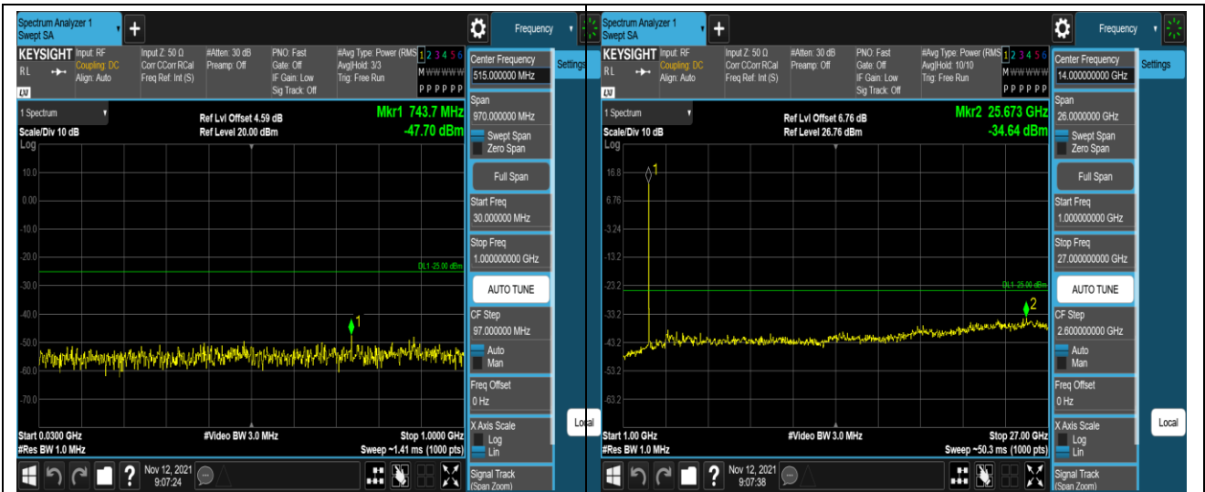
Band38-20MHz-16QAM-37850-1RB#0-Range1:30 ~1000MHz
