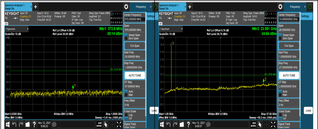
Band38-20MHz-16QAM-38000-1RB#0-Range1:30 ~1000MHz
