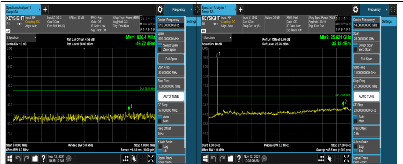
Band41-20MHz-QPSK-40640-1RB#0-Range1:30~1000MHz
