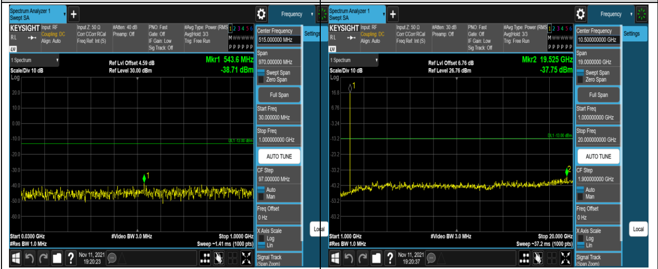
Band66-1.4MHz-QPSK-132322-1RB#0-Range1:30 ~1000MHz
