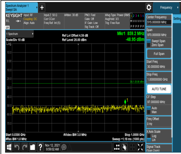
Band41-5MHz-16QAM-40065-1RB#0-Range 1:30~1000MHz
