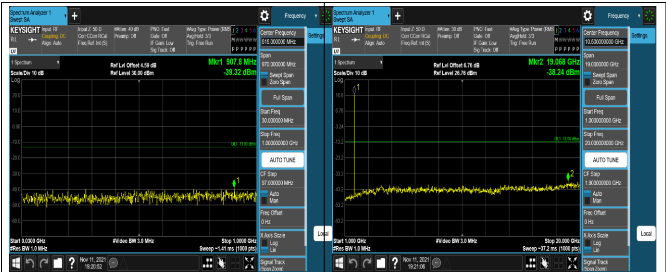
Band66-1.4MHz-16QAM-132665-1RB#0-Range1:3 0~1000MHz
