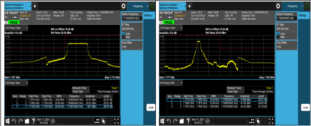
Band66-1.4MHz-QPSK-131979-6RB#0
