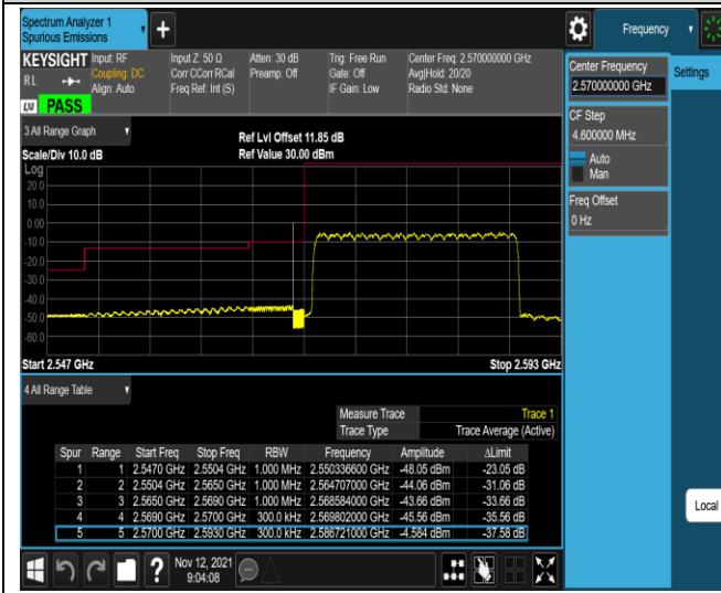
Band38-20MHz-16QAM-37850-100RB#0
