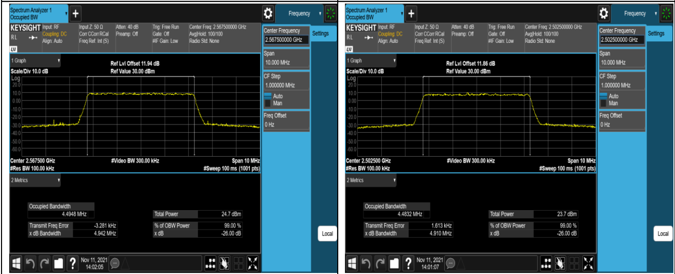
Band7-5MHz-QPSK-21425-25RB#0
