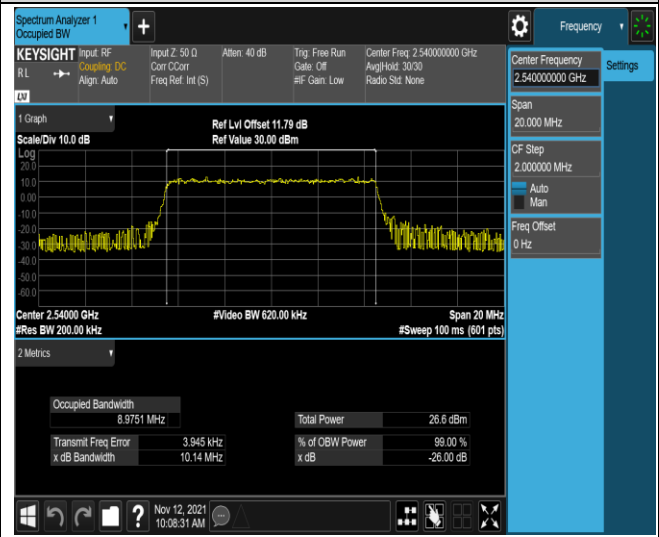
Band41-10MHz-16QAM-40090-50RB#0
