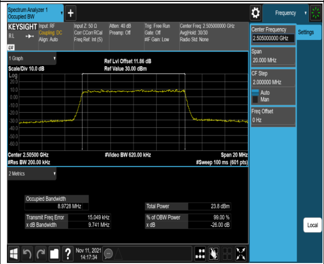
Band7-10MHz-16QAM-20800-50RB#0
