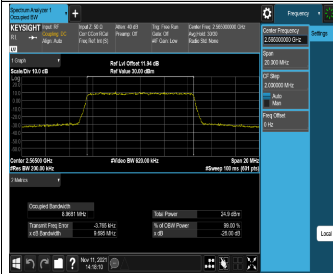
Band7-10MHz-QPSK-21400-50RB#0
