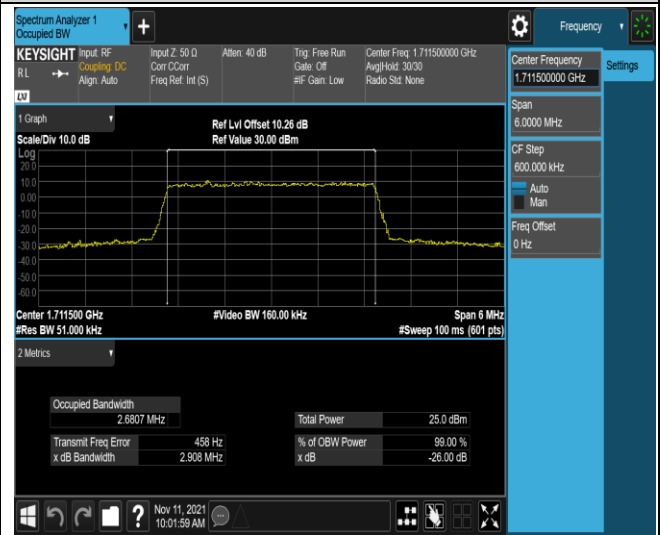
Band4-3MHz-16QAM-19965-15RB#0
