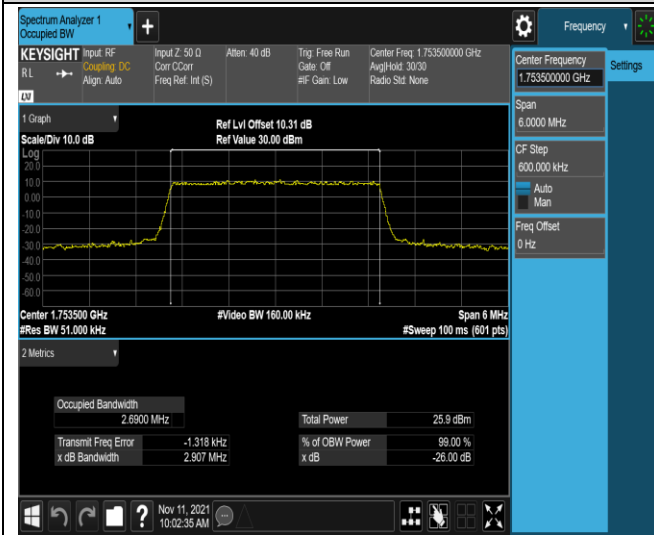
Band4-3MHz-QPSK-20385-15RB#0
