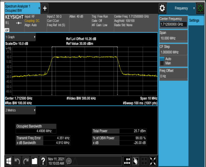
Band4-5MHz-16QAM-19975-25RB#0
