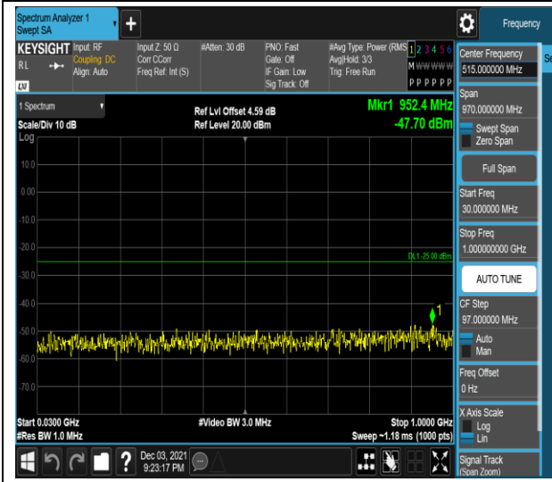
Band41-5MHz-QPSK-40640-1RB#0-Range1:30~1000MHz
