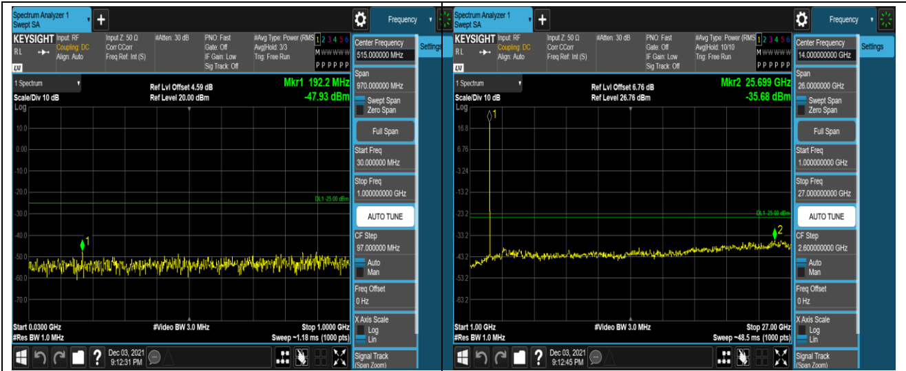
Band38-20MHz-QPSK-38000-1RB#0-Range1:30~1000MHz
