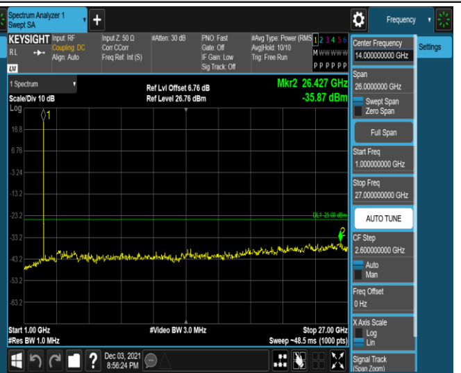
Band38-5MHz-16QAM-37775-1RB#0-Range2:1000~27000MHz
