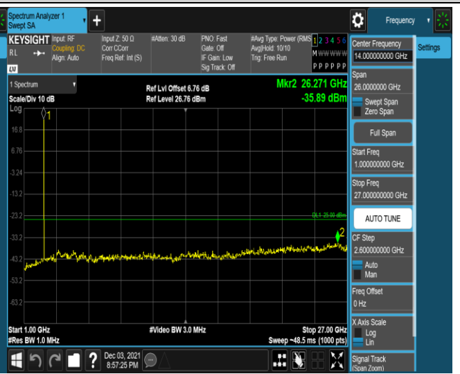
Band38-5MHz-16QAM-37775-1RB#0-Range2:1000~27000MHz
