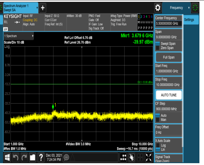
Band5-10MHz-16QAM-20450-1RB#0-Range2:1000~10000MHz
