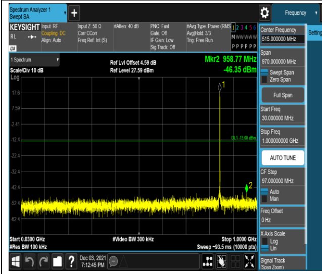
Band5-1.4MHz-16QAM-20525-1RB#0-Range1:30~1000MHz
