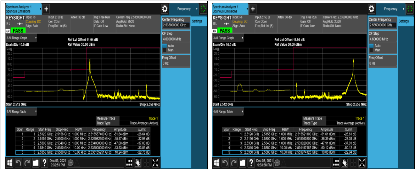
Band41-20MHz-QPSK-40140-1RB#0
