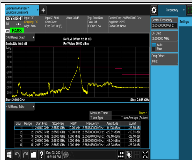
Band41-5MHz-16QAM-41215-1RB#24
