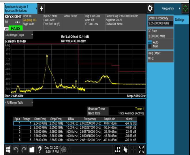
Band41-5MHz-16QAM-41215-1RB#0
