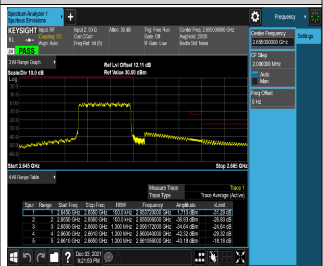
Band41-5MHz-16QAM-41215-25RB#0
