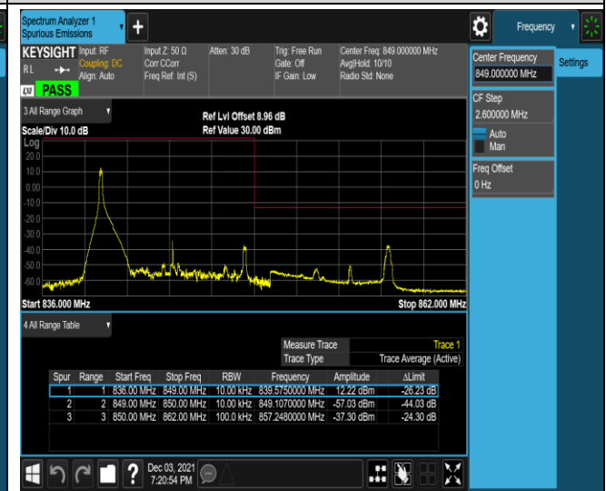
Band5-10MHz-16QAM-20600-1RB#0
