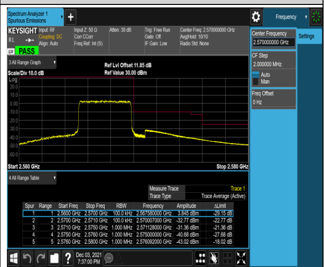
Band7-5MHz-16QAM-21425-25RB#0
