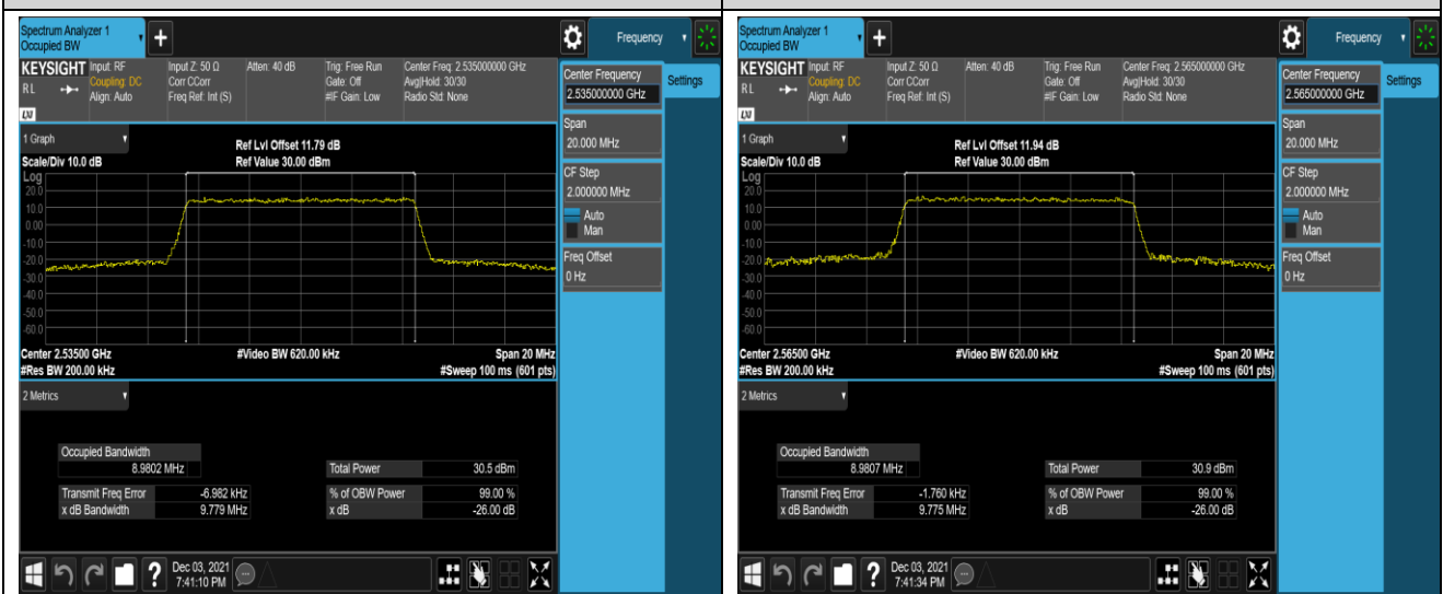
Band7-10MHz-16QAM-21100-50RB#0
