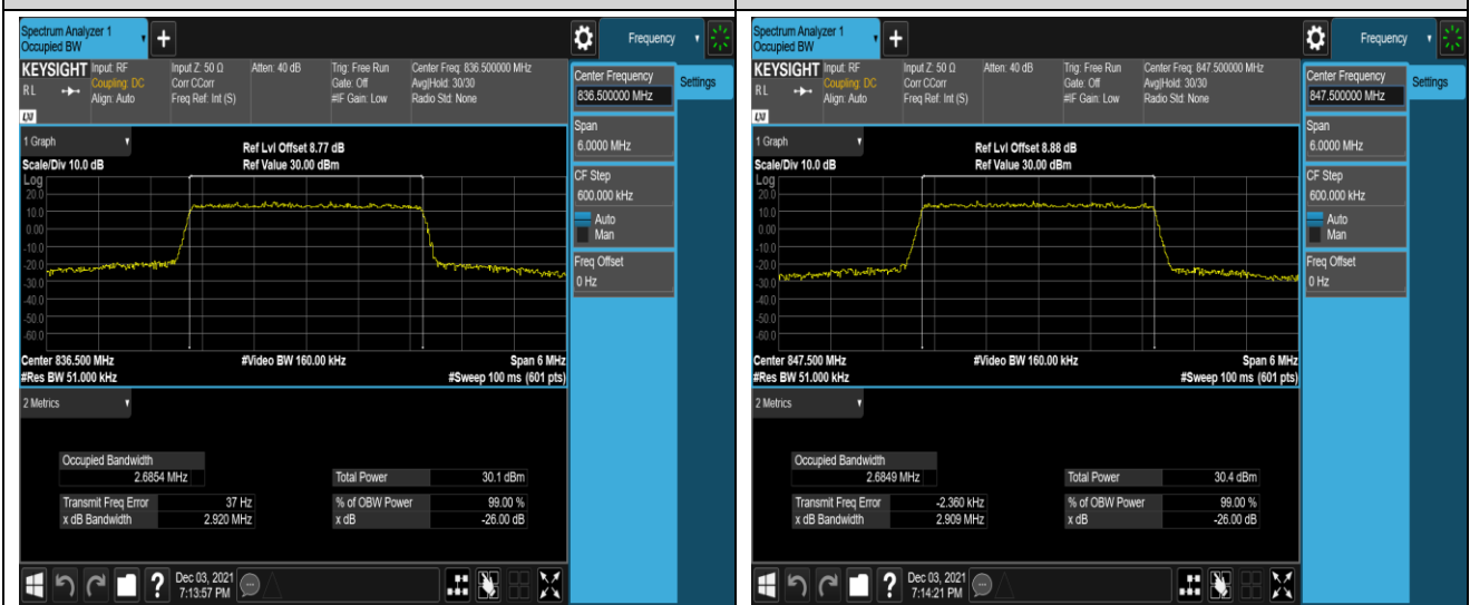
Band5-3MHz-16QAM-20525-15RB#0
