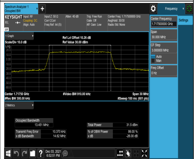
Band4-15MHz-16QAM-20025-75RB#0
