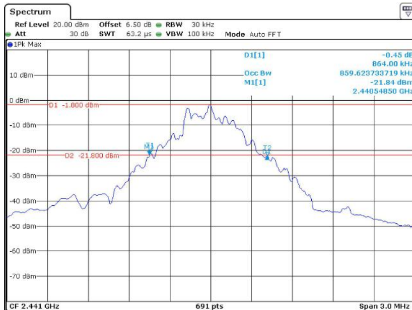
DH1_2441MHz
