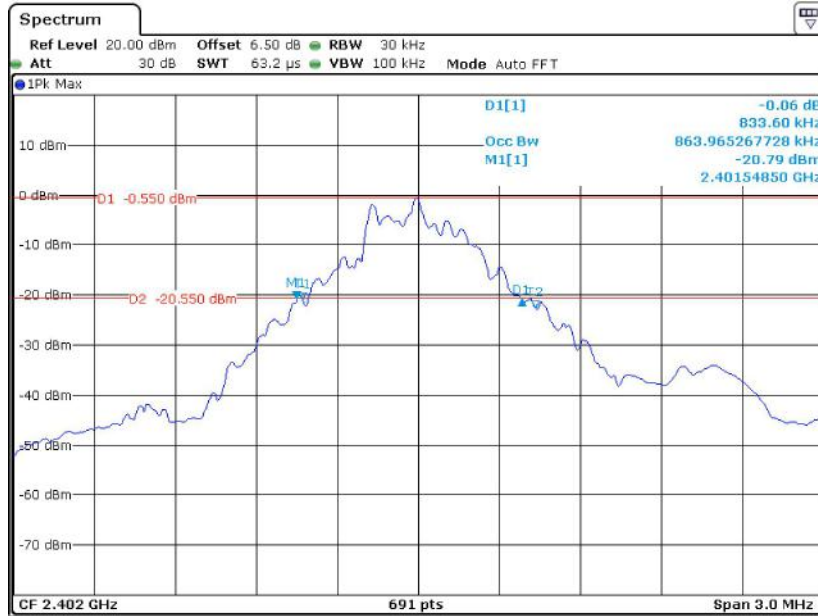
DH1_2402MHz
