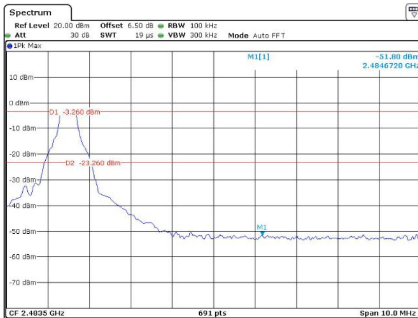
DH1_High_2480MHz
