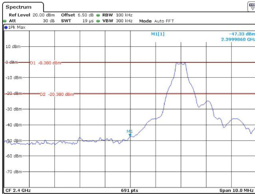
DH1_Low_2402MHz
