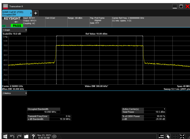
20MHz_15kHz_2560MHz_CP-OFDM 64 QAM_RB106@ 18.898 MHz
