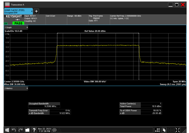
10MHz_15kHz_2505MHz_CP-OFDM 16 QAM_RB52@0 9.260 MHz
