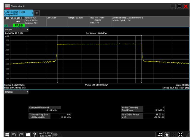
15MHz_15kHz_2507.5MHz_CP-OFDM QPSK_RB79@0 14.104 MHz
