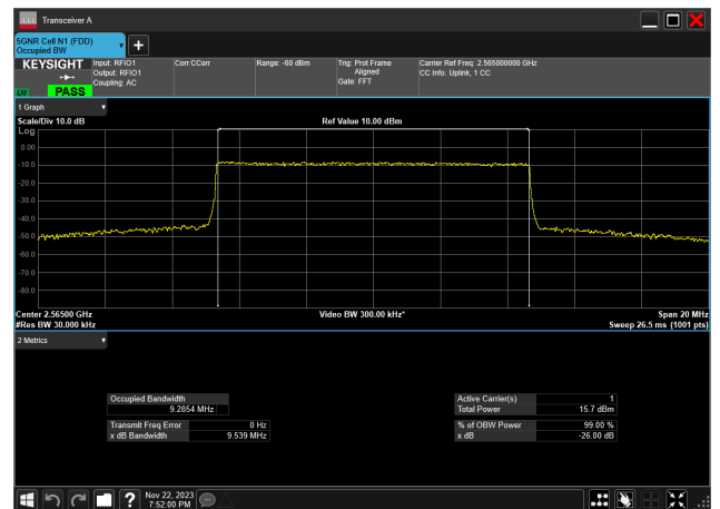
10MHz_15kHz_2565MHz_CP-OFDM 256 QAM_RB52@0 9.285 MHz
