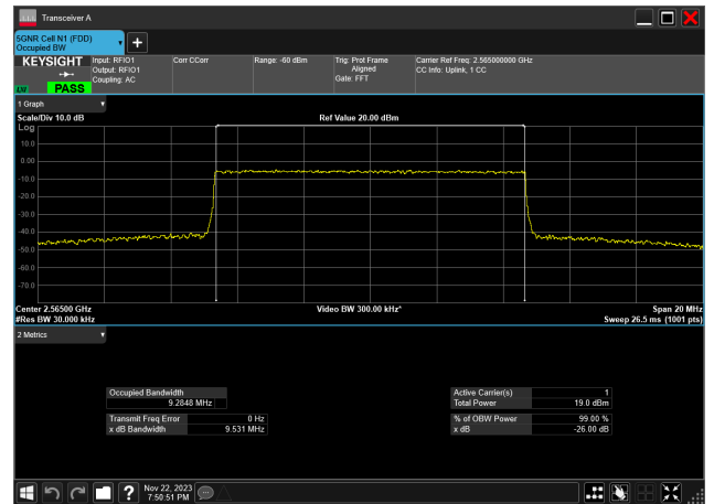
10MHz_15kHz_2565MHz_CP-OFDM 16 QAM_RB52@0 9.285 MHz
