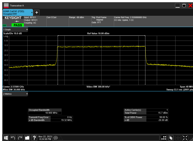
20MHz_15kHz_2535MHz_CP-OFDM 256 QAM_RB106@0 18.900 MHz
