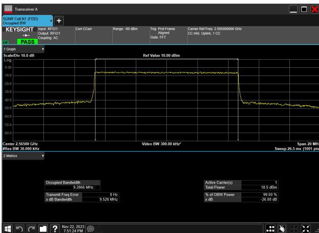
10MHz_15kHz_2565MHz_CP-OFDM 64 QAM_RB52@0 9.287 MHz
