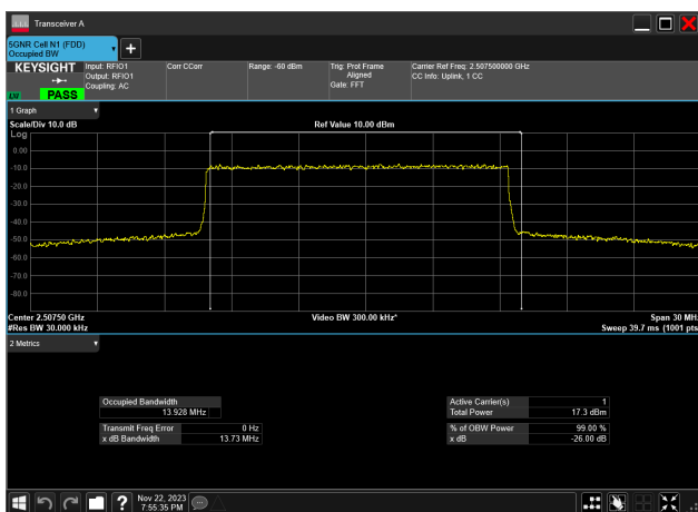
15MHz_15kHz_2507.5MHz_DFT-s-OFDM 256 QAM_RB75@0 13.928 MHz
