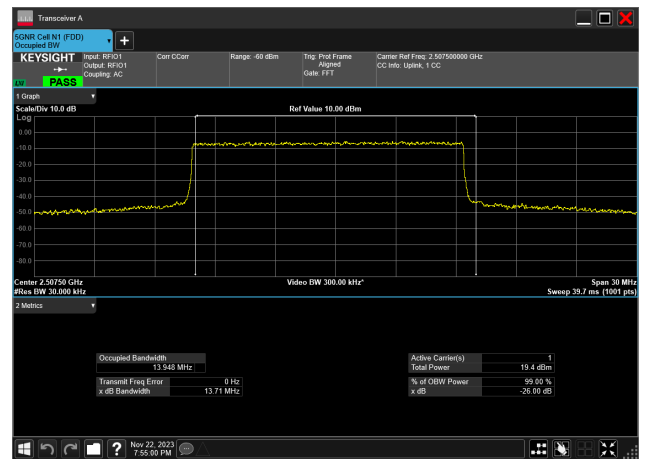
15MHz_15kHz_2507.5MHz_DFT-s-OFDM 64 QAM_RB75@0 13.948 MHz
