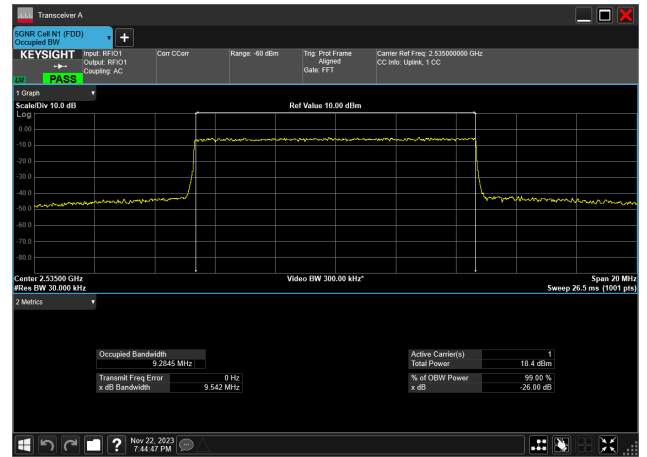
10MHz_15kHz_2535MHz_CP-OFDM 64 QAM_RB52@0 9.285 MHz
