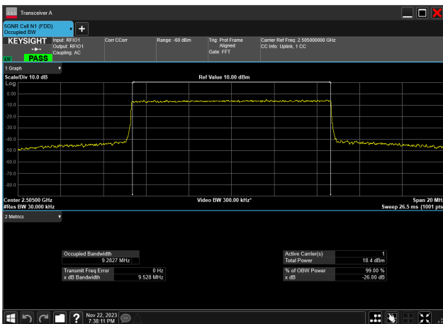
10MHz_15kHz_2505MHz_CP-OFDM 64 QAM_RB52@0 9.283 MHz
