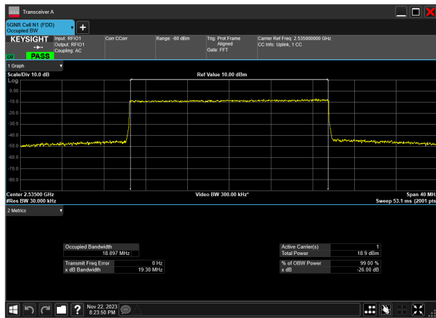
20MHz_15kHz_2535MHz_CP-OFDM 16 QAM_RB106@0 18.897 MHz
