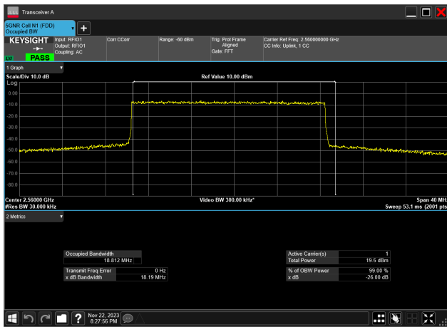
20MHz_15kHz_2560MHz_DFT-s-OFDM 64 QAM_RB100@ 18.812 MHz
