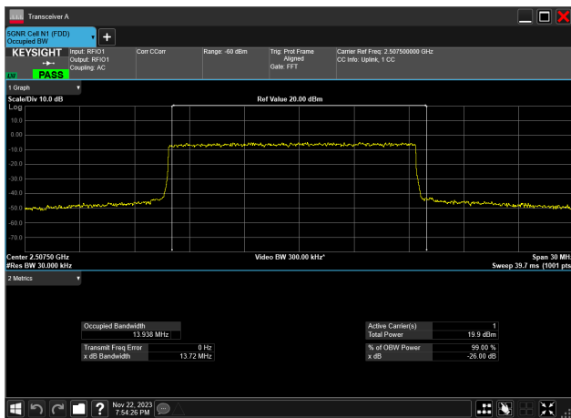
15MHz_15kHz_2507.5MHz_DFT-s-OFDM 16 QAM_RB75@0 13.938 MHz
