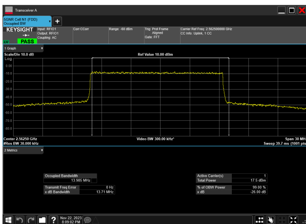
15MHz_15kHz_2562.5MHz_DFT-s-OFDM 256 QAM_RB75@0 13.985 MHz
