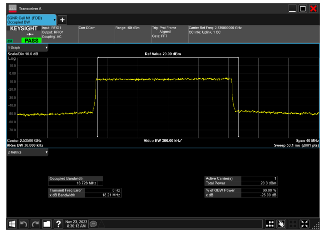
20MHz_15kHz_2535MHz_DFT-s-OFDM QPSK_RB100@0 18.728 MHz
