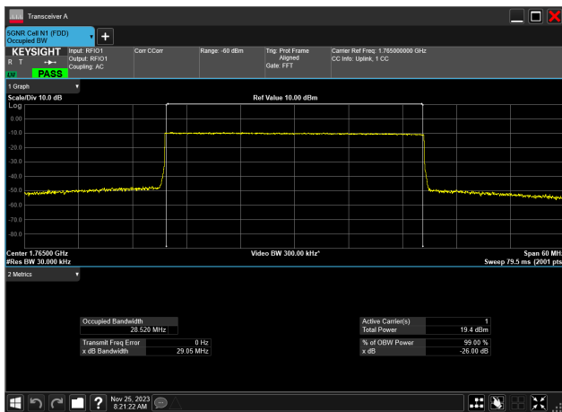
30MHz_15kHz_1765MHz_CP-OFDM QPSK_RB160@ 28.520 MHz
