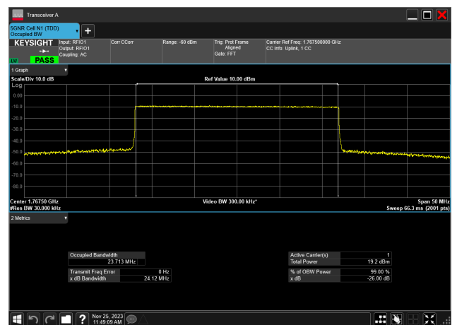
25MHz_15kHz_1767.5MHz_CP-OFDM QPSK_RB133@ 23.713 MHz
