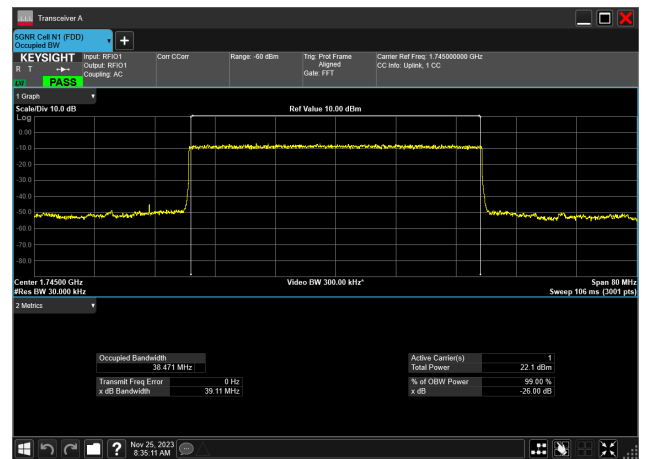
40MHz_15kHz_1745MHz_DFT-s-OFDM PI/2 BPSK_RB216@0 38.471 MHz
