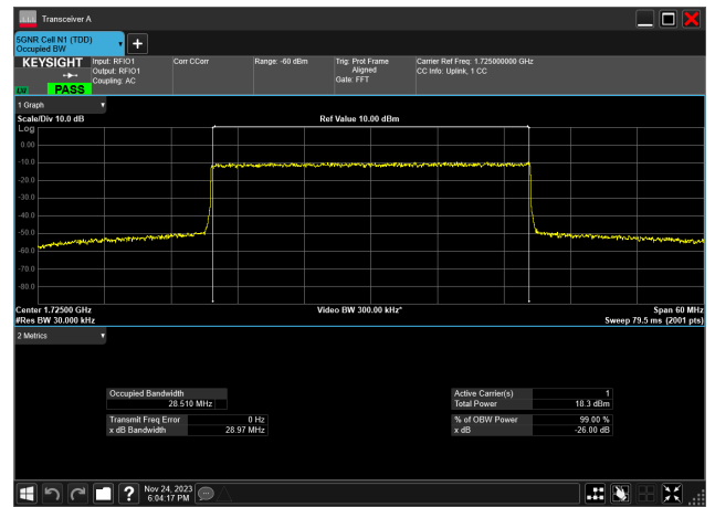
30MHz_15kHz_1725MHz_DFT-s-OFDM 256 QAM_RB160@ 28.510 MHz
