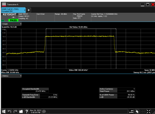
25MHz_15kHz_1722.5MHz_DFT-s-OFDM 16 QAM_RB128@ 23.470 MHz
