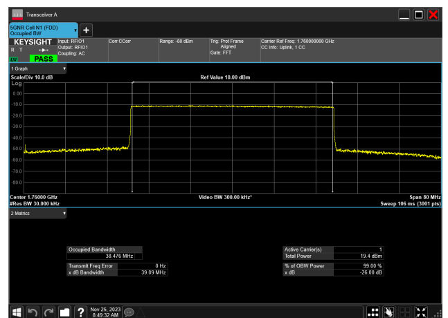
40MHz_15kHz_1760MHz_CP-OFDM QPSK_RB216@0 38.476 MHz
