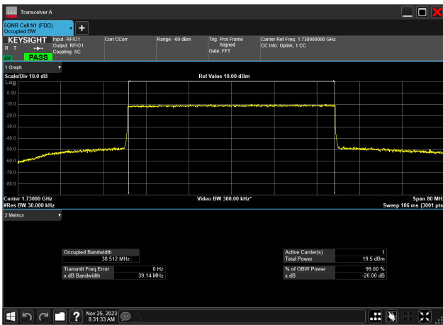
40MHz_15kHz_1730MHz_CP-OFDM 16 QAM_RB216@0 38.512 MHz
