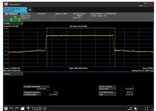
25MHz_15kHz_1722.5MHz_DFT-s-OFDM 64 QAM_RB128@ 23.456 MHz
