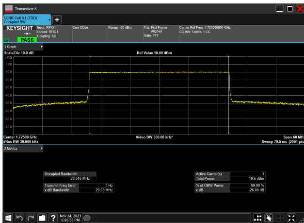
30MHz_15kHz_1725MHz_CP-OFDM QPSK_RB160@ 28.516 MHz
