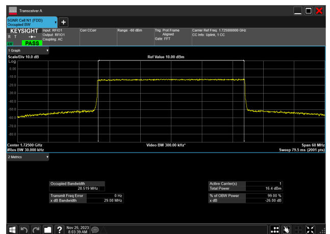
30MHz_15kHz_1725MHz_CP-OFDM 256 QAM_RB160@ 28.519 MHz
