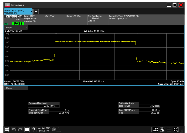
25MHz_15kHz_1767.5MHz_DFT-s-OFDM QPSK_RB128@ 23.524 MHz
