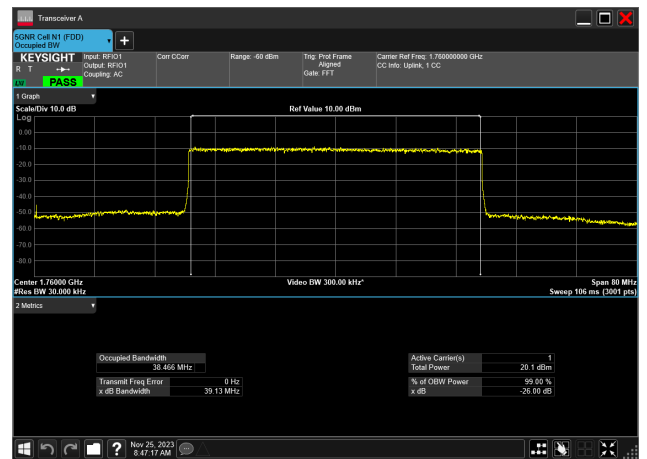
40MHz_15kHz_1760MHz_DFT-s-OFDM 64 QAM_RB216@0 38.466 MHz
