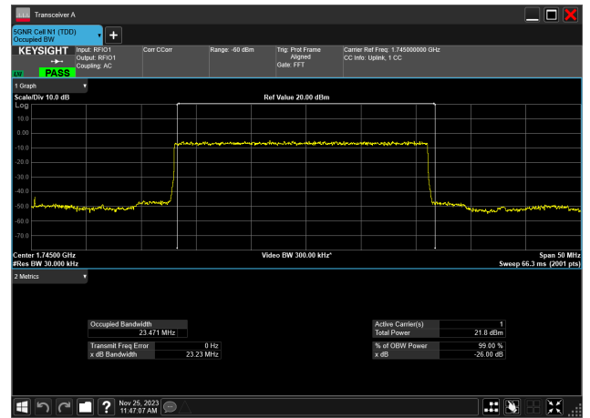
25MHz_15kHz_1745MHz_DFT-s-OFDM PI/2 BPSK_RB128@0 23.471 MHz
