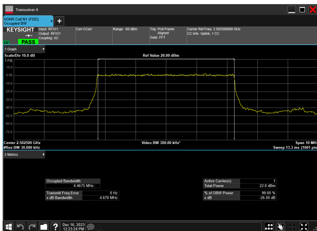
5MHz_15kHz_2502.5MHz_DFT-s-OFDM PI/2 BPSK_RB25@ 4.467 MHz
