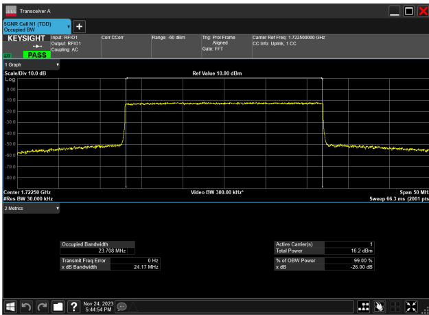
25MHz_15kHz_1722.5MHz_CP-OFDM 256 QAM_RB133@0 23.708 MHz
