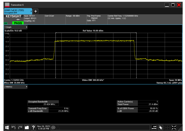
25MHz_15kHz_1722.5MHz_DFT-s-OFDM QPSK_RB128@ 23.424 MHz
