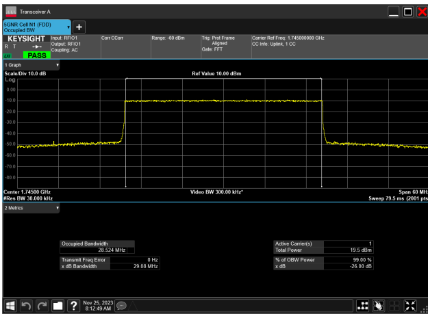
30MHz_15kHz_1745MHz_CP-OFDM 16 QAM_RB160@0 28.524 MHz
