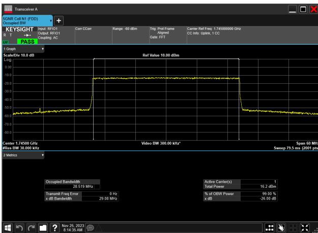
30MHz_15kHz_1745MHz_CP-OFDM 256 QAM_RB160@0 28.519 MHz
