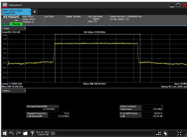
25MHz_15kHz_1745MHz_DFT-s-OFDM 64 QAM_RB128@ 23.550 MHz
