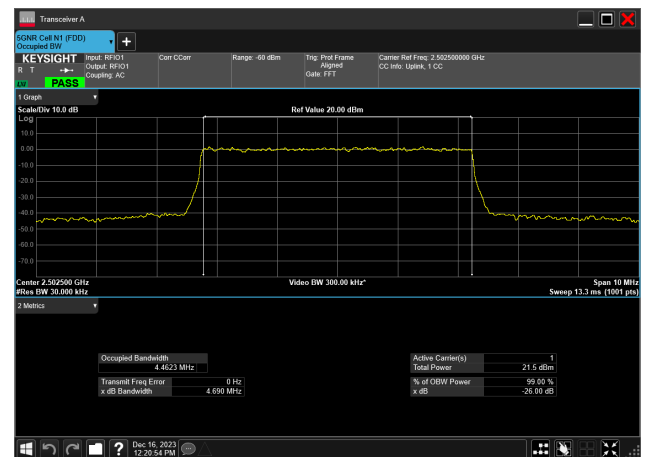
5MHz_15kHz_2502.5MHz_DFT-s-OFDM QPSK_RB25@ 4.462 MHz
