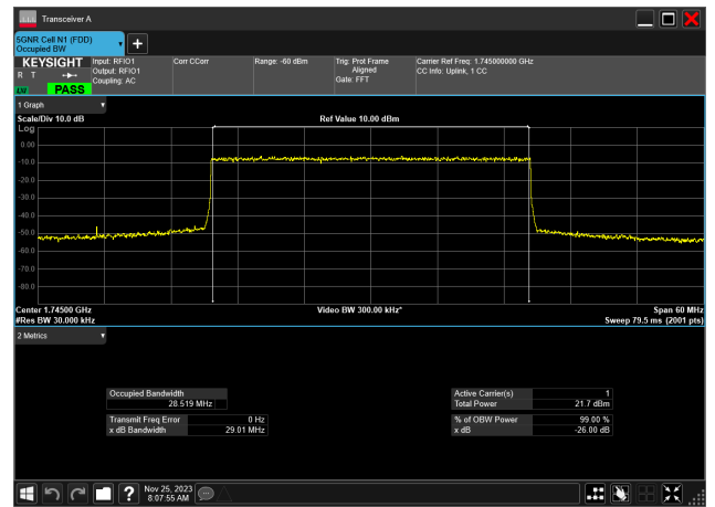
30MHz_15kHz_1745MHz_DFT-s-OFDM QPSK_RB160@ 28.519 MHz
