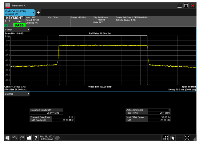
30MHz_15kHz_1745MHz_DFT-s-OFDM 64 QAM_RB160@ 28.507 MHz
