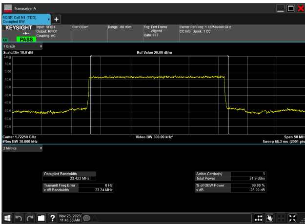
25MHz_15kHz_1722.5MHz_DFT-s-OFDM PI/2 BPSK_RB128@ 23.423 MHz
