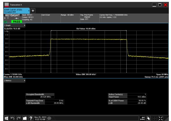
30MHz_15kHz_1765MHz_CP-OFDM 16 QAM_RB160@ 28.520 MHz
