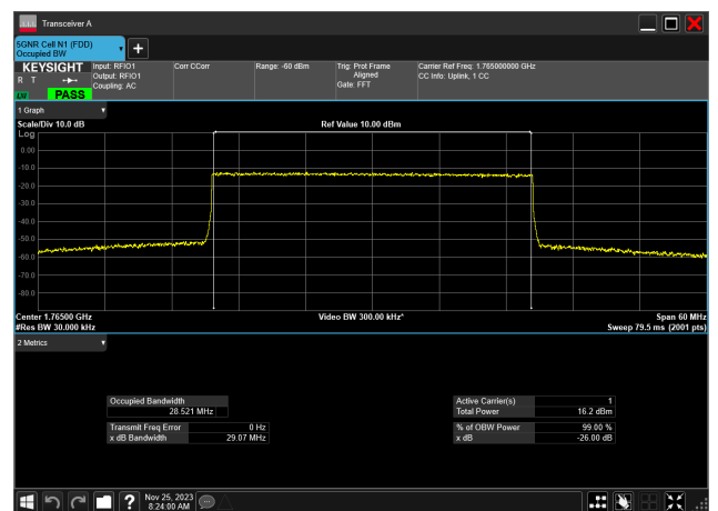
30MHz_15kHz_1765MHz_CP-OFDM 256 QAM_RB160@ 28.521 MHz
