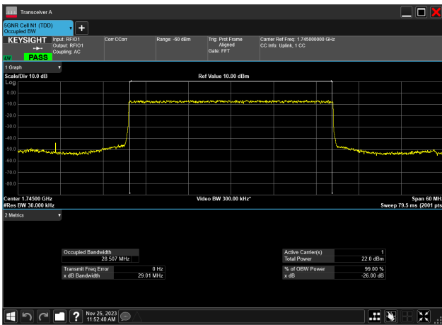
30MHz_15kHz_1745MHz_DFT-s-OFDM PI/2 BPSK_RB160@ 28.507 MHz
