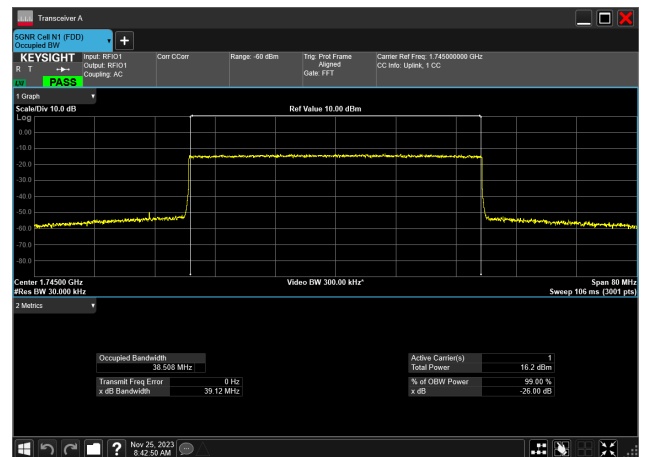
40MHz_15kHz_1745MHz_CP-OFDM 256 QAM_RB216@ 38.508 MHz
