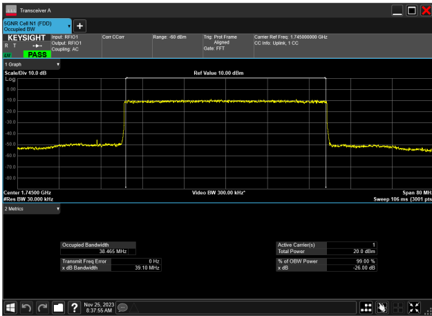
40MHz_15kHz_1745MHz_DFT-s-OFDM 64 QAM_RB216@ 38.465 MHz
