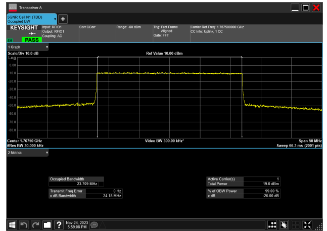
25MHz_15kHz_1767.5MHz_CP-OFDM 64 QAM_RB133@ 23.709 MHz
