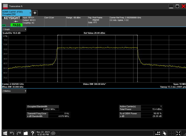
5MHz_15kHz_2502.5MHz_CP-OFDM 256 QAM_RB25@0 4.465 MHz
