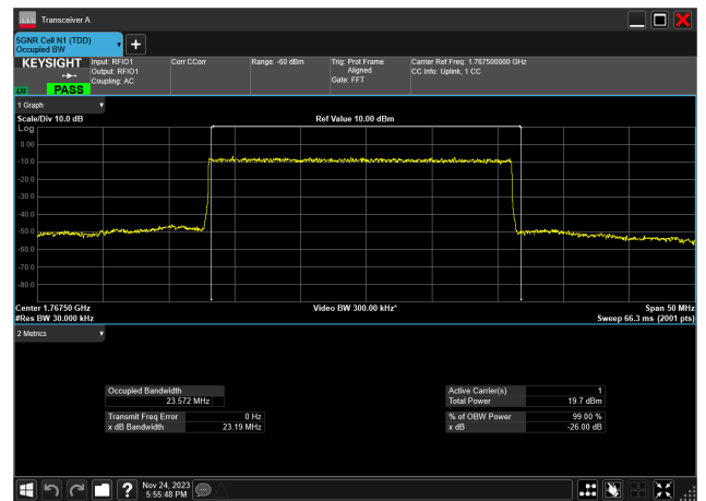
25MHz_15kHz_1767.5MHz_DFT-s-OFDM 64 QAM_RB128@ 23.572 MHz
