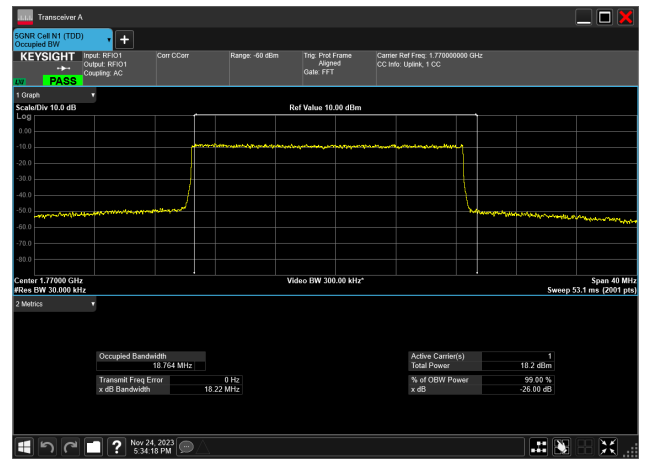
20MHz_15kHz_1770MHz_DFT-s-OFDM 256 QAM_RB100@ 18.764 MHz
