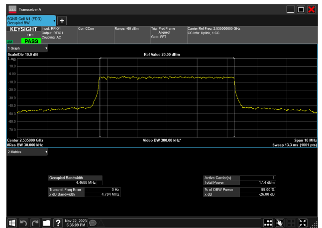
5MHz_15kHz_2535MHz_DFT-s-OFDM 256 QAM_RB25@0 4.469 MHz
