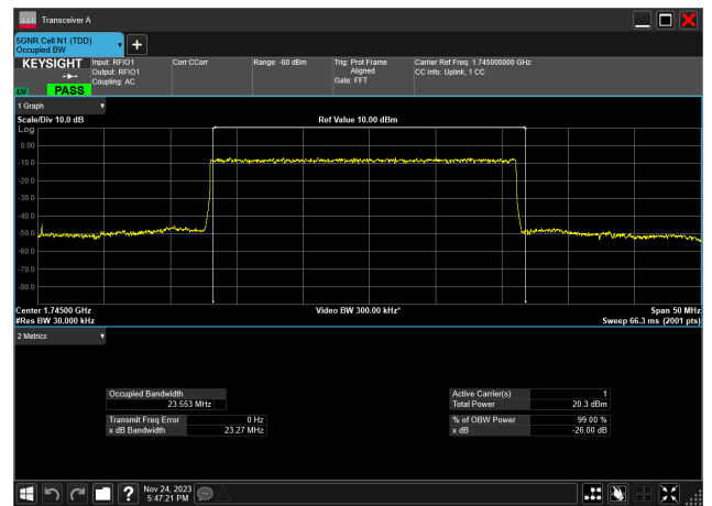
25MHz_15kHz_1745MHz_DFT-s-OFDM 16 QAM_RB128@0 23.553 MHz
