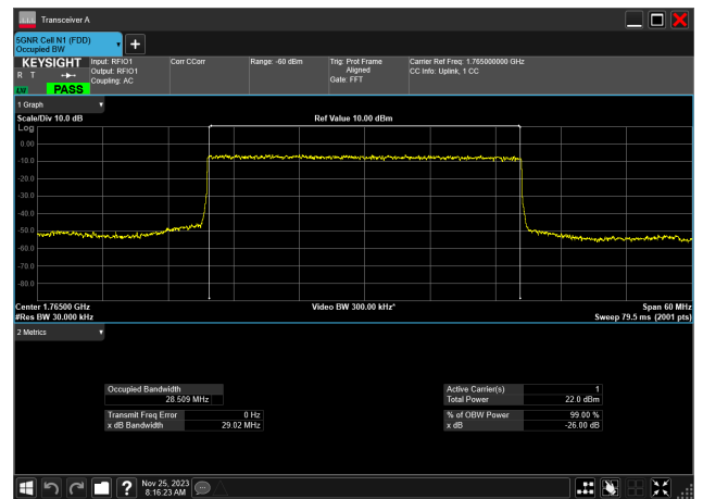
30MHz_15kHz_1765MHz_DFT-s-OFDM PI/2 BPSK_RB160@0 28.509 MHz
