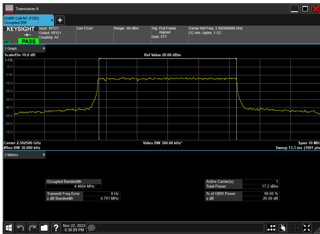
5MHz_15kHz_2502.5MHz_DFT-s-OFDM 256 QAM_RB25@0 4.468 MHz
