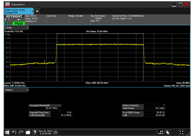
40MHz_15kHz_1745MHz_DFT-s-OFDM 256 QAM_RB216@ 38.477 MHz
