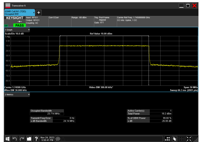
25MHz_15kHz_1745MHz_CP-OFDM 16 QAM_RB133@ 23.714 MHz
