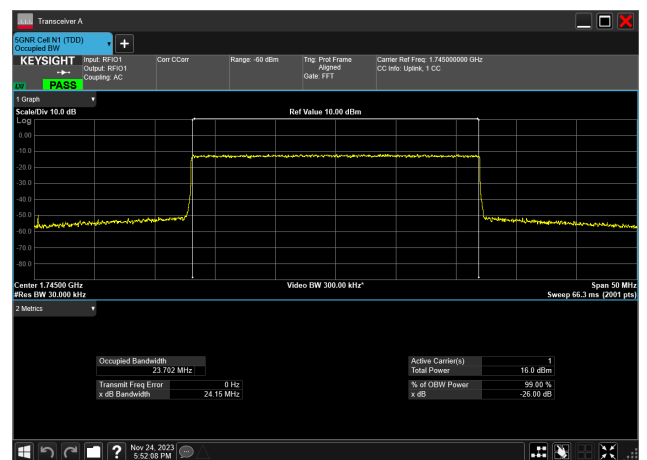
25MHz_15kHz_1745MHz_CP-OFDM 256 QAM_RB133@ 23.702 MHz
