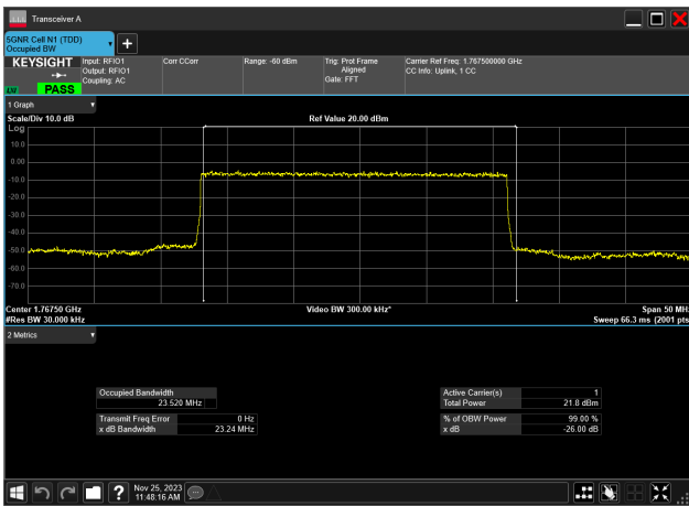
25MHz_15kHz_1767.5MHz_DFT-s-OFDM PI/2 BPSK_RB128@ 23.520 MHz
