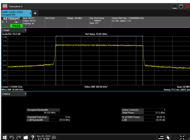
30MHz_15kHz_1765MHz_DFT-s-OFDM QPSK_RB160@0 28.520 MHz
