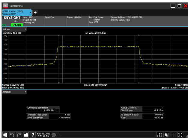
5MHz_15kHz_2502.5MHz_CP-OFDM 16 QAM_RB25@0 4.466 MHz
