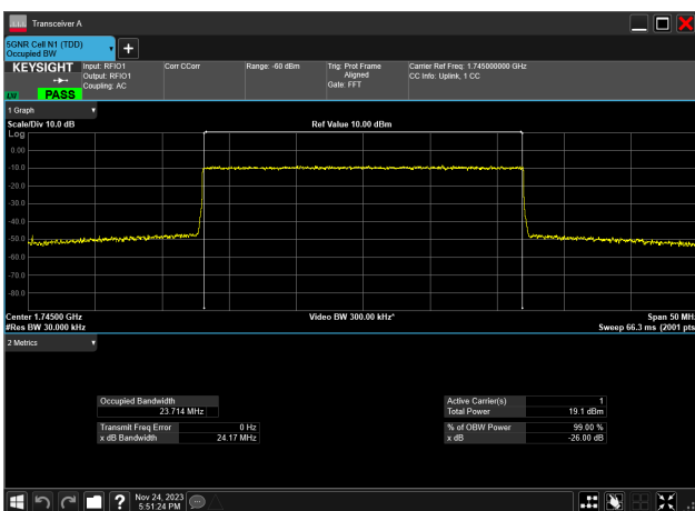
25MHz_15kHz_1745MHz_CP-OFDM 64 QAM_RB133@ 23.714 MHz
