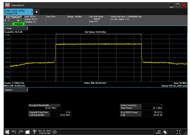
40MHz_15kHz_1730MHz_DFT-s-OFDM 64 QAM_RB216@ 38.507 MHz
