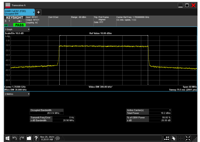
30MHz_15kHz_1765MHz_DFT-s-OFDM 256 QAM_RB160@ 28.514 MHz
