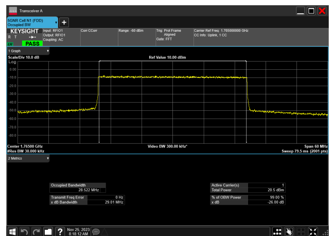
30MHz_15kHz_1765MHz_DFT-s-OFDM 16 QAM_RB160@0 28.522 MHz
