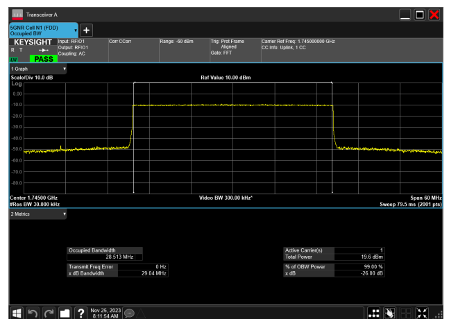
30MHz_15kHz_1745MHz_CP-OFDM QPSK_RB160@ 28.513 MHz
