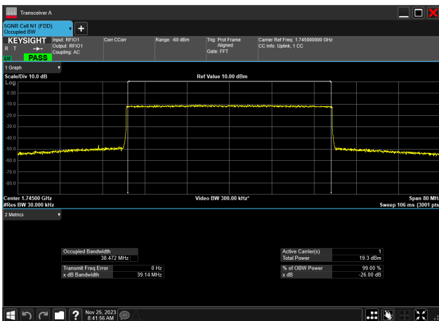
40MHz_15kHz_1745MHz_CP-OFDM 64 QAM_RB216@ 38.472 MHz
