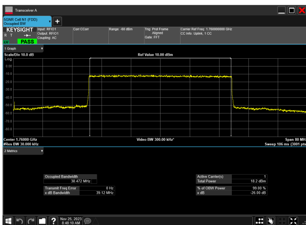
40MHz_15kHz_1760MHz_DFT-s-OFDM 256 QAM_RB216@0 38.472 MHz
