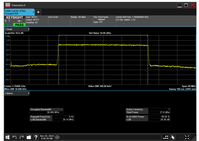
40MHz_15kHz_1760MHz_DFT-s-OFDM QPSK_RB216@0 38.466 MHz
