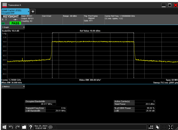
30MHz_15kHz_1745MHz_DFT-s-OFDM 16 QAM_RB160@ 28.517 MHz
