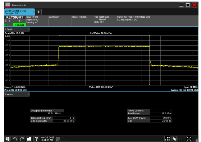
40MHz_15kHz_1745MHz_CP-OFDM 16 QAM_RB216@ 38.511 MHz
