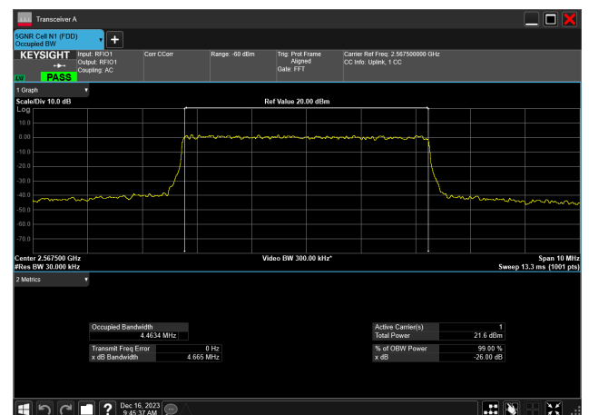
5MHz_15kHz_2567.5MHz_DFT-s-OFDM QPSK_RB25@ 4.463 MHz
