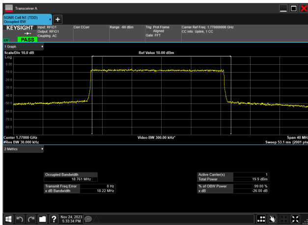
20MHz_15kHz_1770MHz_DFT-s-OFDM 64 QAM_RB100@ 18.761 MHz
