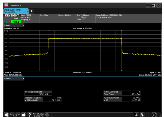
25MHz_15kHz_1722.5MHz_CP-OFDM QPSK_RB133@ 23.709 MHz
