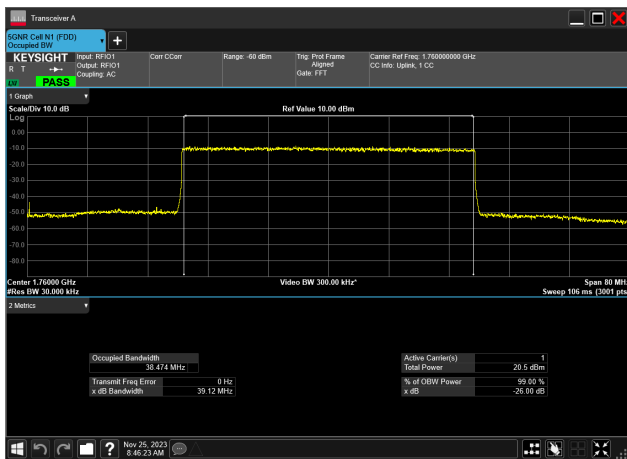
40MHz_15kHz_1760MHz_DFT-s-OFDM 16 QAM_RB216@0 38.474 MHz
