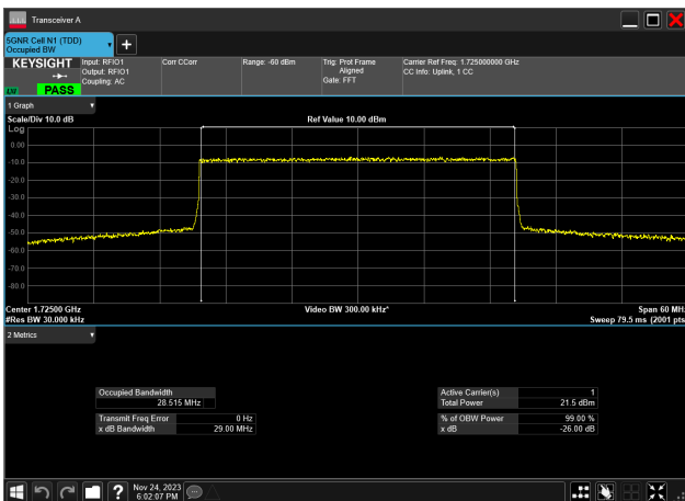
30MHz_15kHz_1725MHz_DFT-s-OFDM QPSK_RB160@ 28.515 MHz
