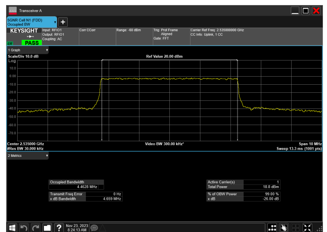
5MHz_15kHz_2535MHz_CP-OFDM 16 QAM_RB25@0 4.463 MHz
