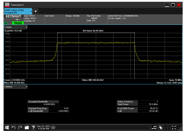
5MHz_15kHz_2535MHz_DFT-s-OFDM 16 QAM_RB25@0 4.465 MHz
