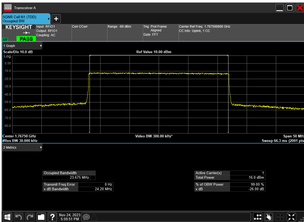
25MHz_15kHz_1767.5MHz_CP-OFDM 256 QAM_RB133@ 23.675 MHz
