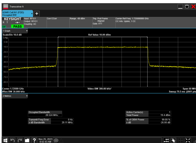
30MHz_15kHz_1725MHz_CP-OFDM 64 QAM_RB160@ 28.524 MHz
