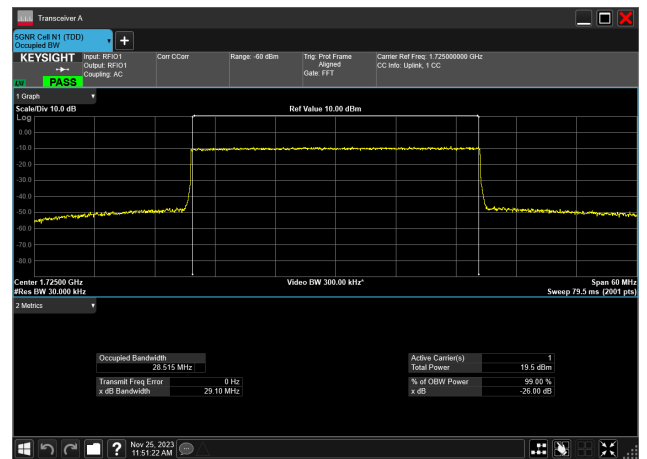
30MHz_15kHz_1725MHz_CP-OFDM 16 QAM_RB160@ 28.515 MHz
