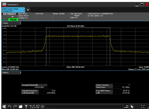
5MHz_15kHz_2535MHz_DFT-s-OFDM 64 QAM_RB25@0 4.461 MHz
