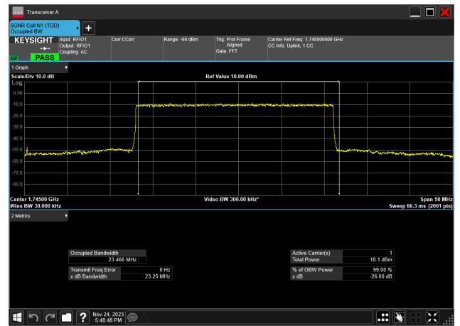
25MHz_15kHz_1745MHz_DFT-s-OFDM 256 QAM_RB128@ 23.466 MHz
