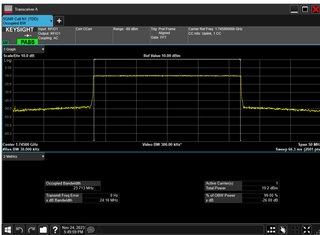
25MHz_15kHz_1745MHz_CP-OFDM QPSK_RB133@ 23.713 MHz
