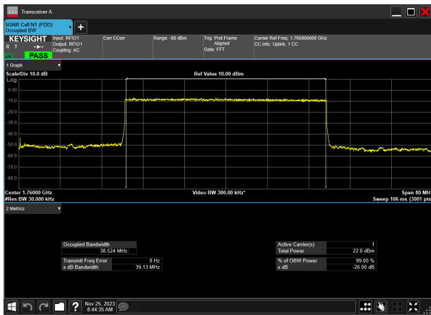
40MHz_15kHz_1760MHz_DFT-s-OFDM PI/2 BPSK_RB216@0 38.524 MHz
