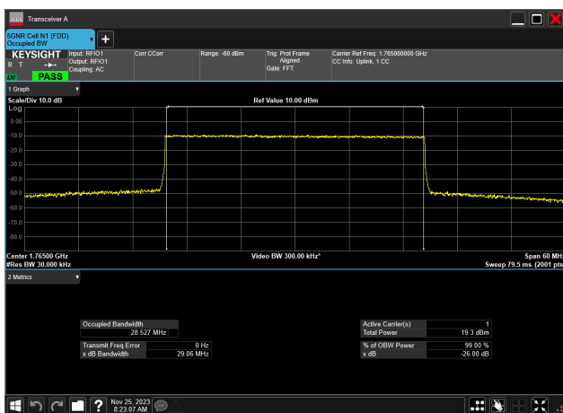
30MHz_15kHz_1765MHz_CP-OFDM 64 QAM_RB160@ 28.527 MHz
