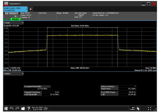
25MHz_15kHz_1722.5MHz_CP-OFDM 64 QAM_RB133@0 23.705 MHz
