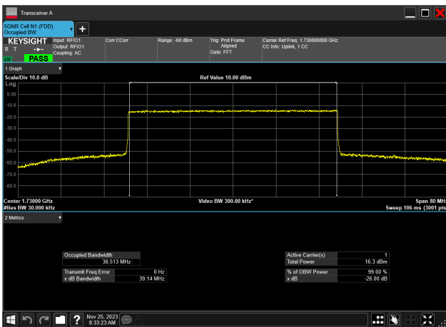
40MHz_15kHz_1730MHz_CP-OFDM 256 QAM_RB216@0 38.513 MHz
