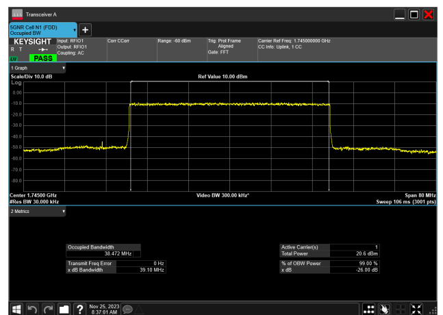
40MHz_15kHz_1745MHz_DFT-s-OFDM 16 QAM_RB216@0 38.472 MHz
