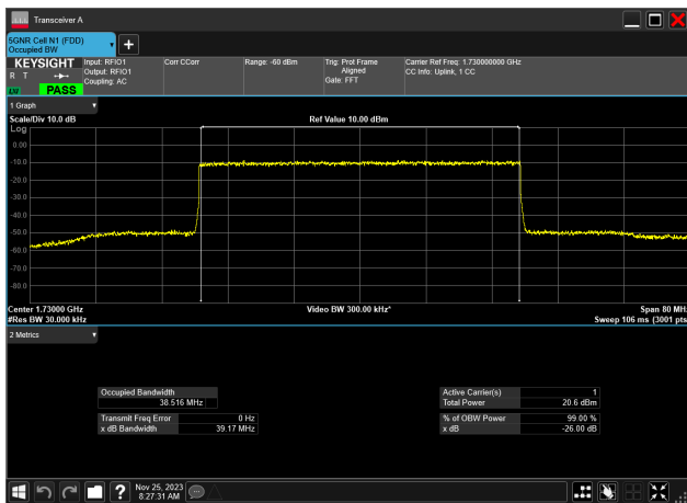
40MHz_15kHz_1730MHz_DFT-s-OFDM 16 QAM_RB216@ 38.516 MHz
