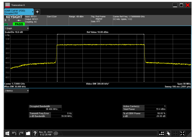
40MHz_15kHz_1730MHz_CP-OFDM 64 QAM_RB216@0 38.466 MHz
