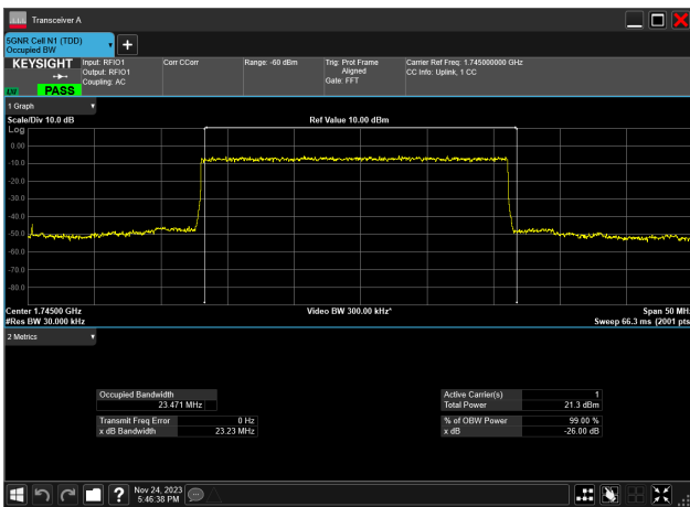
25MHz_15kHz_1745MHz_DFT-s-OFDM QPSK_RB128@0 23.471 MHz
