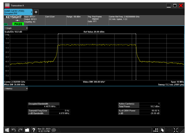
5MHz_15kHz_2502.5MHz_CP-OFDM 64 QAM_RB25@0 4.467 MHz
