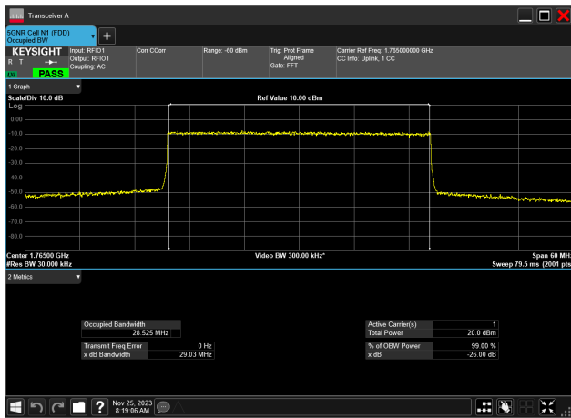
30MHz_15kHz_1765MHz_DFT-s-OFDM 64 QAM_RB160@ 28.525 MHz
