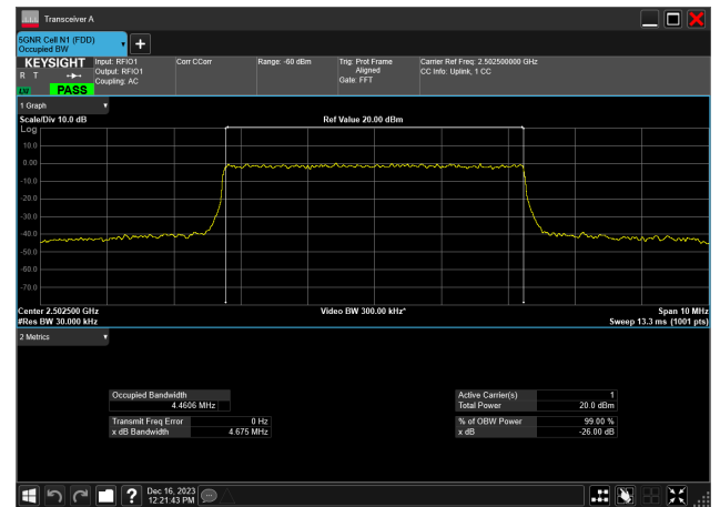
5MHz_15kHz_2502.5MHz_DFT-s-OFDM 64 QAM_RB25@ 4.461 MHz
