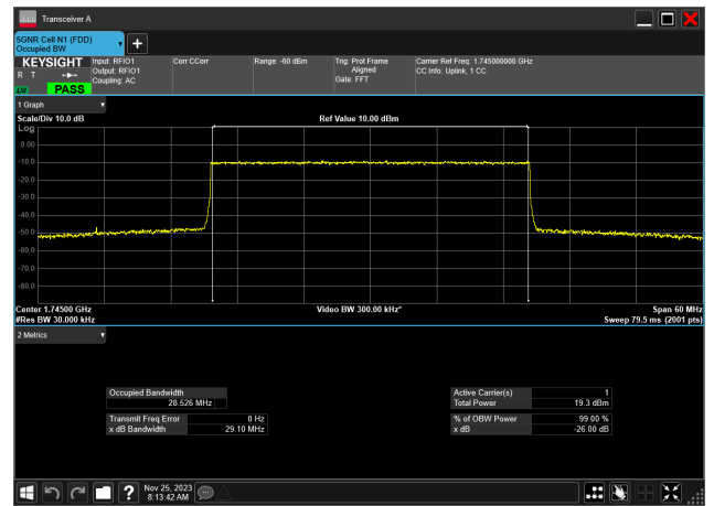
30MHz_15kHz_1745MHz_CP-OFDM 64 QAM_RB160@0 28.526 MHz
