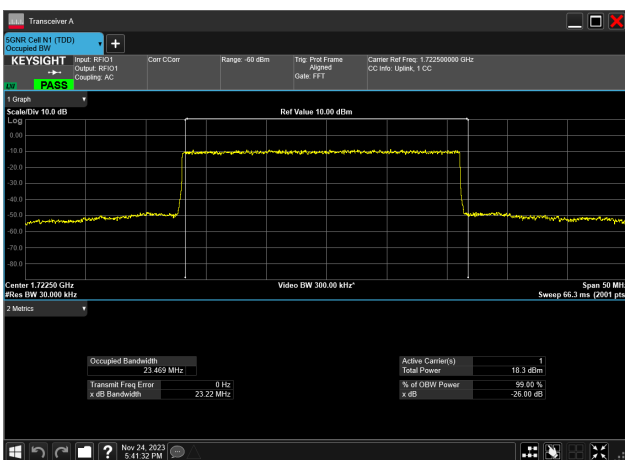
25MHz_15kHz_1722.5MHz_DFT-s-OFDM 256 QAM_RB128@ 23.469 MHz
