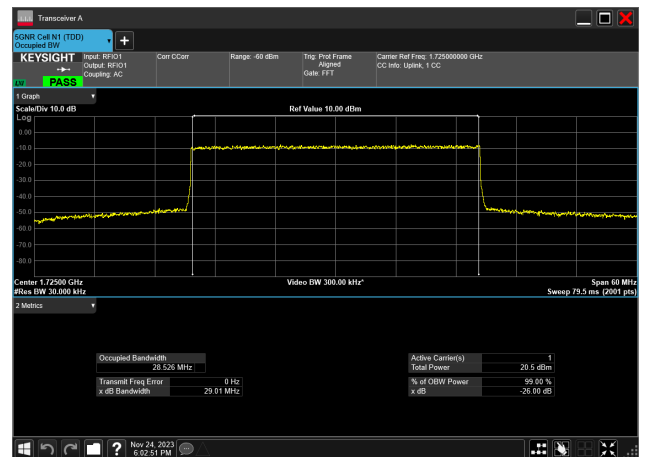
30MHz_15kHz_1725MHz_DFT-s-OFDM 16 QAM_RB160@ 28.526 MHz
