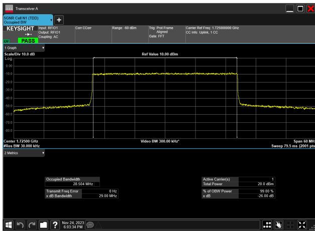
30MHz_15kHz_1725MHz_DFT-s-OFDM 64 QAM_RB160@ 28.504 MHz
