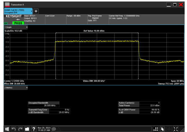
30MHz_15kHz_1725MHz_DFT-s-OFDM PI/2 BPSK_RB160@ 28.509 MHz
