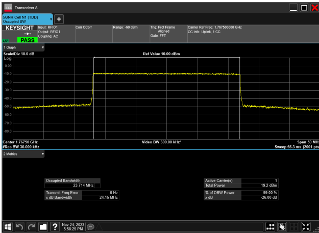
25MHz_15kHz_1767.5MHz_CP-OFDM 16 QAM_RB133@ 23.714 MHz
