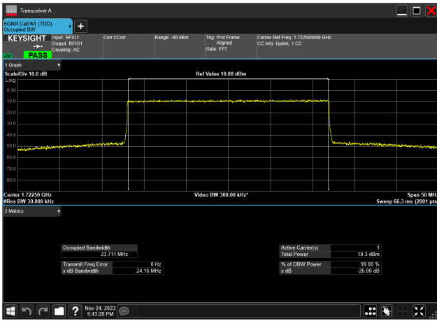
25MHz_15kHz_1722.5MHz_CP-OFDM 16 QAM_RB133@0 23.711 MHz
