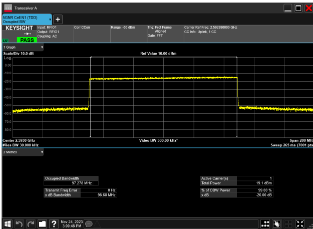
100MHz_30kHz_2592.99MHz_CP-OFDM QPSK_RB273@0 97.278 MHz
