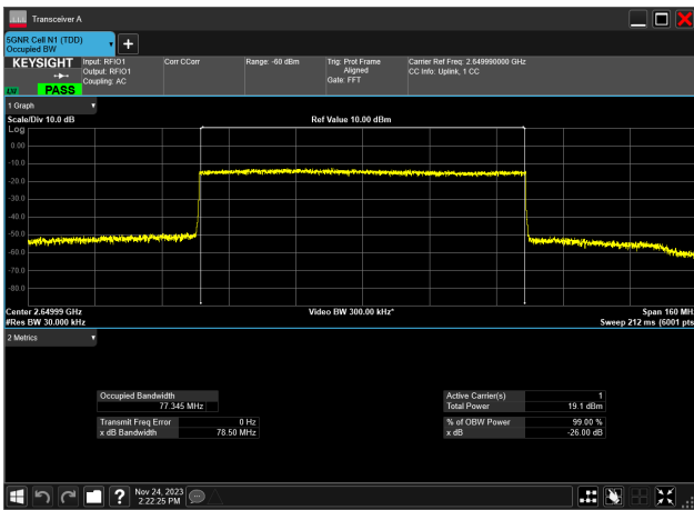
80MHz_30kHz_2649.99MHz_CP-OFDM 16 QAM_RB217@0 77.345 MHz
