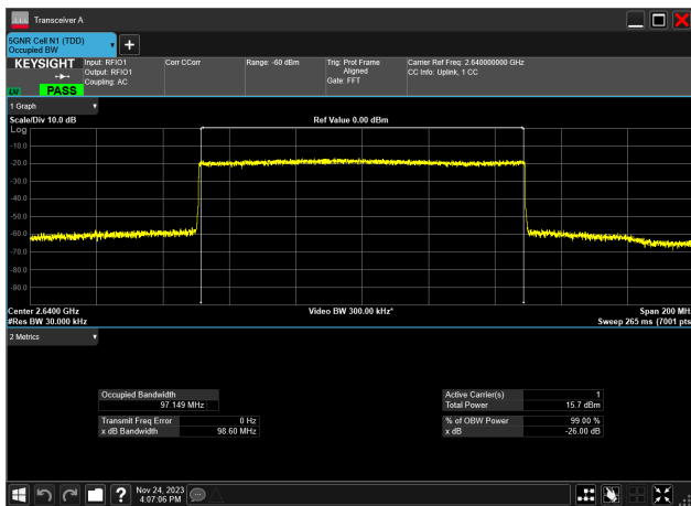
100MHz_30kHz_2640MHz_CP-OFDM 256 QAM_RB273@0 97.149 MHz
