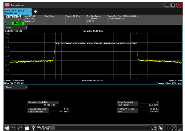
40MHz_30kHz_2670MHz_CP-OFDM 16 QAM_RB106@ 37.835 MHz
