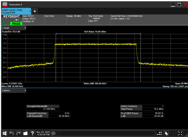
40MHz_30kHz_2516.01MHz_DFT-s-OFDM 64 QAM_RB100@0 37.349 MHz
