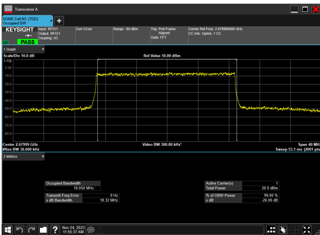
20MHz_30kHz_2679.99MHz_DFT-s-OFDM 16 QAM_RB50@ 18.050 MHz
