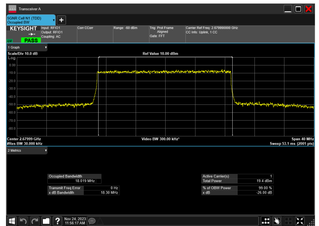
20MHz_30kHz_2679.99MHz_DFT-s-OFDM 64 QAM_RB50@ 18.019 MHz
