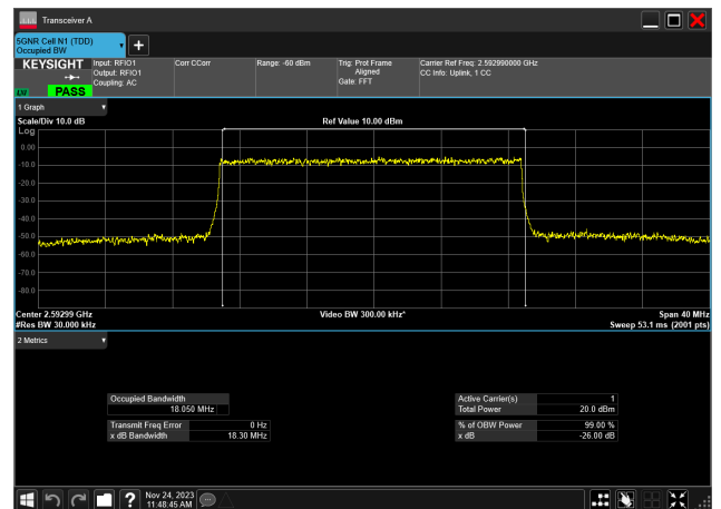
20MHz_30kHz_2592.99MHz_DFT-s-OFDM 16 QAM_RB50@0 18.050 MHz
