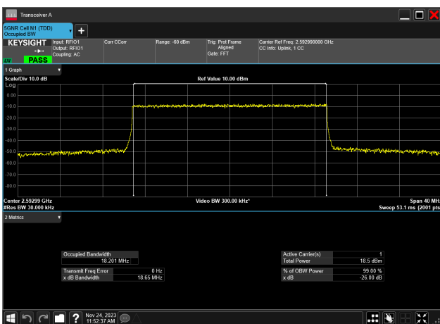
20MHz_30kHz_2592.99MHz_CP-OFDM 64 QAM_RB51@0 18.201 MHz
