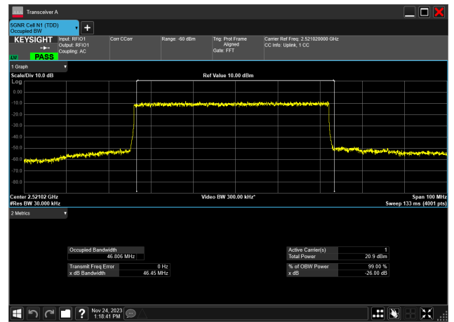
50MHz_30kHz_2521.02MHz_DFT-s-OFDM QPSK_RB128@0 46.806 MHz
