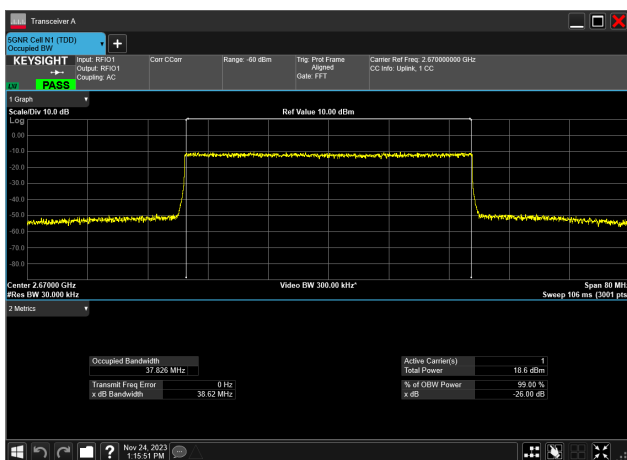
40MHz_30kHz_2670MHz_CP-OFDM 64 QAM_RB106@ 37.826 MHz
