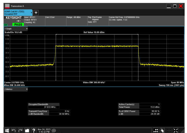
40MHz_30kHz_2670MHz_CP-OFDM 256 QAM_RB106@ 37.833 MHz
