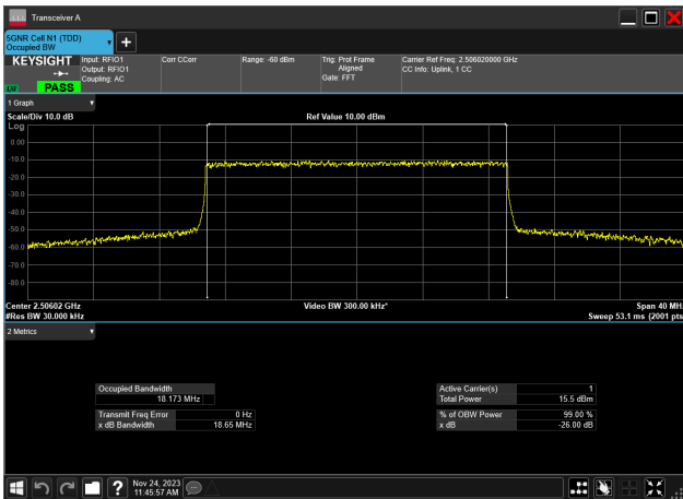
20MHz_30kHz_2506.02MHz_CP-OFDM 256 QAM_RB51@0 18.173 MHz
