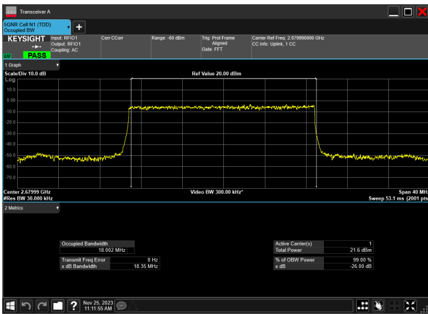
20MHz_30kHz_2679.99MHz_DFT-s-OFDM PI/2 BPSK_RB50@ 18.002 MHz
