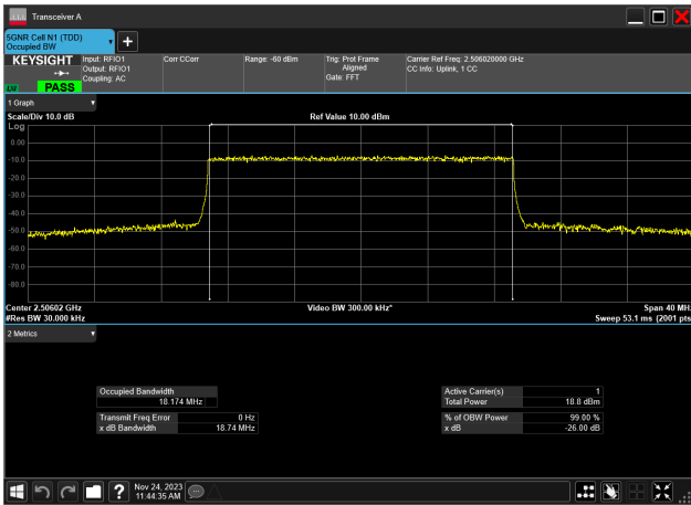
20MHz_30kHz_2506.02MHz_CP-OFDM 16 QAM_RB51@0 18.174 MHz
