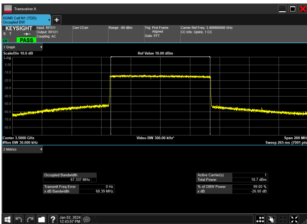
70MHz_30kHz_3500MHz_CP-OFDM 256 QAM_RB189@0 67.337 MHz
