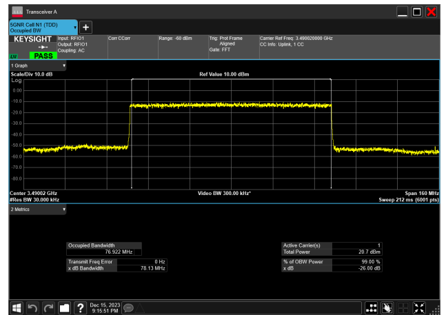
80MHz_30kHz_3490MHz_DFT-s-OFDM 64 QAM_RB216@ 76.922 MHz
