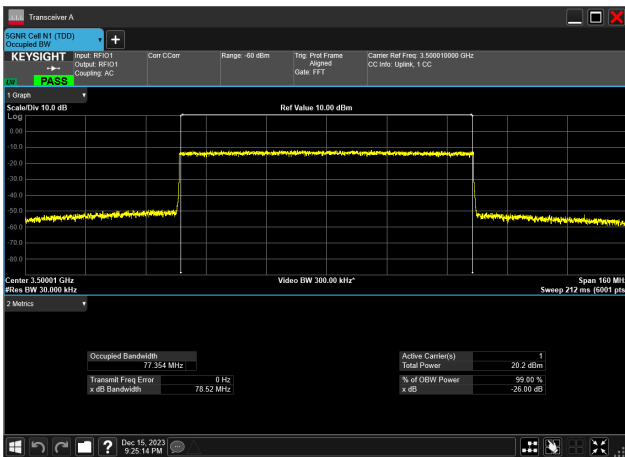
80MHz_30kHz_3500MHz_CP-OFDM 64 QAM_RB217@0 77.354 MHz
