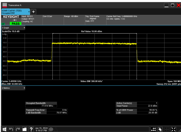
80MHz_30kHz_3500MHz_DFT-s-OFDM 16 QAM_RB216@0 77.014 MHz
