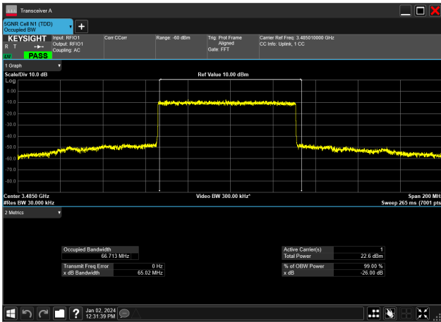
70MHz_30kHz_3485MHz_DFT-s-OFDM 64 QAM_RB180@0 66.713 MHz
