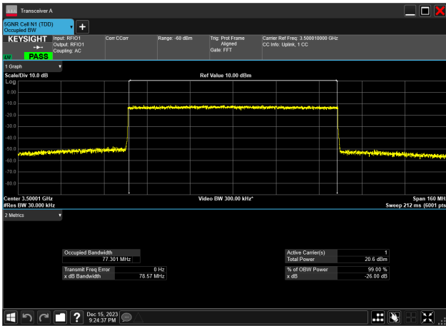
80MHz_30kHz_3500MHz_CP-OFDM 16 QAM_RB217@0 77.301 MHz
