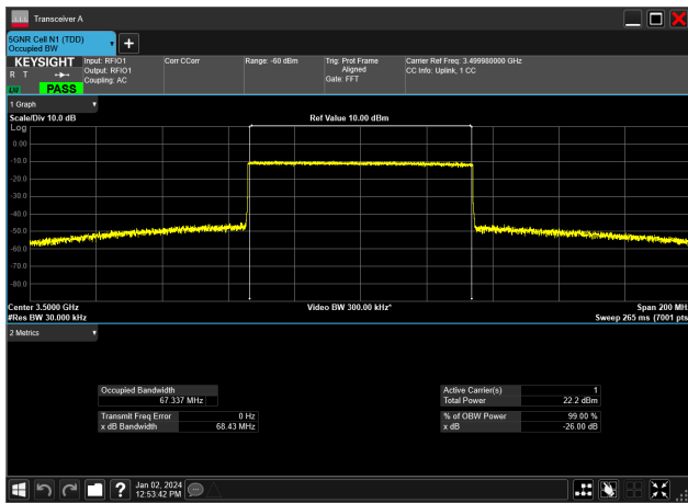
70MHz_30kHz_3500MHz_CP-OFDM QPSK_RB189@ 67.337 MHz
