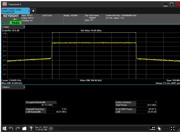
50MHz_15kHz_3955MHz_CP-OFDM 16 QAM_RB270@0 48.151 MHz
