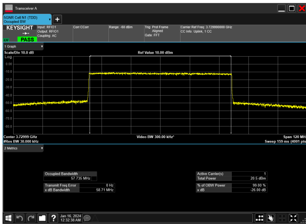
60MHz_30kHz_3730MHz_CP-OFDM 16 QAM_RB162@0 57.735 MHz
