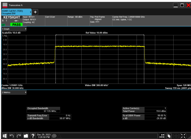
60MHz_30kHz_3950MHz_CP-OFDM 64 QAM_RB162@0 57.725 MHz
