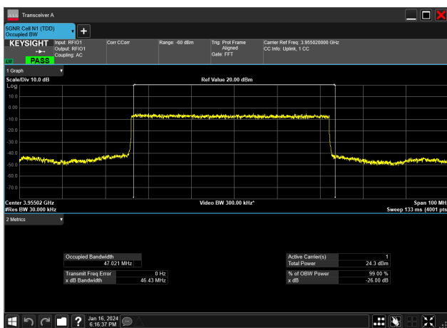
50MHz_30kHz_3955MHz_DFT-s-OFDM PI/2 BPSK_RB128@ 47.021 MHz
