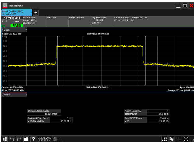
50MHz_30kHz_3840MHz_DFT-s-OFDM 16 QAM_RB128@ 47.005 MHz
