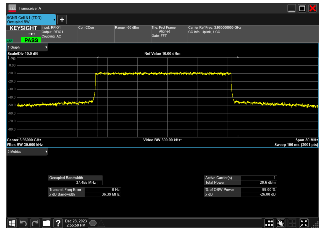
40MHz_30kHz_3960MHz_DFT-s-OFDM 64 QAM_RB100@0 37.455 MHz
