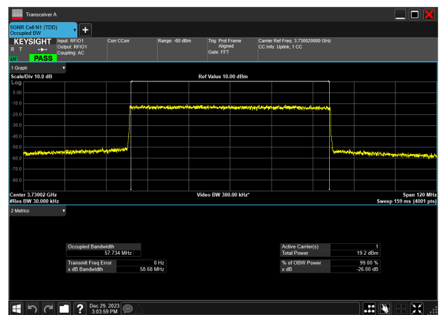
60MHz_30kHz_3730MHz_DFT-s-OFDM 256 QAM_RB162@0 57.734 MHz
