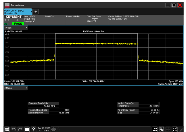
50MHz_30kHz_3725MHz_CP-OFDM 64 QAM_RB133@ 47.370 MHz
