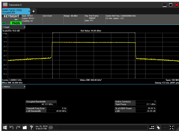
50MHz_15kHz_3840MHz_CP-OFDM QPSK_RB270@0 48.121 MHz
