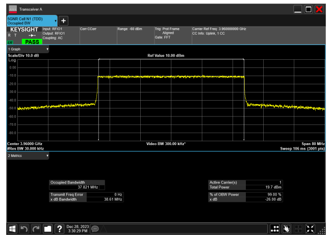
40MHz_30kHz_3960MHz_CP-OFDM 64 QAM_RB106@ 37.821 MHz
