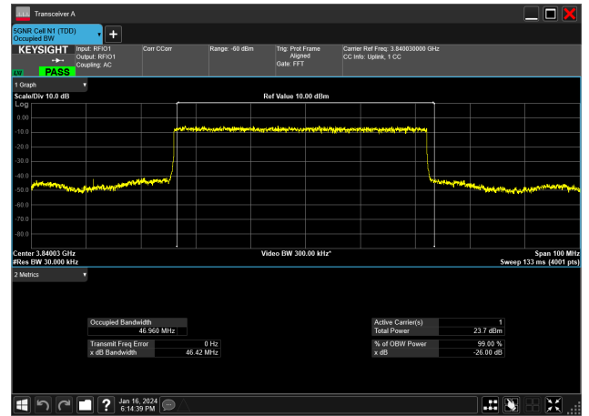
50MHz_30kHz_3840MHz_DFT-s-OFDM PI/2 BPSK_RB128@ 46.960 MHz
