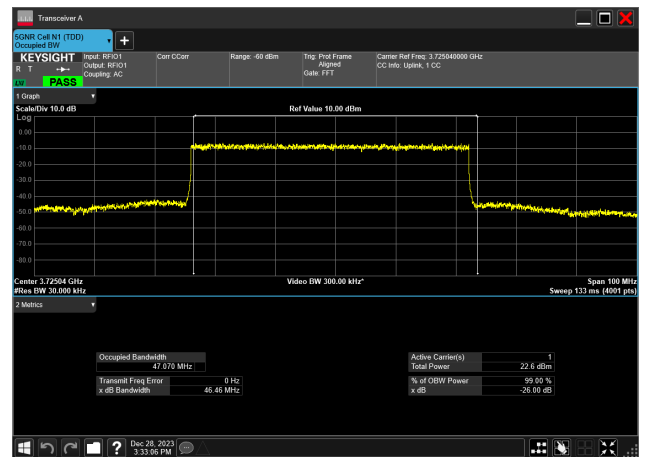
50MHz_30kHz_3725MHz_DFT-s-OFDM QPSK_RB128@ 47.070 MHz
