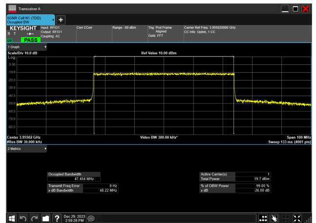
50MHz_30kHz_3955MHz_CP-OFDM 64 QAM_RB133@ 47.454 MHz
