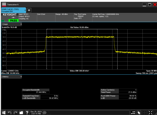
40MHz_30kHz_3840MHz_DFT-s-OFDM 16 QAM_RB100@0 37.444 MHz
