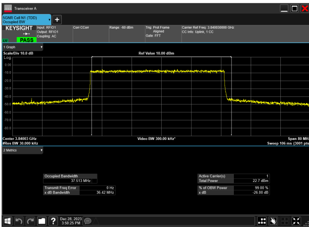
40MHz_30kHz_3840MHz_DFT-s-OFDM QPSK_RB100@ 37.513 MHz
