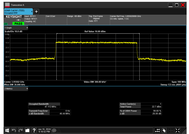
50MHz_30kHz_3955MHz_DFT-s-OFDM 16 QAM_RB128@ 47.113 MHz
