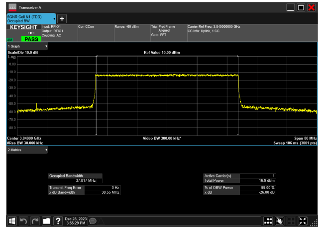
40MHz_30kHz_3840MHz_CP-OFDM 256 QAM_RB106@0 37.817 MHz
