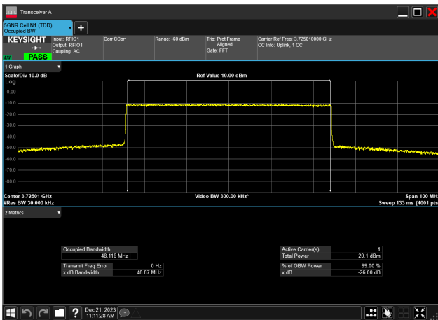
50MHz_15kHz_3725MHz_CP-OFDM 64 QAM_RB270@0 48.116 MHz
