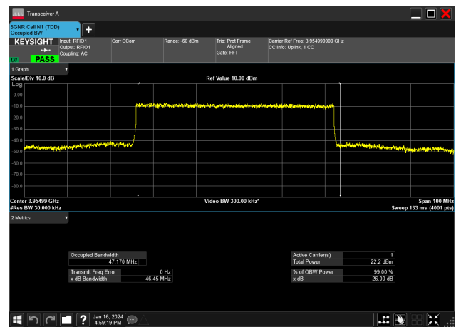
50MHz_30kHz_3955MHz_DFT-s-OFDM 64 QAM_RB128@ 47.170 MHz
