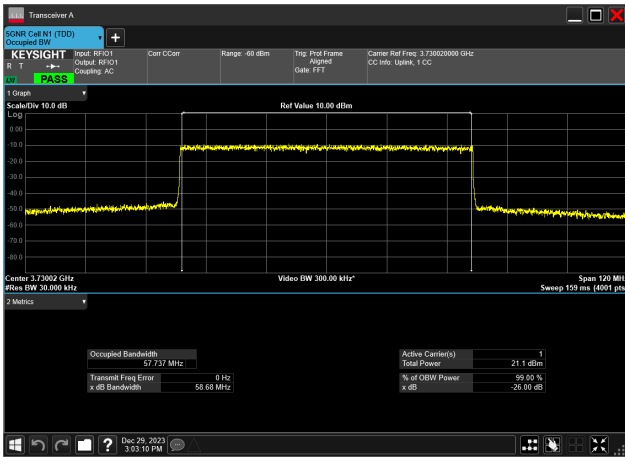
60MHz_30kHz_3730MHz_DFT-s-OFDM 64 QAM_RB162@0 57.737 MHz
