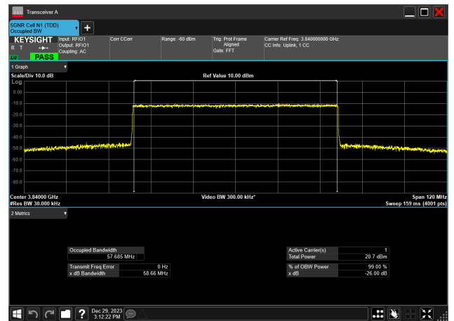
60MHz_30kHz_3840MHz_CP-OFDM 16 QAM_RB162@0 57.685 MHz
