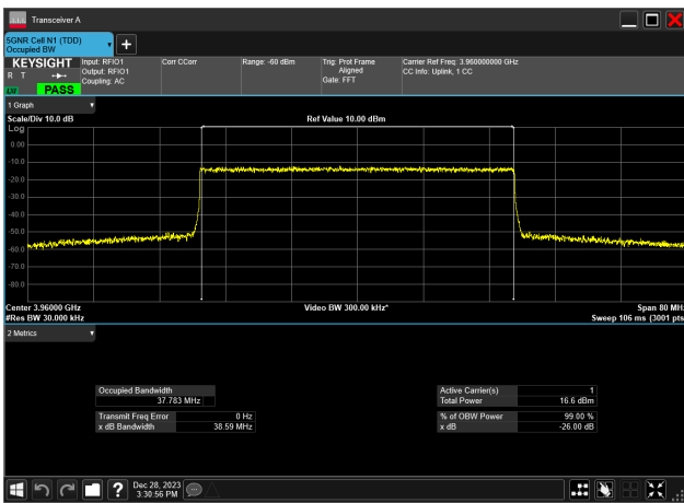
40MHz_30kHz_3960MHz_CP-OFDM 256 QAM_RB106@ 37.783 MHz
