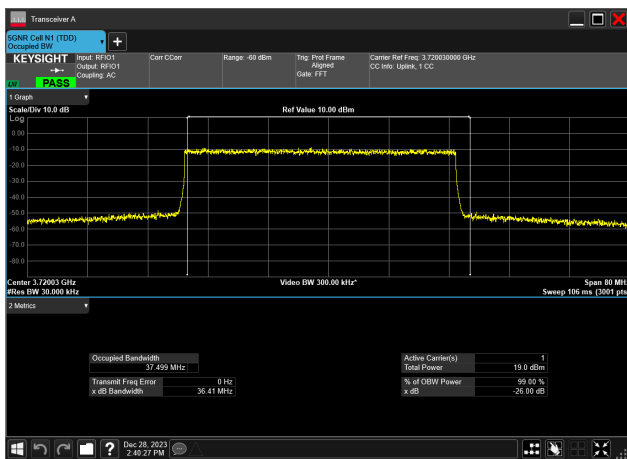
40MHz_30kHz_3720MHz_DFT-s-OFDM 256 QAM_RB100@ 37.499 MHz
