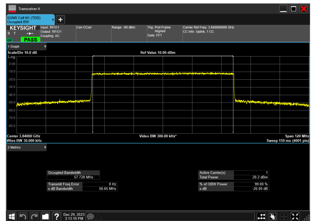
60MHz_30kHz_3840MHz_CP-OFDM 64 QAM_RB162@0 57.728 MHz
