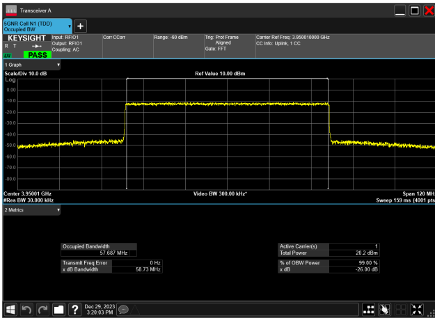
60MHz_30kHz_3950MHz_CP-OFDM 16 QAM_RB162@0 57.687 MHz
