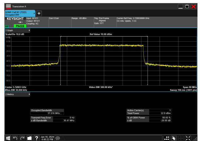
40MHz_30kHz_3720MHz_DFT-s-OFDM QPSK_RB100@ 37.516 MHz
