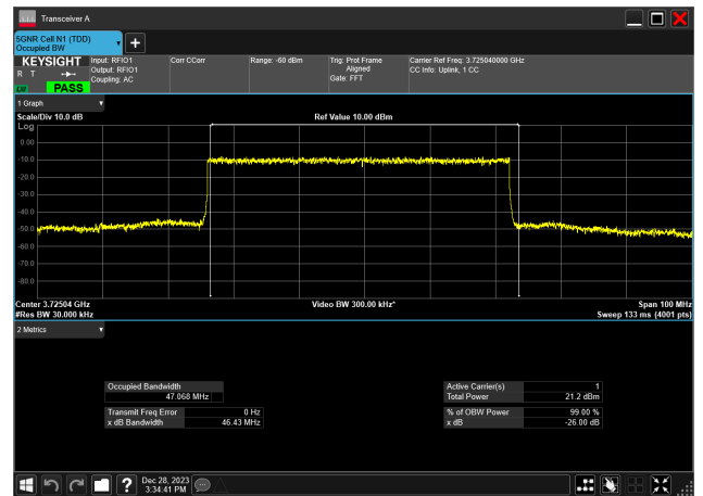
50MHz_30kHz_3725MHz_DFT-s-OFDM 64 QAM_RB128@ 47.068 MHz
