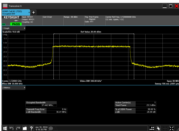
40MHz_30kHz_3720MHz_DFT-s-OFDM PI/2 BPSK_RB100@ 37.442 MHz
