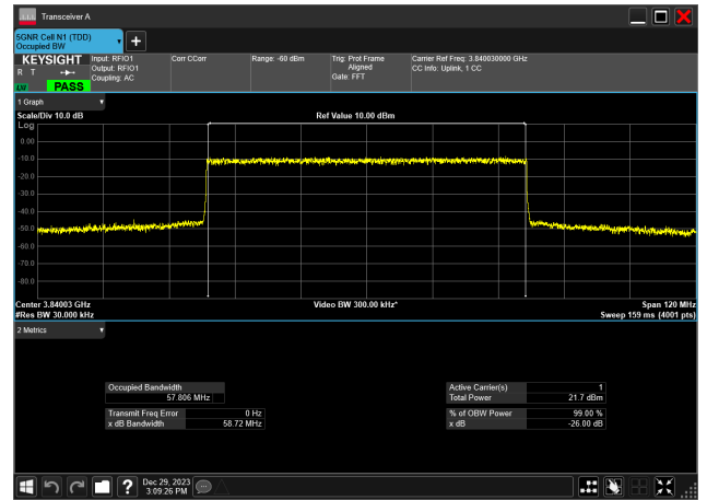
60MHz_30kHz_3840MHz_DFT-s-OFDM 16 QAM_RB162@0 57.806 MHz
