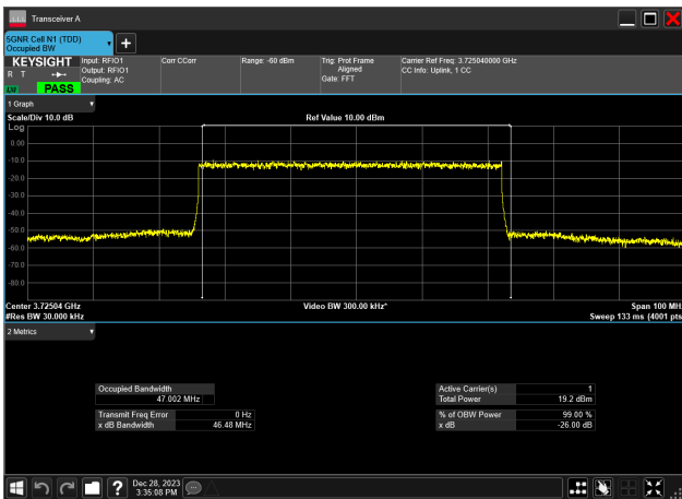
50MHz_30kHz_3725MHz_DFT-s-OFDM 256 QAM_RB128@ 47.002 MHz
