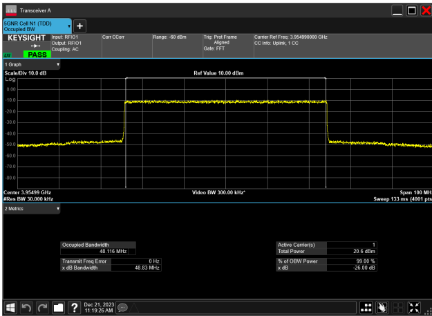
50MHz_15kHz_3955MHz_DFT-s-OFDM 64 QAM_RB270@ 48.116 MHz
