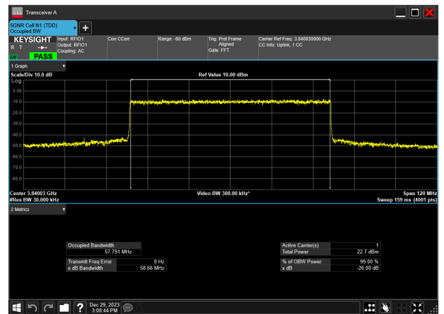
60MHz_30kHz_3840MHz_DFT-s-OFDM QPSK_RB162@0 57.791 MHz
