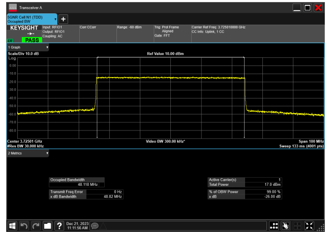
50MHz_15kHz_3725MHz_CP-OFDM 256 QAM_RB270@0 48.118 MHz
