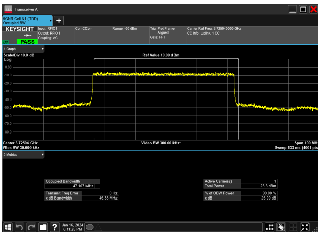
50MHz_30kHz_3725MHz_DFT-s-OFDM PI/2 BPSK_RB128@ 47.107 MHz
