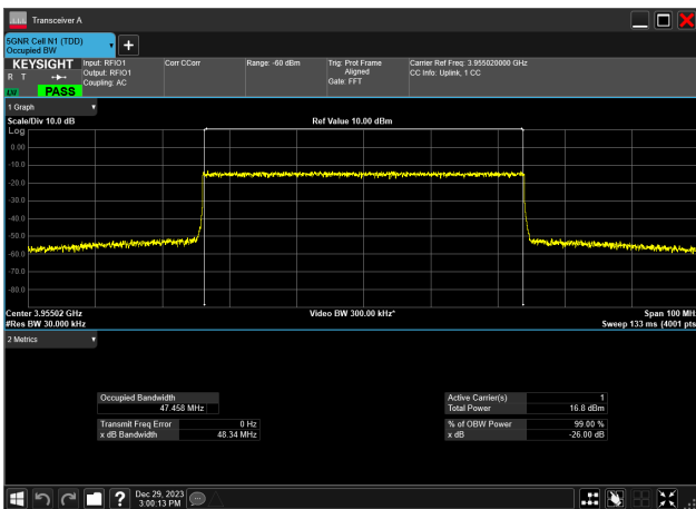
50MHz_30kHz_3955MHz_CP-OFDM 256 QAM_RB133@ 47.458 MHz
