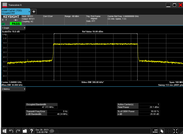
50MHz_30kHz_3840MHz_CP-OFDM 64 QAM_RB133@ 47.372 MHz
