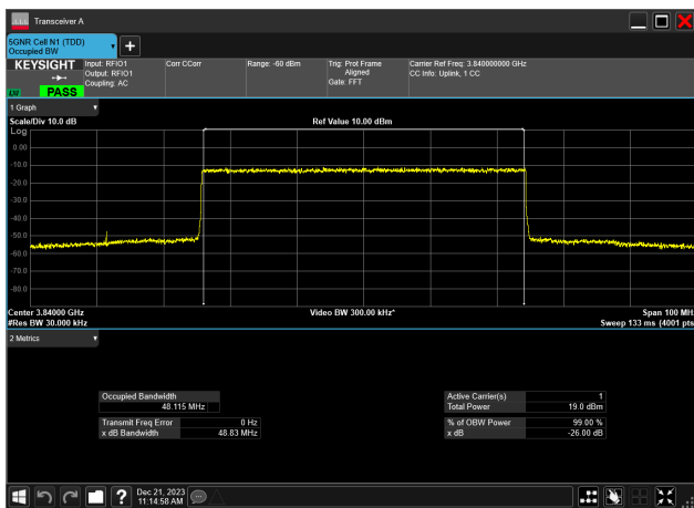
50MHz_15kHz_3840MHz_DFT-s-OFDM 256 QAM_RB270@0 48.115 MHz
