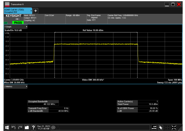
50MHz_15kHz_3955MHz_CP-OFDM 256 QAM_RB270@0 48.122 MHz
