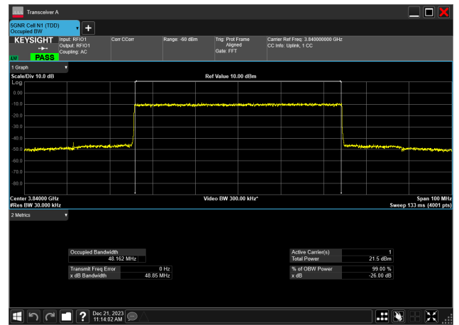
50MHz_15kHz_3840MHz_DFT-s-OFDM 16 QAM_RB270@0 48.162 MHz
