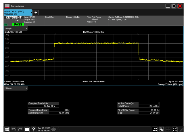
50MHz_15kHz_3840MHz_DFT-s-OFDM QPSK_RB270@0 48.122 MHz
