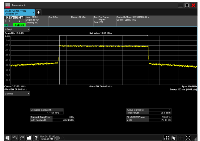
50MHz_30kHz_3725MHz_CP-OFDM 16 QAM_RB133@ 47.461 MHz
