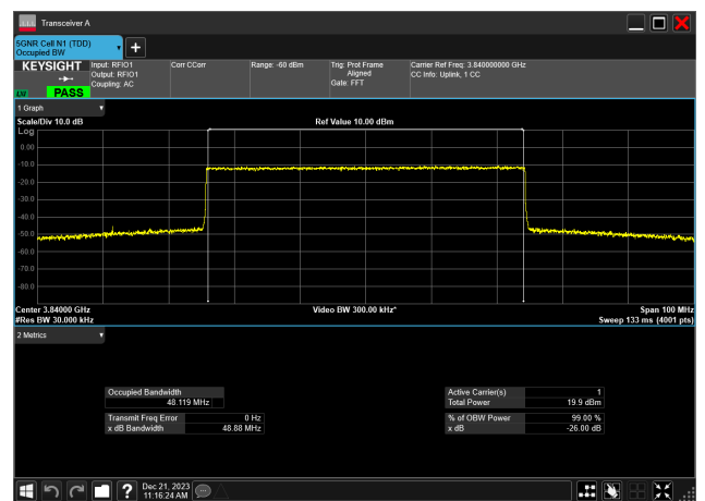
50MHz_15kHz_3840MHz_CP-OFDM 64 QAM_RB270@0 48.119 MHz
