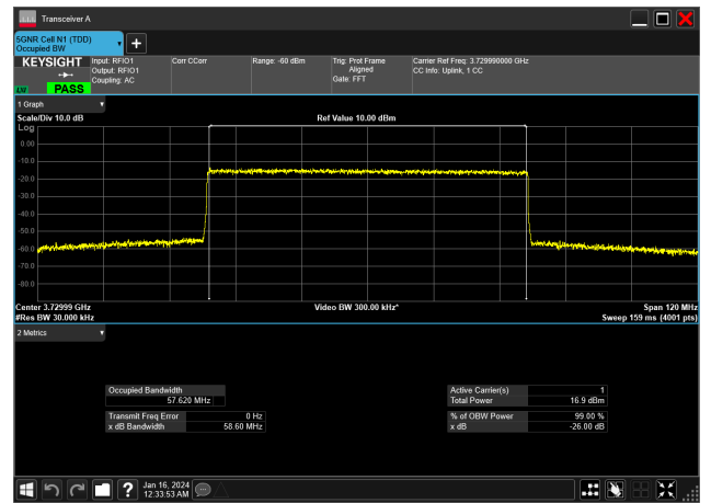
60MHz_30kHz_3730MHz_CP-OFDM 256 QAM_RB162@0 57.620 MHz
