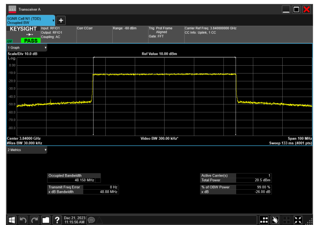
50MHz_15kHz_3840MHz_CP-OFDM 16 QAM_RB270@0 48.150 MHz
