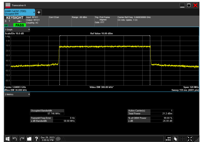
60MHz_30kHz_3840MHz_DFT-s-OFDM 64 QAM_RB162@0 57.746 MHz
