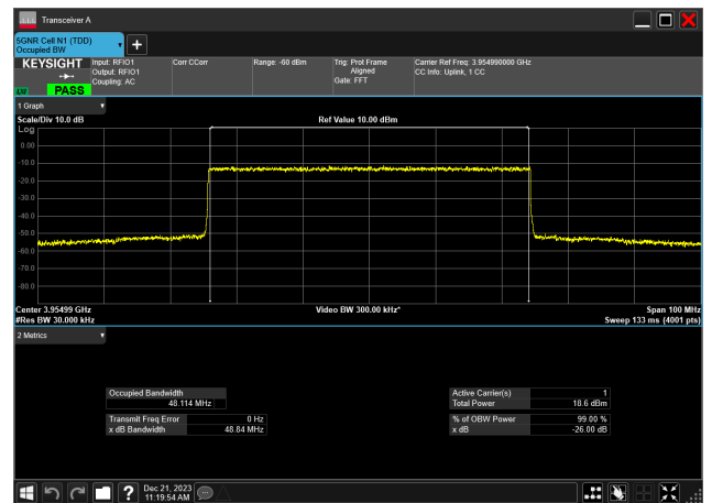
50MHz_15kHz_3955MHz_DFT-s-OFDM 256 QAM_RB270@0 48.114 MHz
