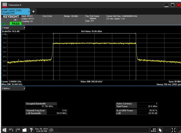
40MHz_30kHz_3840MHz_CP-OFDM 64 QAM_RB106@0 37.785 MHz
