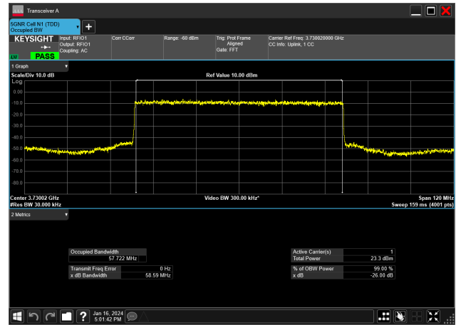
60MHz_30kHz_3730MHz_DFT-s-OFDM PI/2 BPSK_RB162@0 57.722 MHz
