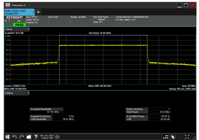
40MHz_30kHz_3840MHz_CP-OFDM QPSK_RB106@0 37.781 MHz
