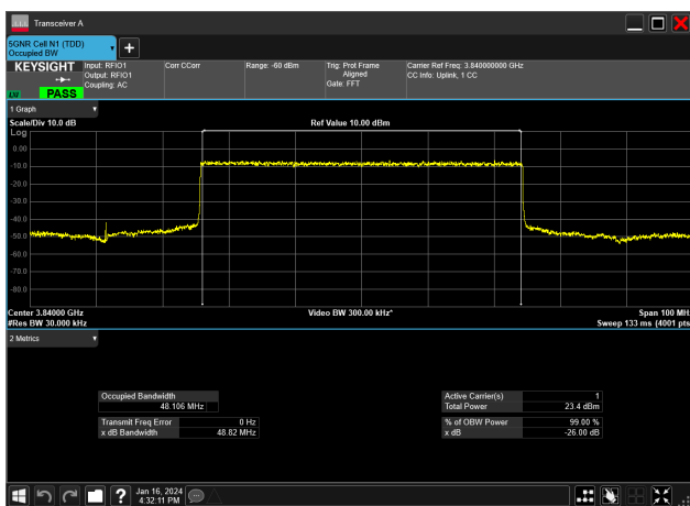
50MHz_15kHz_3840MHz_DFT-s-OFDM PI/2 BPSK_RB270@0 48.106 MHz
