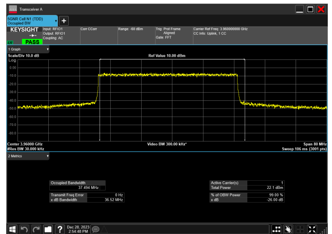
40MHz_30kHz_3960MHz_DFT-s-OFDM QPSK_RB100@0 37.494 MHz
