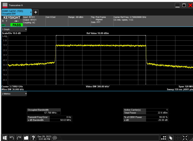
60MHz_30kHz_3730MHz_DFT-s-OFDM QPSK_RB162@0 57.788 MHz
