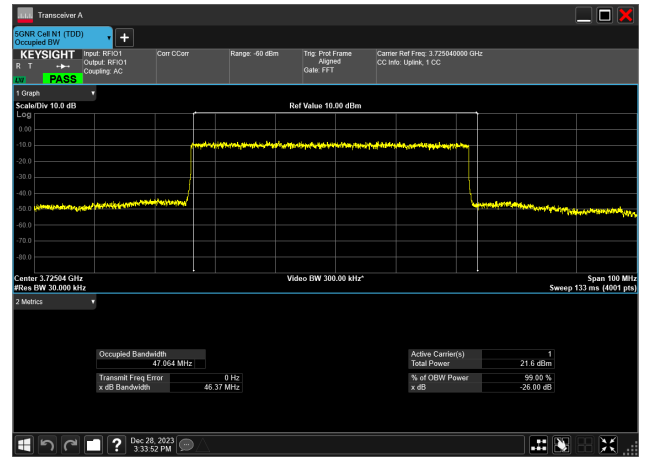
50MHz_30kHz_3725MHz_DFT-s-OFDM 16 QAM_RB128@ 47.064 MHz
