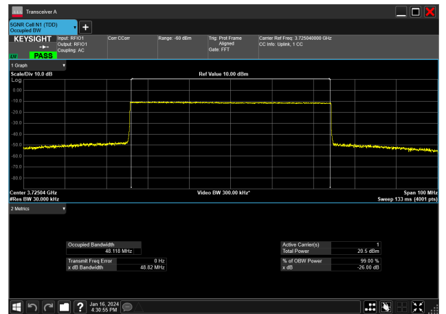
50MHz_15kHz_3725MHz_CP-OFDM QPSK_RB270@0 48.118 MHz
