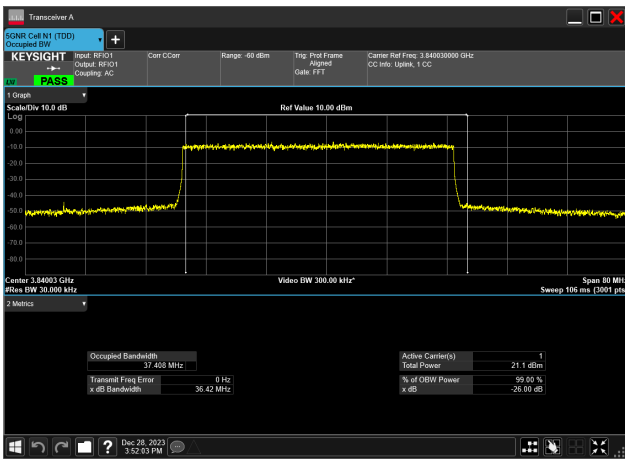
40MHz_30kHz_3840MHz_DFT-s-OFDM 64 QAM_RB100@ 37.408 MHz
