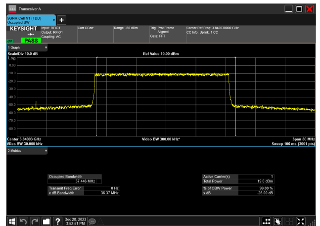
40MHz_30kHz_3840MHz_DFT-s-OFDM 256 QAM_RB100@0 37.446 MHz
