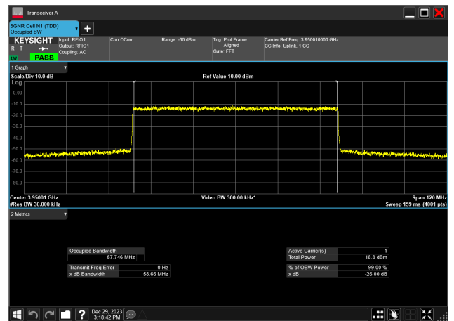
60MHz_30kHz_3950MHz_DFT-s-OFDM 256 QAM_RB162@0 57.746 MHz
