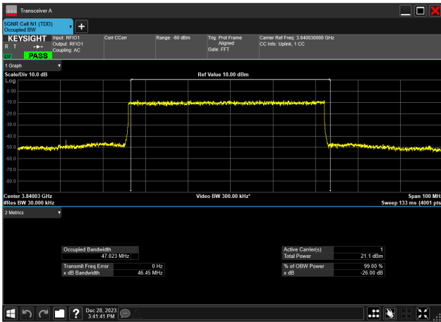
50MHz_30kHz_3840MHz_DFT-s-OFDM 64 QAM_RB128@ 47.023 MHz
