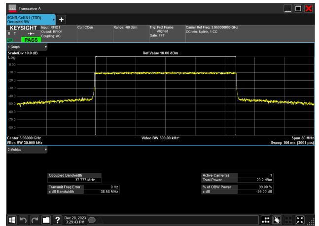
40MHz_30kHz_3960MHz_CP-OFDM 16 QAM_RB106@ 37.777 MHz
