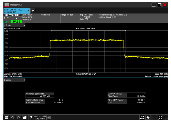
50MHz_30kHz_3840MHz_DFT-s-OFDM 256 QAM_RB128@ 46.909 MHz
