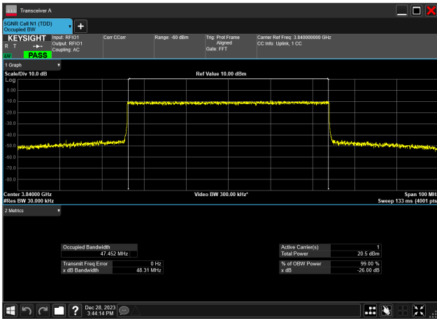
50MHz_30kHz_3840MHz_CP-OFDM 16 QAM_RB133@ 47.452 MHz
