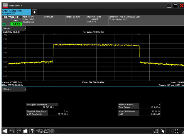
60MHz_30kHz_3730MHz_CP-OFDM 64 QAM_RB162@0 57.745 MHz
