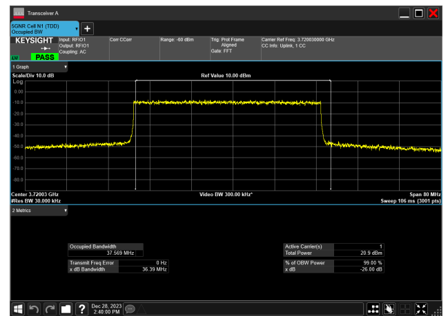
40MHz_30kHz_3720MHz_DFT-s-OFDM 64 QAM_RB100@ 37.569 MHz
