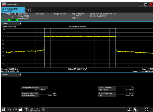
50MHz_15kHz_3725MHz_DFT-s-OFDM 16 QAM_RB270@0 48.157 MHz
