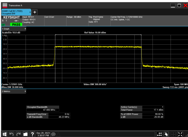
50MHz_30kHz_3725MHz_CP-OFDM 256 QAM_RB133@ 47.406 MHz
