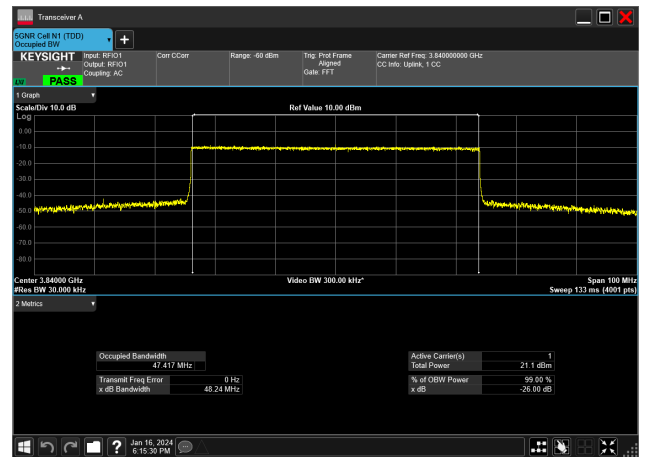
50MHz_30kHz_3840MHz_CP-OFDM QPSK_RB133@ 47.417 MHz
