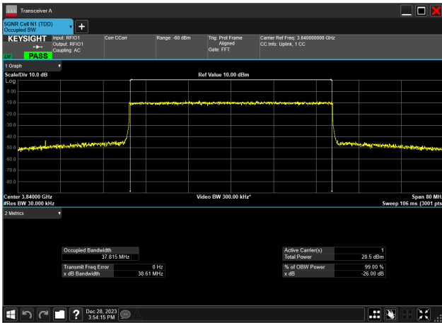
40MHz_30kHz_3840MHz_CP-OFDM 16 QAM_RB106@0 37.815 MHz
