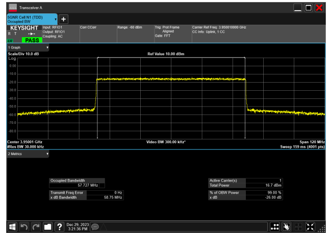
60MHz_30kHz_3950MHz_CP-OFDM 256 QAM_RB162@0 57.727 MHz
