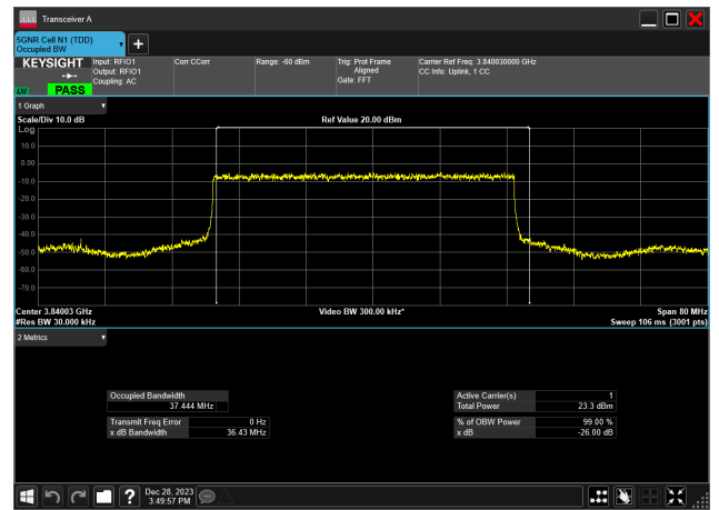
40MHz_30kHz_3840MHz_DFT-s-OFDM PI/2 BPSK_RB100@ 37.444 MHz
