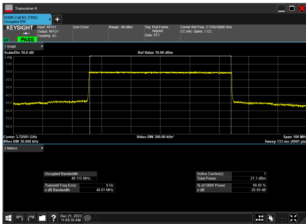
50MHz_15kHz_3725MHz_DFT-s-OFDM 64 QAM_RB270@0 48.115 MHz
