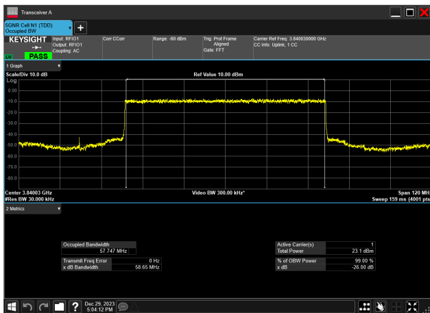
60MHz_30kHz_3840MHz_DFT-s-OFDM PI/2 BPSK_RB162@0 57.747 MHz
