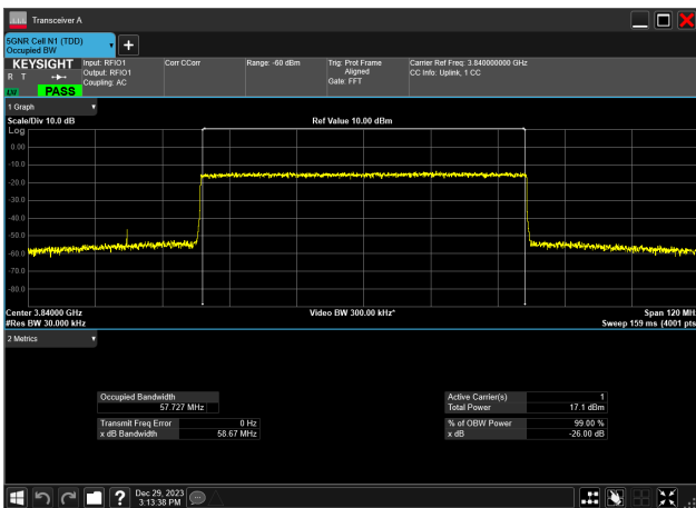
60MHz_30kHz_3840MHz_CP-OFDM 256 QAM_RB162@0 57.727 MHz
