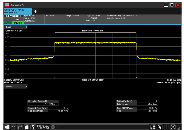
50MHz_30kHz_3955MHz_CP-OFDM 16 QAM_RB133@ 47.410 MHz
