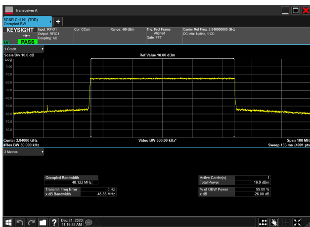
50MHz_15kHz_3840MHz_CP-OFDM 256 QAM_RB270@0 48.122 MHz
