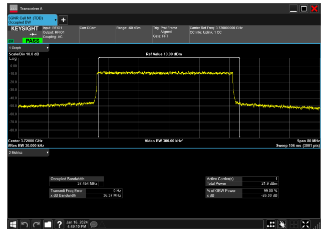
40MHz_30kHz_3720MHz_DFT-s-OFDM 16 QAM_RB100@ 37.454 MHz
