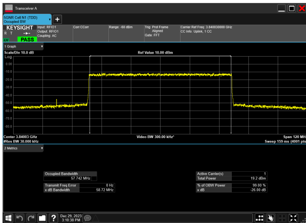
60MHz_30kHz_3840MHz_DFT-s-OFDM 256 QAM_RB162@0 57.742 MHz
