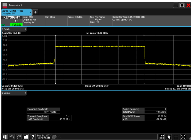
50MHz_15kHz_3955MHz_CP-OFDM 64 QAM_RB270@0 48.117 MHz
