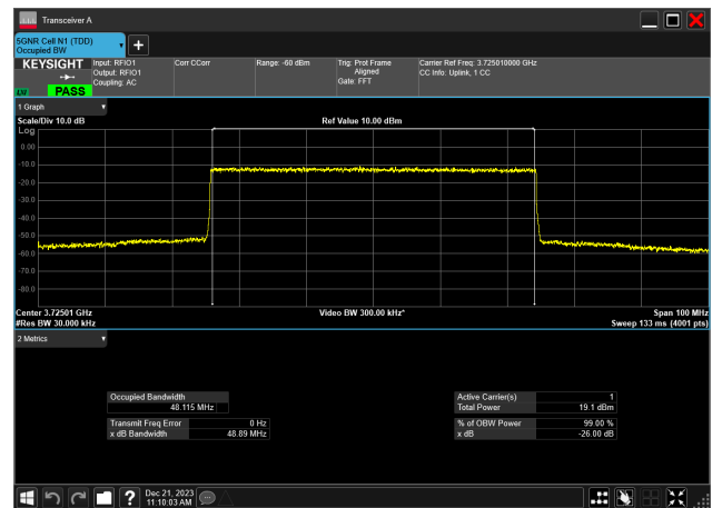
50MHz_15kHz_3725MHz_DFT-s-OFDM 256 QAM_RB270@0 48.115 MHz
