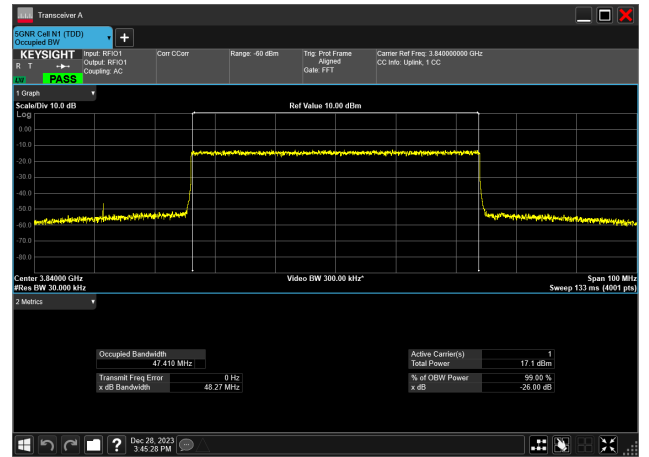
50MHz_30kHz_3840MHz_CP-OFDM 256 QAM_RB133@ 47.410 MHz
