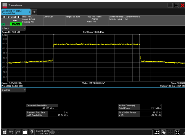
50MHz_15kHz_3955MHz_DFT-s-OFDM 16 QAM_RB270@0 48.163 MHz
