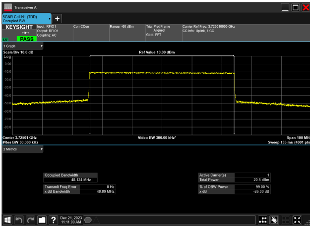
50MHz_15kHz_3725MHz_CP-OFDM 16 QAM_RB270@0 48.124 MHz
