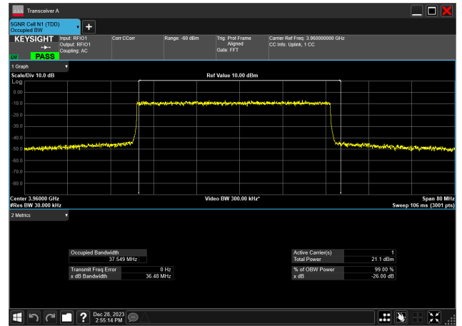
40MHz_30kHz_3960MHz_DFT-s-OFDM 16 QAM_RB100@0 37.549 MHz
