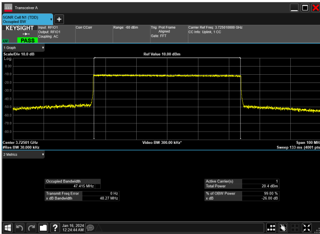
50MHz_30kHz_3725MHz_CP-OFDM QPSK_RB133@ 47.415 MHz
