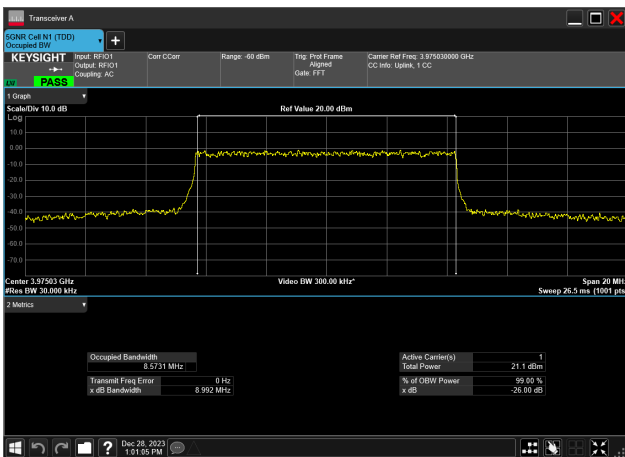
10MHz_30kHz_3975MHz_DFT-s-OFDM 16 QAM_RB24@0 8.573 MHz
