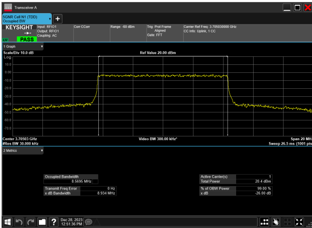
10MHz_30kHz_3705MHz_CP-OFDM 16 QAM_RB24@ 8.569 MHz
