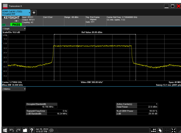
20MHz_15kHz_3710MHz_DFT-s-OFDM PI/2 BPSK_RB100@ 18.766 MHz
