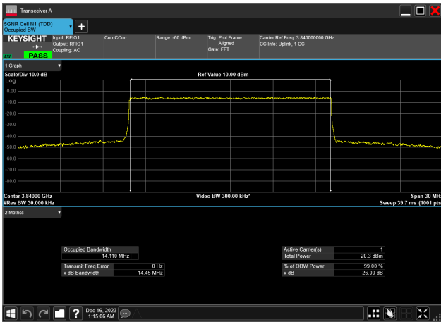
15MHz_15kHz_3840MHz_CP-OFDM 16 QAM_RB79@ 14.110 MHz
