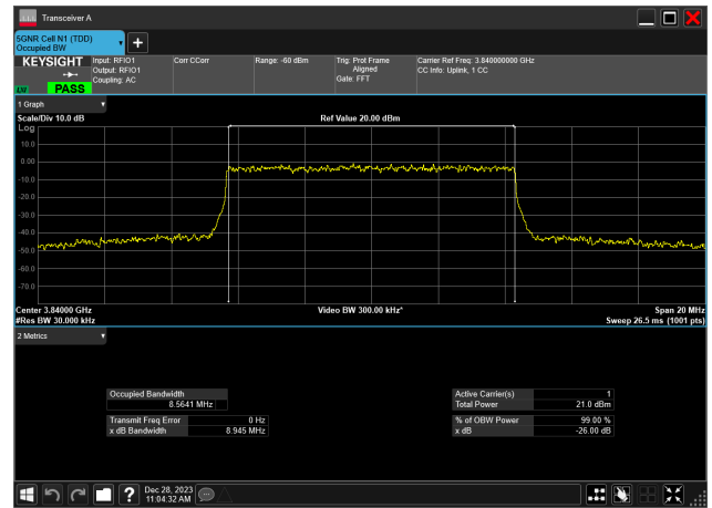
10MHz_30kHz_3840MHz_DFT-s-OFDM 64 QAM_RB24@0 8.564 MHz
