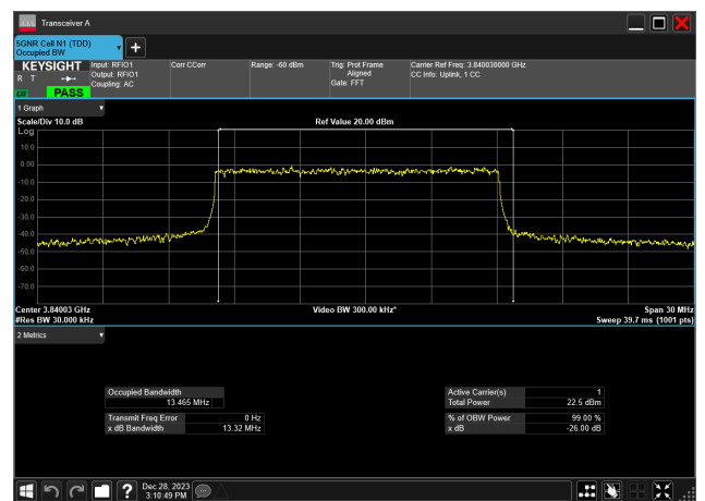
15MHz_30kHz_3840MHz_DFT-s-OFDM QPSK_RB36@ 13.465 MHz
