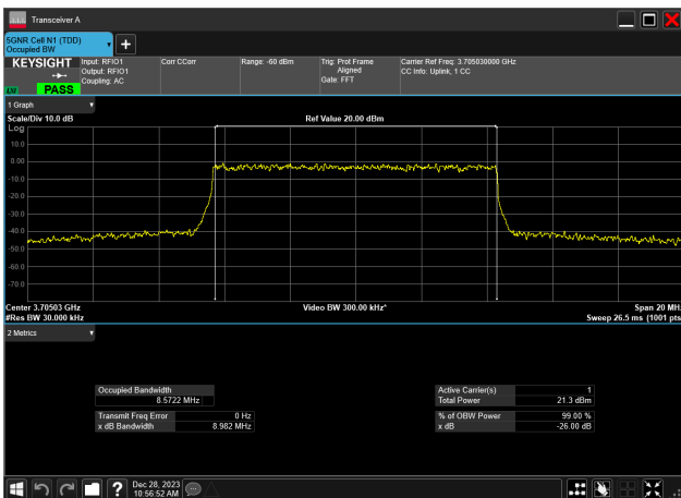
10MHz_30kHz_3705MHz_DFT-s-OFDM 16 QAM_RB24@ 8.572 MHz
