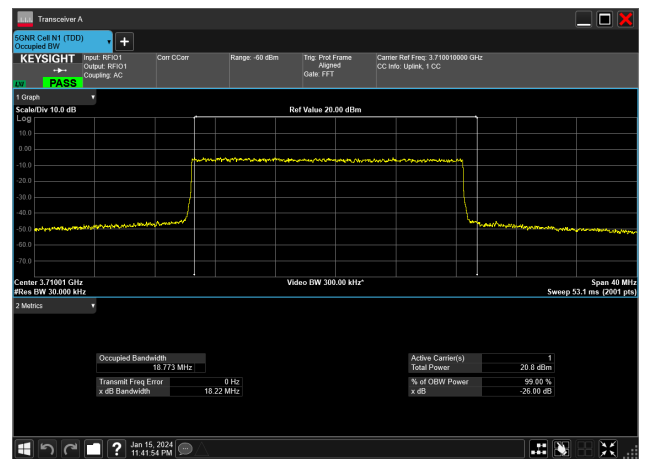
20MHz_15kHz_3710MHz_DFT-s-OFDM 64 QAM_RB100@ 18.773 MHz
