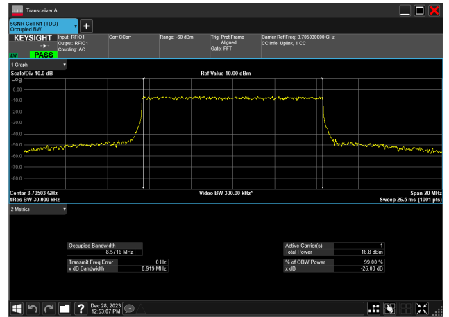
10MHz_30kHz_3705MHz_CP-OFDM 256 QAM_RB24@ 8.572 MHz
