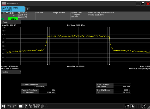
10MHz_30kHz_3975MHz_DFT-s-OFDM 64 QAM_RB24@0 8.567 MHz
