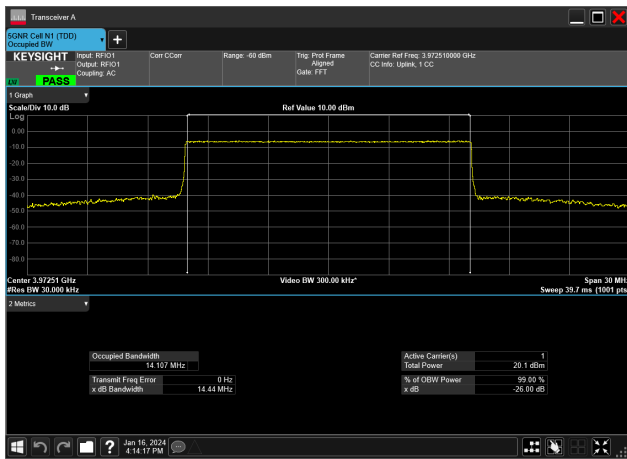
15MHz_15kHz_3972.5MHz_CP-OFDM QPSK_RB79@ 14.107 MHz
