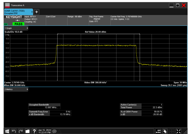
15MHz_15kHz_3707.5MHz_DFT-s-OFDM QPSK_RB75@ 13.997 MHz
