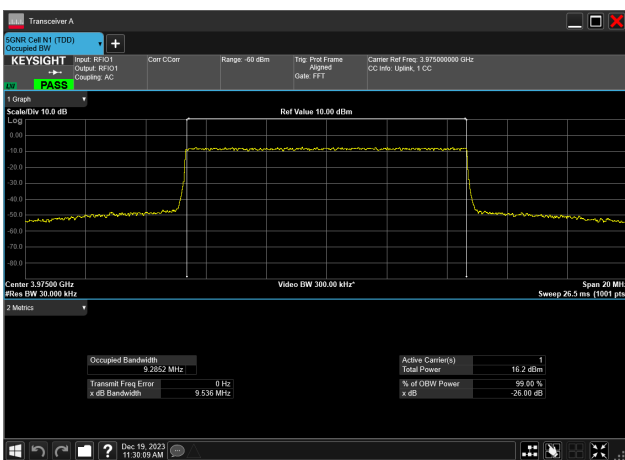
10MHz_15kHz_3975MHz_CP-OFDM 256 QAM_RB52@0 9.285 MHz
