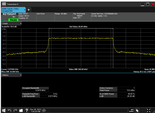
10MHz_30kHz_3975MHz_CP-OFDM 64 QAM_RB24@0 8.568 MHz
