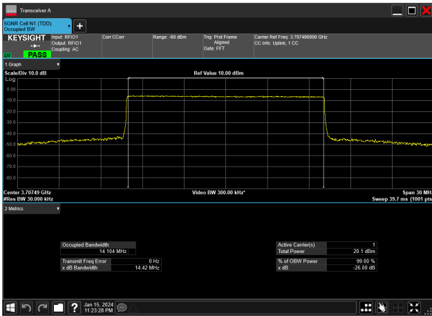
15MHz_15kHz_3707.5MHz_CP-OFDM QPSK_RB79@ 14.104 MHz
