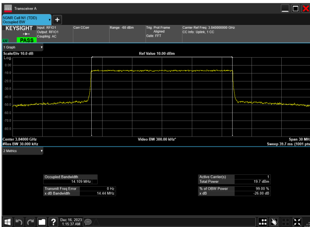
15MHz_15kHz_3840MHz_CP-OFDM 64 QAM_RB79@ 14.109 MHz
