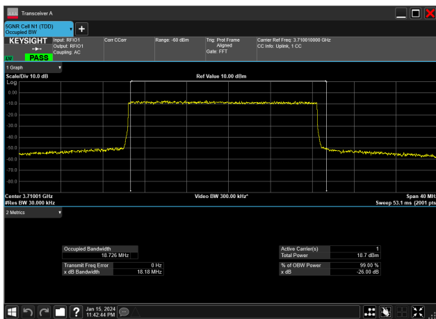
20MHz_15kHz_3710MHz_DFT-s-OFDM 256 QAM_RB100@ 18.726 MHz
