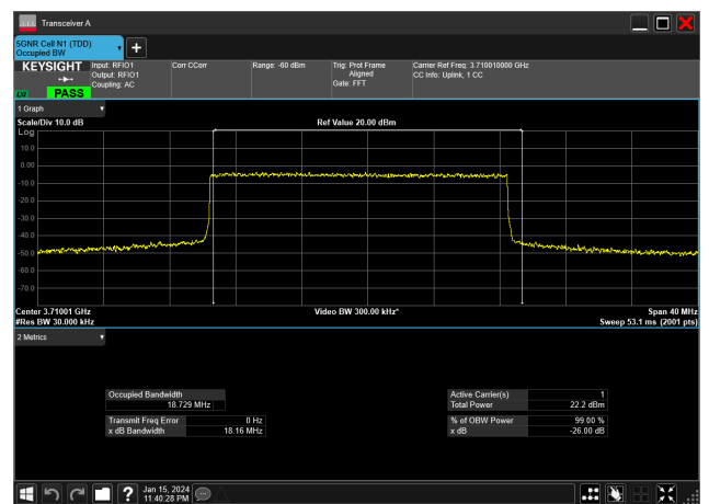
20MHz_15kHz_3710MHz_DFT-s-OFDM QPSK_RB100@ 18.729 MHz
