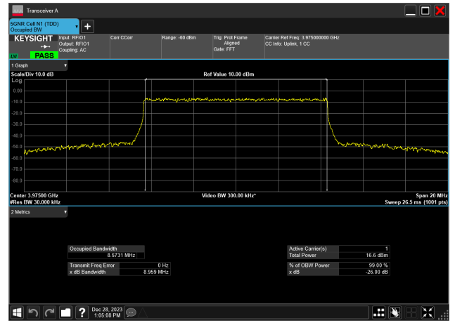
10MHz_30kHz_3975MHz_CP-OFDM 256 QAM_RB24@0 8.573 MHz
