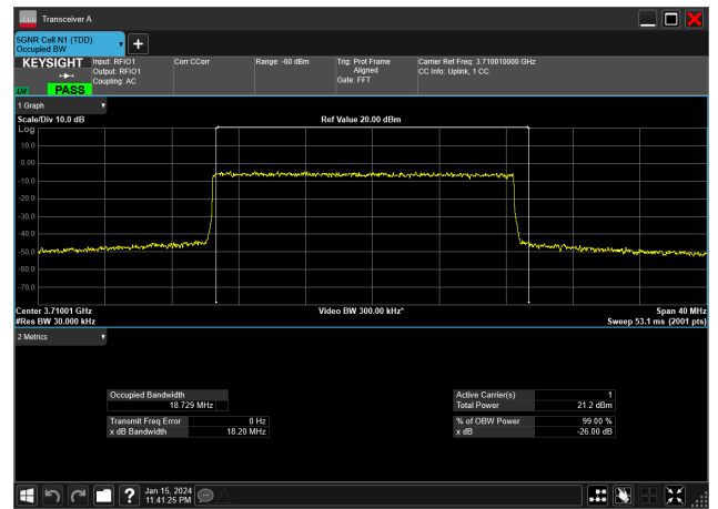
20MHz_15kHz_3710MHz_DFT-s-OFDM 16 QAM_RB100@ 18.729 MHz
