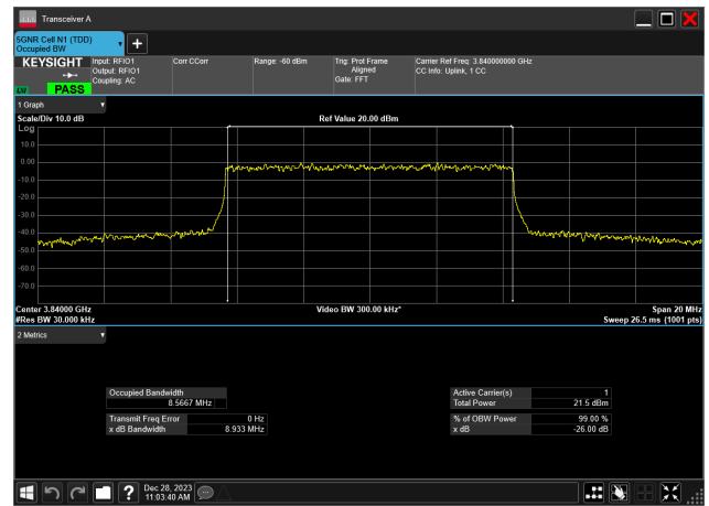
10MHz_30kHz_3840MHz_DFT-s-OFDM 16 QAM_RB24@0 8.567 MHz
