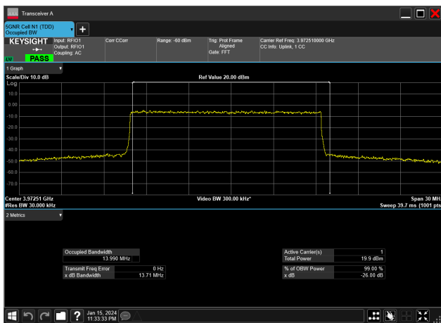
15MHz_15kHz_3972.5MHz_DFT-s-OFDM 256 QAM_RB75@ 13.990 MHz
