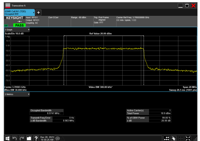
10MHz_30kHz_3705MHz_DFT-s-OFDM 256 QAM_RB24@ 8.574 MHz
