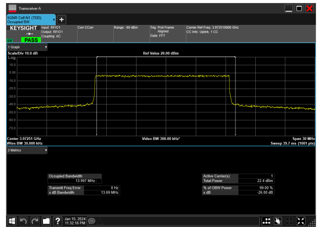
15MHz_15kHz_3972.5MHz_DFT-s-OFDM 16 QAM_RB75@ 13.997 MHz
