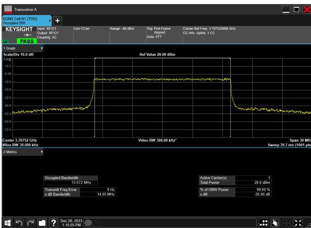
15MHz_30kHz_3707.5MHz_CP-OFDM 64 QAM_RB38@0 13.572 MHz
