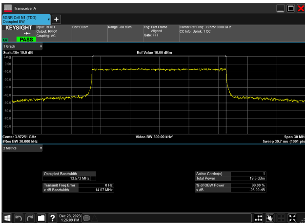
15MHz_30kHz_3972.5MHz_CP-OFDM 64 QAM_RB38@0 13.573 MHz
