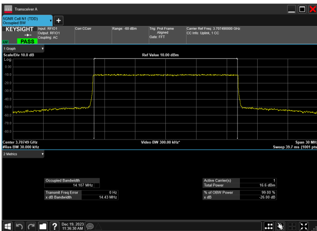
15MHz_15kHz_3707.5MHz_CP-OFDM 256 QAM_RB79@0 14.107 MHz
