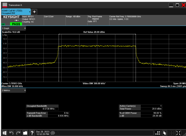
10MHz_30kHz_3705MHz_CP-OFDM 64 QAM_RB24@ 8.574 MHz
