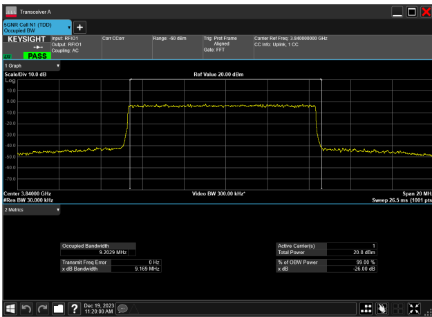
10MHz_15kHz_3840MHz_DFT-s-OFDM 64 QAM_RB50@0 9.203 MHz
