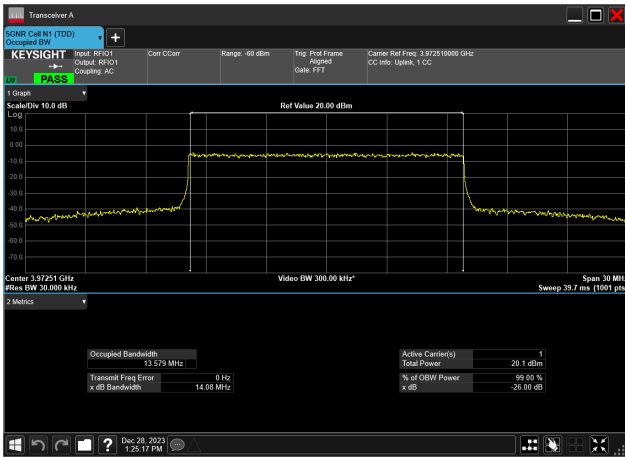
15MHz_30kHz_3972.5MHz_CP-OFDM 16 QAM_RB38@0 13.579 MHz
