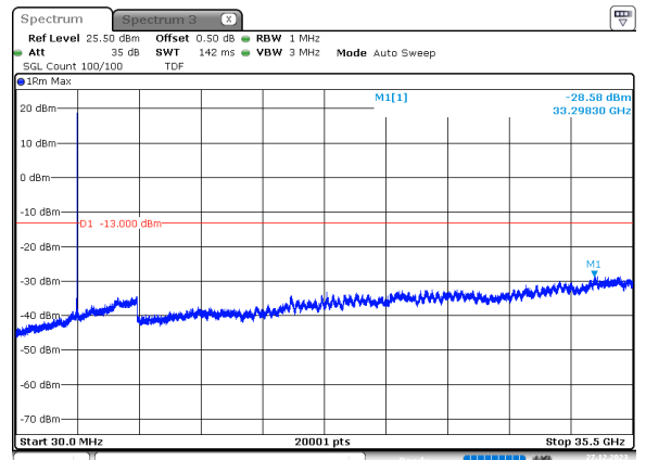
50MHz_30kHz_3525MHz_DFT-s-OFDM QPSK_RB1@132 -28.58 dBm
