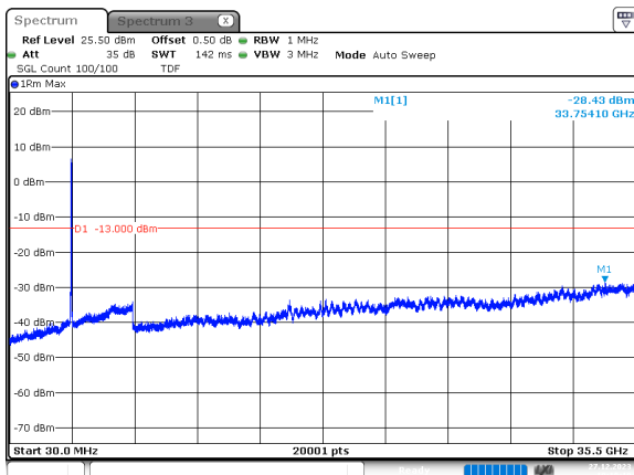
60MHz_30kHz_3500MHz_DFT-s-OFDM QPSK_RB162@0 -28.43 dBm
