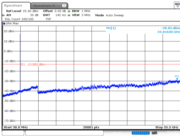
15MHz_30kHz_3457.5MHz_DFT-s-OFDM QPSK_RB1@0 -28.83 dBm
