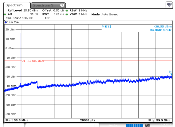
50MHz_30kHz_3475MHz_DFT-s-OFDM QPSK_RB1@132 -28.55 dBm
