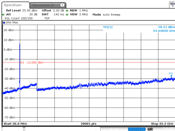
70MHz_30kHz_3515MHz_DFT-s-OFDM QPSK_RB180@0 -28.21 dBm
