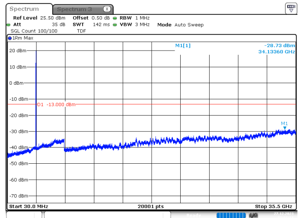
25MHz_30kHz_3500MHz_DFT-s-OFDM QPSK_RB1@64 -28.73 dBm
