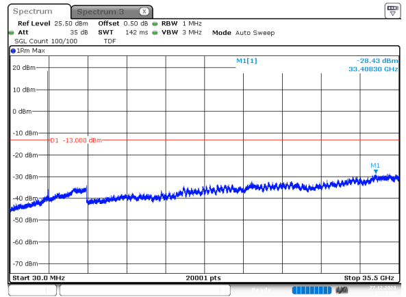
25MHz_30kHz_3462.5MHz_DFT-s-OFDM QPSK_RB1@0 -28.43 dBm
