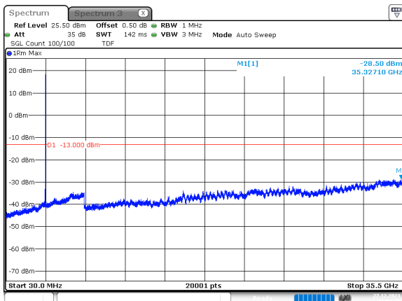
50MHz_30kHz_3500MHz_DFT-s-OFDM QPSK_RB1@132 -28.50 dBm
