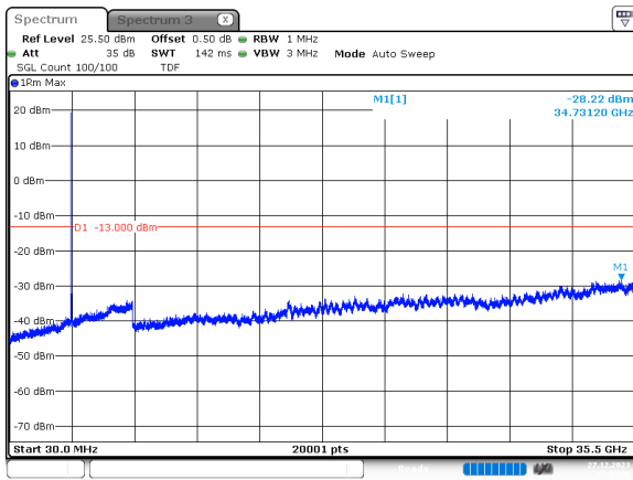
40MHz_30kHz_3500MHz_DFT-s-OFDM QPSK_RB1@0 -28.22 dBm
