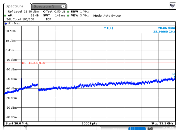
15MHz_30kHz_3500MHz_DFT-s-OFDM QPSK_RB36@0 -28.36 dBm
