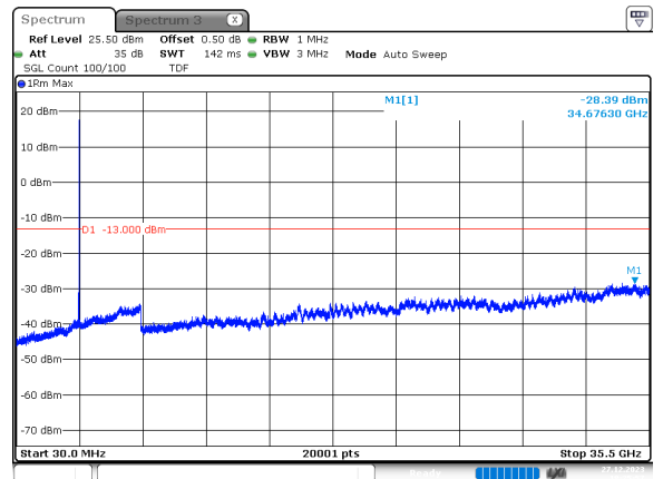
70MHz_30kHz_3515MHz_DFT-s-OFDM QPSK_RB1@188 -28.39 dBm
