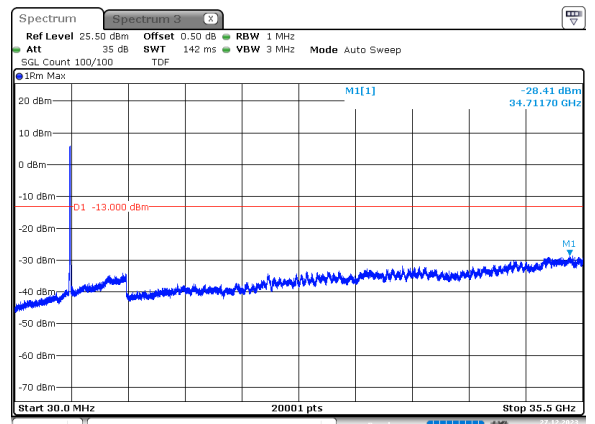
60MHz_30kHz_3480MHz_DFT-s-OFDM QPSK_RB162@0 -28.41 dBm
