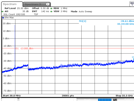
50MHz_30kHz_3475MHz_DFT-s-OFDM QPSK_RB1@0 -28.61 dBm
