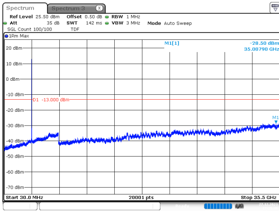
15MHz_30kHz_3542.5MHz_DFT-s-OFDM QPSK_RB36@0 -28.50 dBm
