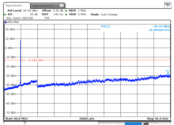
40MHz_30kHz_3470MHz_DFT-s-OFDM QPSK_RB100@0 -28.42 dBm
