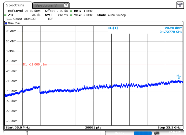
50MHz_30kHz_3500MHz_DFT-s-OFDM QPSK_RB1@0 -28.20 dBm
