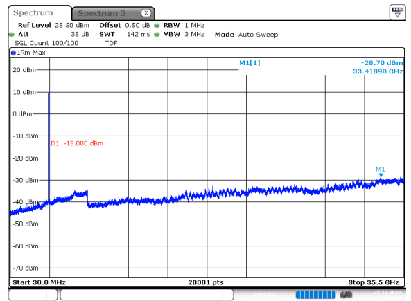
25MHz_30kHz_3462.5MHz_DFT-s-OFDM QPSK_RB64@0 -28.70 dBm
