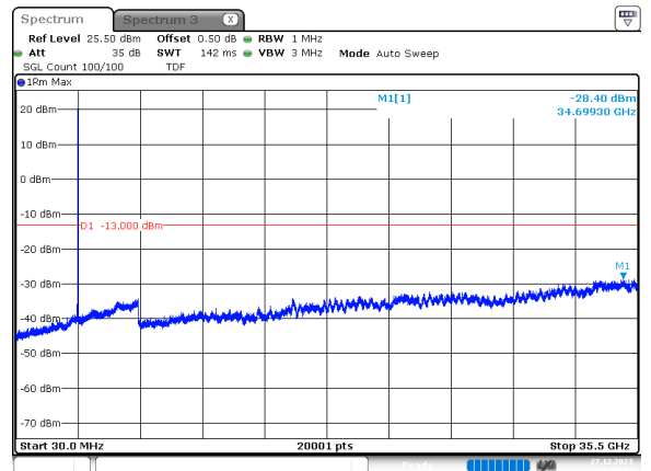
60MHz_30kHz_3500MHz_DFT-s-OFDM QPSK_RB1@161 -28.40 dBm
