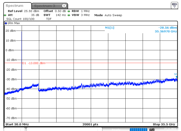
25MHz_30kHz_3537.5MHz_DFT-s-OFDM QPSK_RB1@0 -28.56 dBm
