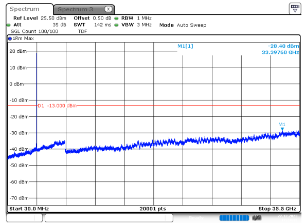
15MHz_30kHz_3542.5MHz_DFT-s-OFDM QPSK_RB1@37 -28.40 dBm
