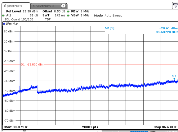
60MHz_30kHz_3480MHz_DFT-s-OFDM QPSK_RB1@161 -28.61 dBm
