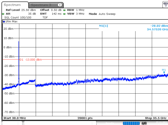
50MHz_30kHz_3475MHz_DFT-s-OFDM QPSK_RB128@0 -28.02 dBm
