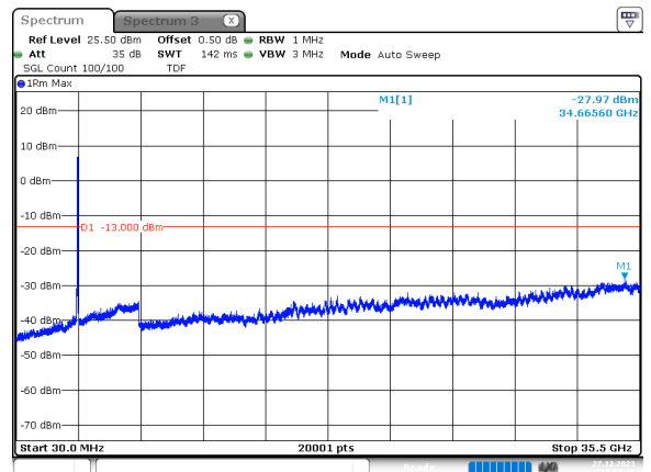
50MHz_30kHz_3500MHz_DFT-s-OFDM QPSK_RB128@0 -27.97 dBm
