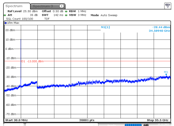
25MHz_30kHz_3537.5MHz_DFT-s-OFDM QPSK_RB64@0 -28.44 dBm
