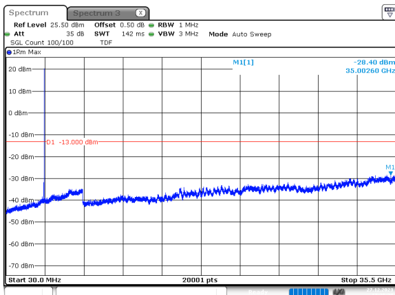
40MHz_30kHz_3470MHz_DFT-s-OFDM QPSK_RB1@105 -28.40 dBm
