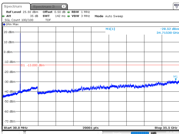
70MHz_30kHz_3500MHz_DFT-s-OFDM QPSK_RB1@188 -28.52 dBm
