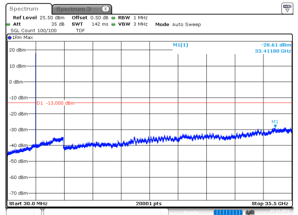
30MHz_30kHz_3535MHz_DFT-s-OFDM QPSK_RB1@77 -28.61 dBm
