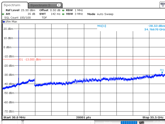
25MHz_30kHz_3500MHz_DFT-s-OFDM QPSK_RB1@0 -28.53 dBm
