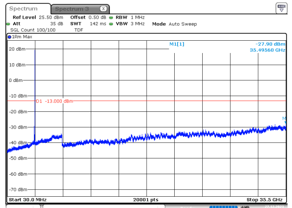
90MHz_30kHz_3505MHz_DFT-s-OFDM QPSK_RB1@244 -27.90 dBm
