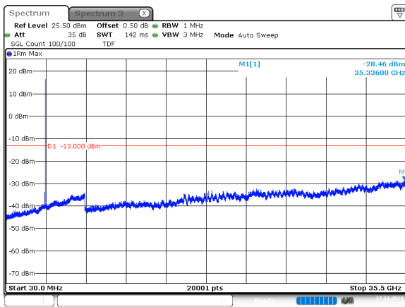
25MHz_30kHz_3462.5MHz_DFT-s-OFDM QPSK_RB1@64 -28.46 dBm
