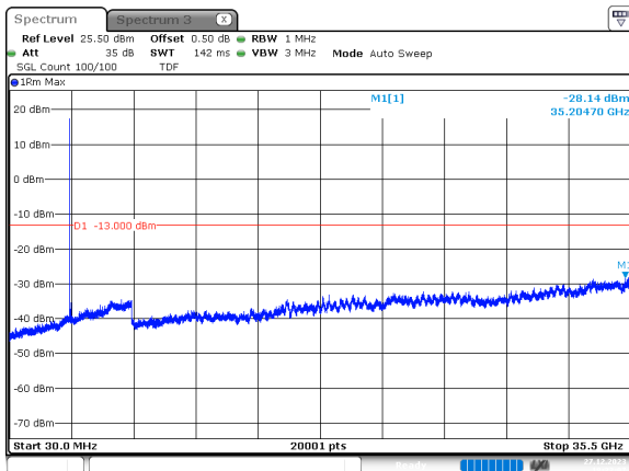
80MHz_30kHz_3500MHz_DFT-s-OFDM QPSK_RB1@0 -28.14 dBm
