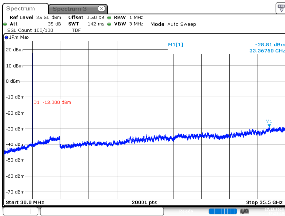
15MHz_30kHz_3542.5MHz_DFT-s-OFDM QPSK_RB1@0 -28.81 dBm
