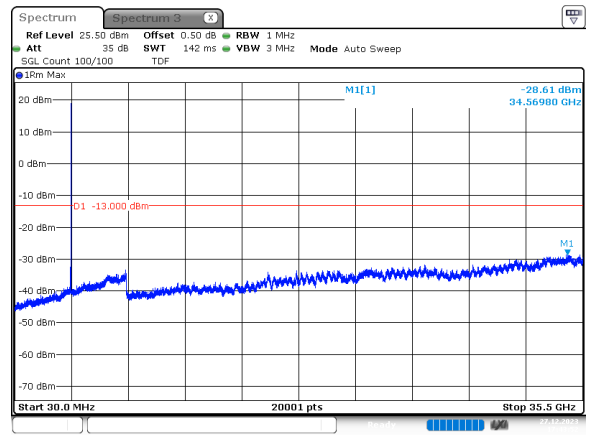
40MHz_30kHz_3500MHz_DFT-s-OFDM QPSK_RB1@105 -28.61 dBm
