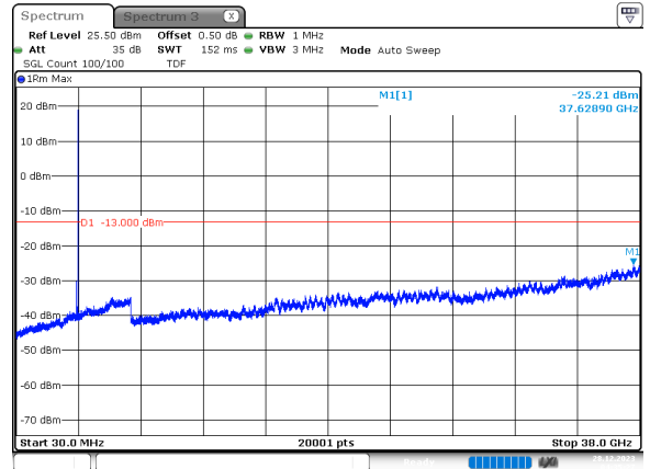
70MHz_30kHz_3735MHz_DFT-s-OFDM QPSK_RB1@188 -25.21 dBm
