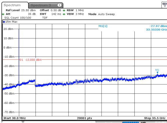
50MHz_30kHz_3525MHz_DFT-s-OFDM QPSK_RB1@0 -27.97 dBm
