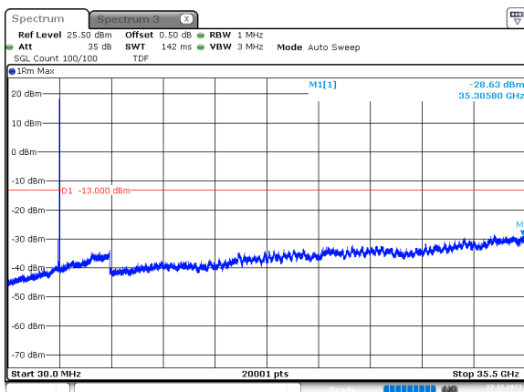
90MHz_30kHz_3500MHz_DFT-s-OFDM QPSK_RB1@244 -28.63 dBm
