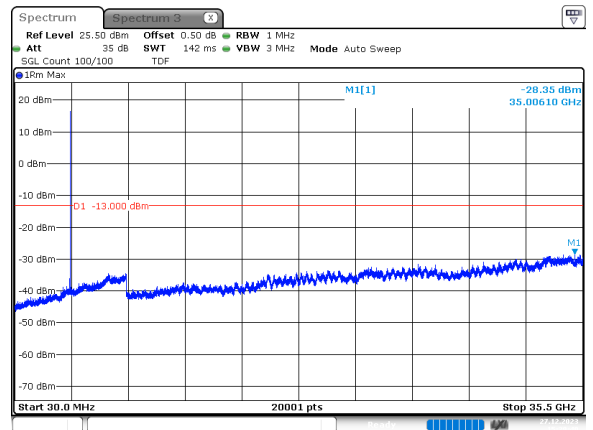
30MHz_30kHz_3465MHz_DFT-s-OFDM QPSK_RB1@77 -28.35 dBm
