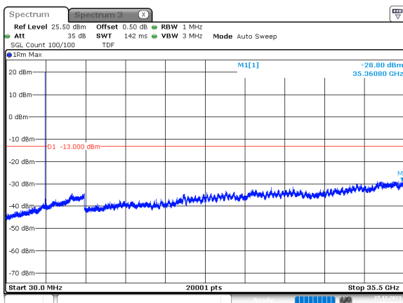
15MHz_30kHz_3500MHz_DFT-s-OFDM QPSK_RB1@37 -28.80 dBm
