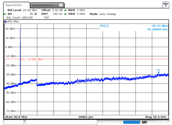
15MHz_30kHz_3457.5MHz_DFT-s-OFDM QPSK_RB1@37 -28.72 dBm
