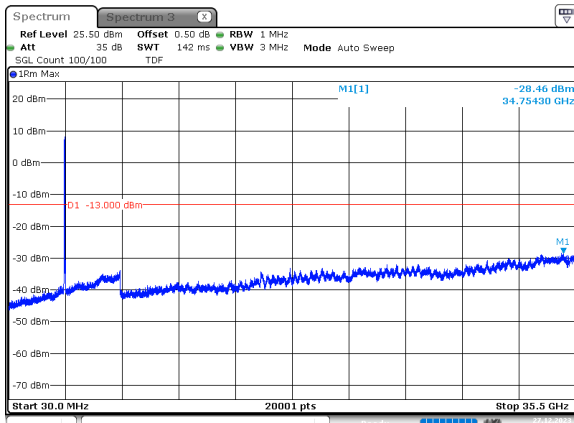
50MHz_30kHz_3525MHz_DFT-s-OFDM QPSK_RB128@0 -28.46 dBm
