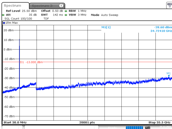
25MHz_30kHz_3500MHz_DFT-s-OFDM QPSK_RB64@0 -28.60 dBm
