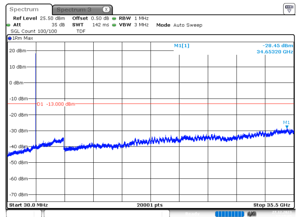
15MHz_30kHz_3500MHz_DFT-s-OFDM QPSK_RB1@0 -28.45 dBm
