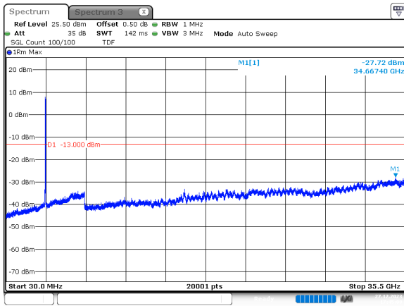
40MHz_30kHz_3500MHz_DFT-s-OFDM QPSK_RB100@0 -27.72 dBm
