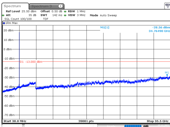
60MHz_30kHz_3520MHz_DFT-s-OFDM QPSK_RB1@161 -28.56 dBm
