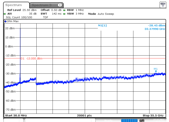
70MHz_30kHz_3485MHz_DFT-s-OFDM QPSK_RB1@188 -28.45 dBm
