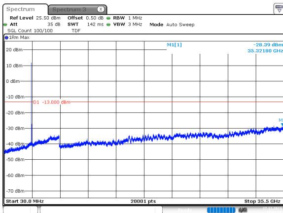
15MHz_30kHz_3457.5MHz_DFT-s-OFDM QPSK_RB36@0 -28.39 dBm
