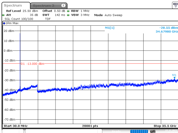
70MHz_30kHz_3515MHz_DFT-s-OFDM QPSK_RB1@0 -28.55 dBm
