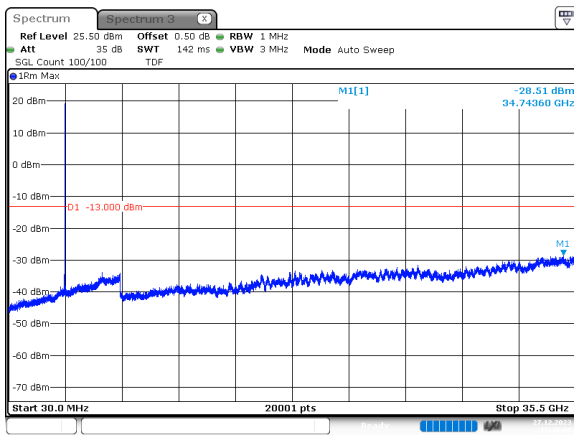
40MHz_30kHz_3530MHz_DFT-s-OFDM QPSK_RB1@105 -28.51 dBm
