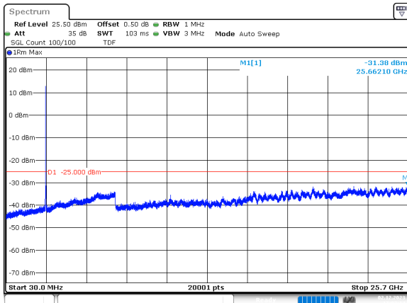
15MHz_15kHz_2535MHz_DFT-s-OFDM QPSK_RB75@0 -31.38 dBm
