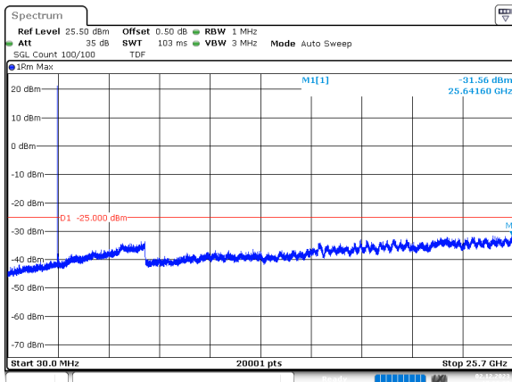
15MHz_15kHz_2535MHz_DFT-s-OFDM QPSK_RB1@0 -31.56 dBm
