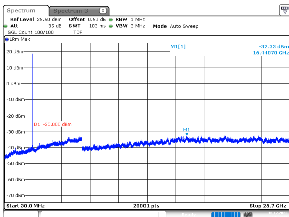
20MHz_15kHz_2535MHz_DFT-s-OFDM QPSK_RB1@105 -32.33 dBm
