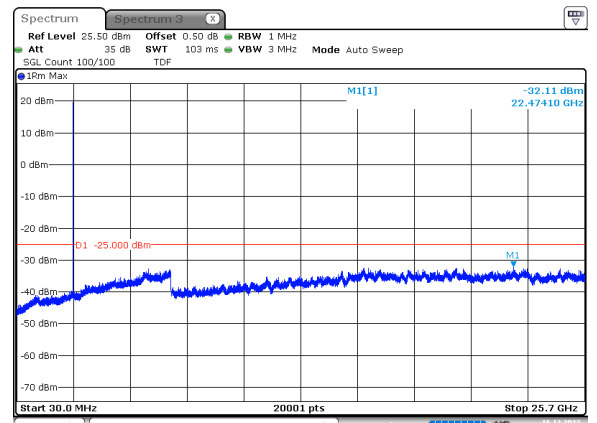
5MHz_15kHz_2567.5MHz_DFT-s-OFDM QPSK_RB1@0 -32.11 dBm
