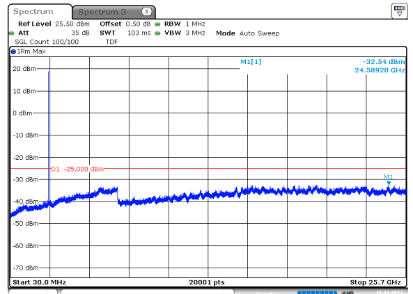
5MHz_15kHz_2502.5MHz_DFT-s-OFDM QPSK_RB1@0 -32.54 dBm
