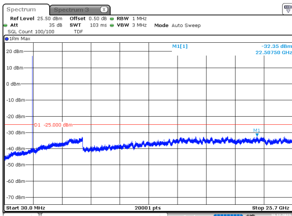
5MHz_15kHz_2502.5MHz_DFT-s-OFDM QPSK_RB1@24 -32.35 dBm
