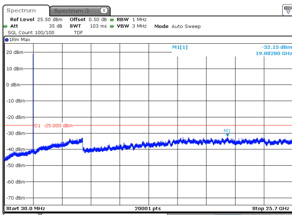
5MHz_15kHz_2567.5MHz_DFT-s-OFDM QPSK_RB1@24 -32.15 dBm
