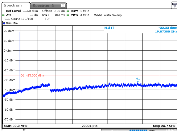
5MHz_15kHz_2535MHz_DFT-s-OFDM QPSK_RB1@0 -32.33 dBm
