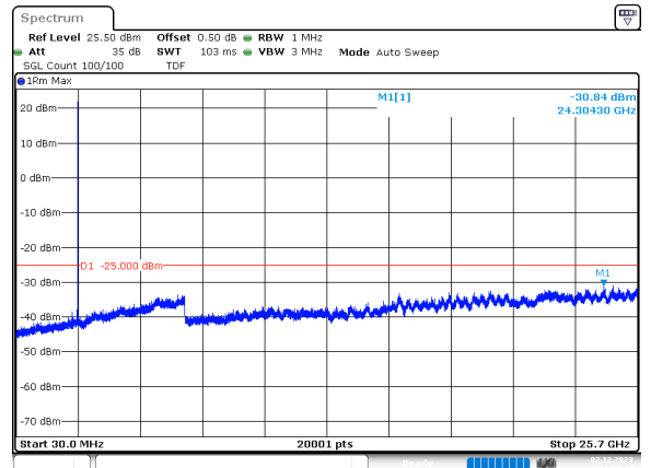
15MHz_15kHz_2562.5MHz_DFT-s-OFDM QPSK_RB1@0 -30.84 dBm
