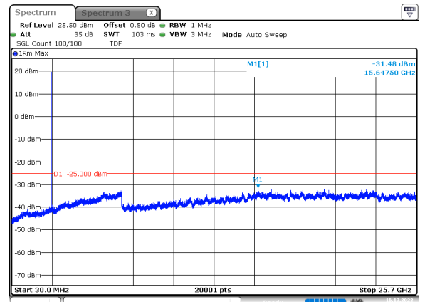
5MHz_15kHz_2535MHz_DFT-s-OFDM QPSK_RB1@24 -31.48 dBm
