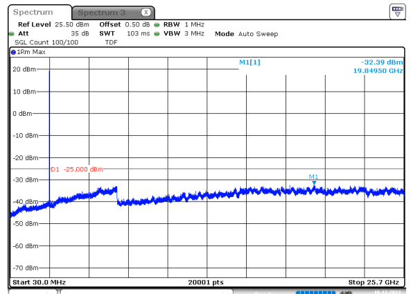
20MHz_15kHz_2560MHz_DFT-s-OFDM QPSK_RB1@105 -32.39 dBm
