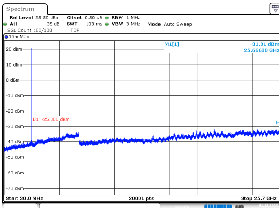
15MHz_15kHz_2562.5MHz_DFT-s-OFDM QPSK_RB1@78 -31.31 dBm
