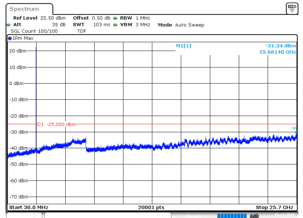
15MHz_15kHz_2535MHz_DFT-s-OFDM QPSK_RB1@78 -31.34 dBm
