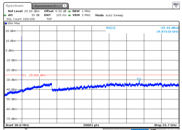
5MHz_15kHz_2502.5MHz_DFT-s-OFDM QPSK_RB25@0 -32.45 dBm
