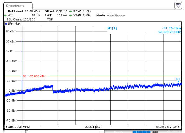
15MHz_15kHz_2562.5MHz_DFT-s-OFDM QPSK_RB75@0 -31.56 dBm
