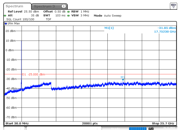
20MHz_15kHz_2535MHz_DFT-s-OFDM QPSK_RB100@0 -31.85 dBm
