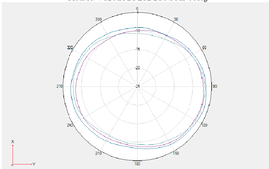
GSM900/WCDMA B8/LTE B8/N8 \Theta=90^\circ
