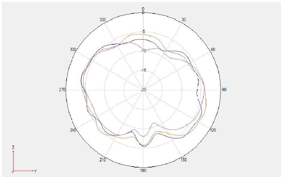
PCS/WCDMA B2/LTE B2 \Phi=90^\circ
