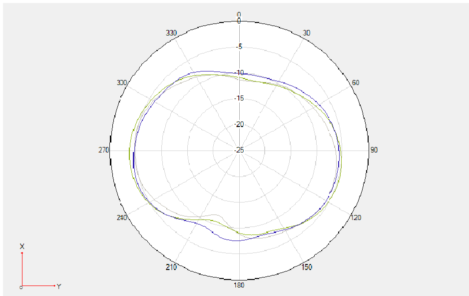
DCS /LTE B3/ N3 \Theta = 90^\circ
