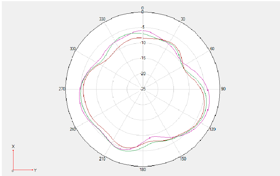
LTE B7/B41/N7/N41 \Theta=90^\circ
