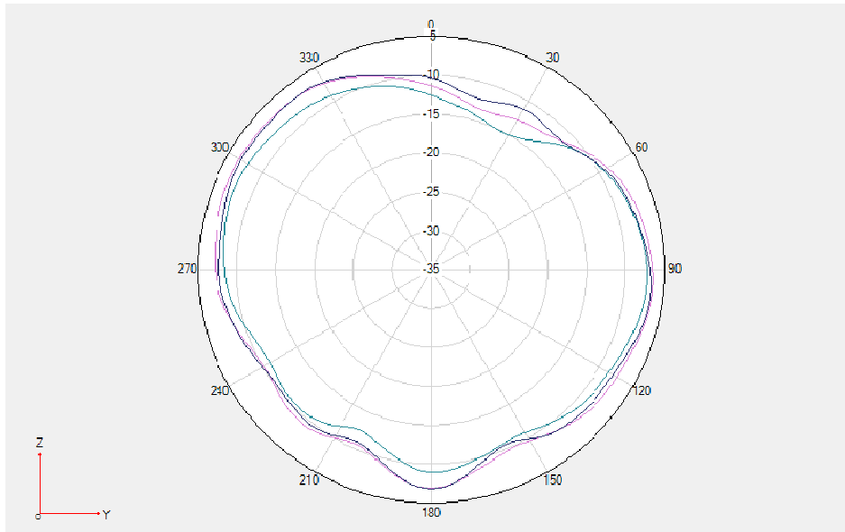
GSM900/WCDMA B8/LTE B8/N8 \Phi=90^\circ
