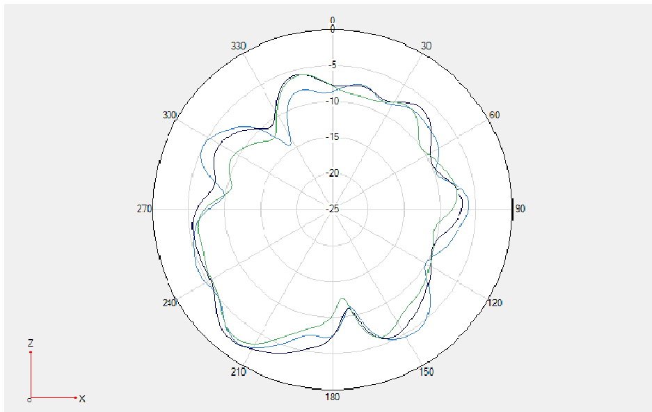
LTE B7/B41/N7/N41 \Phi=0^\circ
