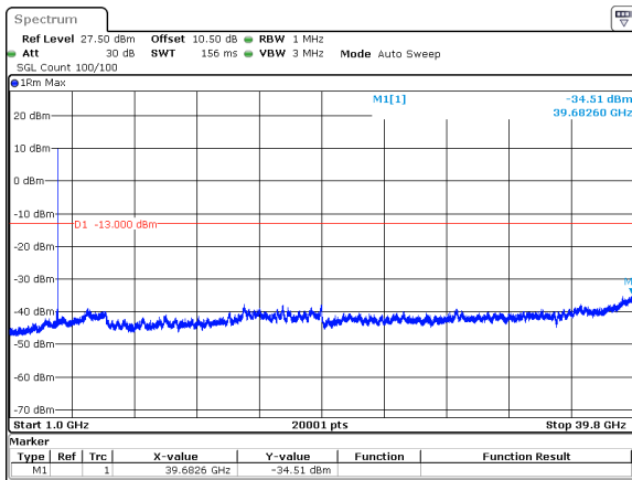
30MHz_15kHz_3965MHz_DFT-s-OFDM QPSK_RB1@159&-34.51 dBm
