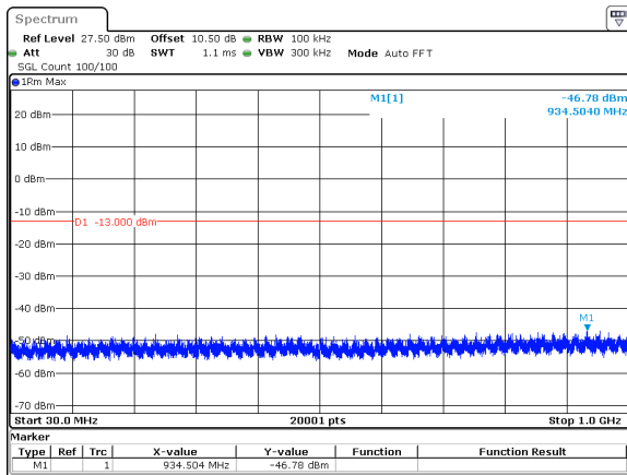
40MHz_15kHz_3840MHz_DFT-s-OFDM QPSK_RB1@215&-46.78 dBm
