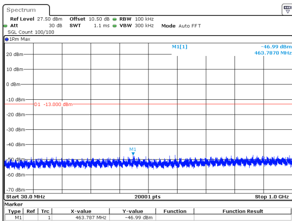
60MHz_30kHz_3840MHz_DFT-s-OFDM QPSK_RB162@0&-46.99 dBm
