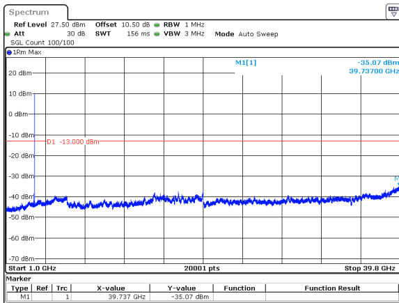
90MHz_30kHz_3745MHz_DFT-s-OFDM QPSK_RB1@244&-35.07 dBm
