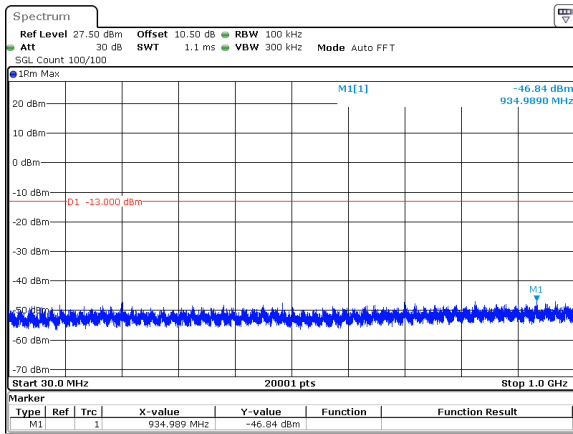
80MHz_30kHz_3740MHz_DFT-s-OFDM QPSK_RB1@0&-46.84 dBm
