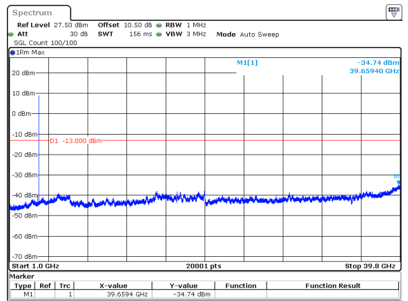
100MHz_30kHz_3840MHz_DFT-s-OFDM QPSK_RB1@272&-34.74 dBm
