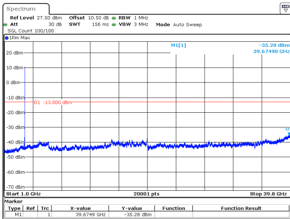
60MHz_30kHz_3730MHz_DFT-s-OFDM QPSK_RB1@161&-35.28 dBm
