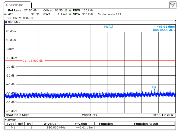
40MHz_15kHz_3720MHz_DFT-s-OFDM QPSK_RB1@0&-46.61 dBm
