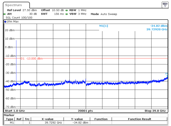
100MHz_30kHz_3930MHz_DFT-s-OFDM QPSK_RB1@0&-34.82 dBm
