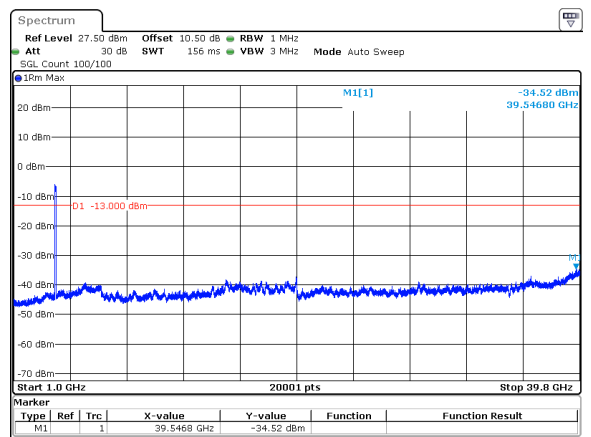
100MHz_30kHz_3840MHz_DFT-s-OFDM QPSK_RB270@0&-34.52 dBm
