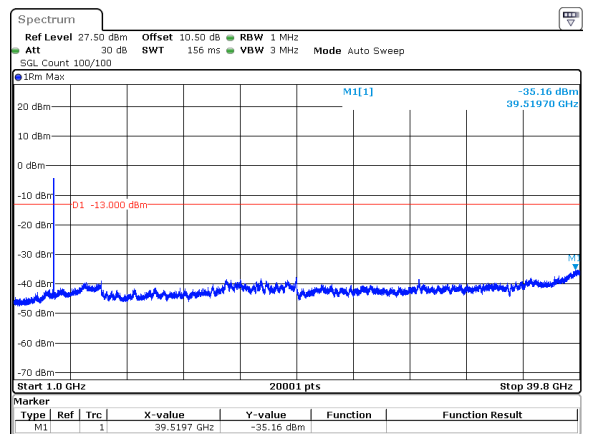
70MHz_30kHz_3735MHz_DFT-s-OFDM QPSK_RB180@0&-35.16 dBm
