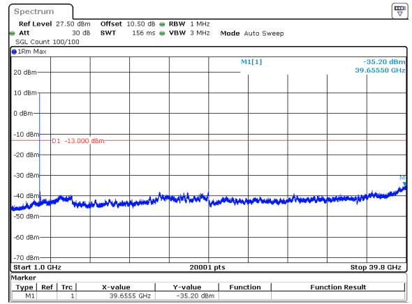
50MHz_30kHz_3840MHz_DFT-s-OFDM QPSK_RB1@0&-35.20 dBm
