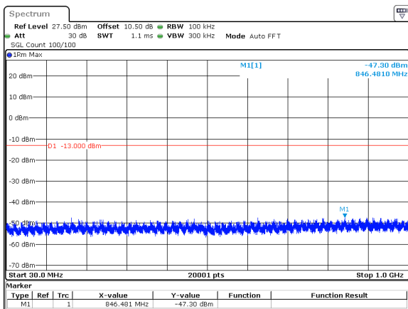
50MHz_30kHz_3725MHz_DFT-s-OFDM QPSK_RB128@0&-47.30 dBm
