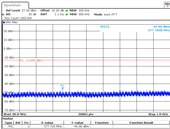
40MHz_30kHz_3720MHz_DFT-s-OFDM QPSK_RB1@105&-45.96 dBm
