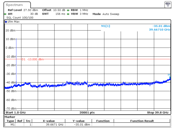
30MHz_15kHz_3715MHz_DFT-s-OFDM QPSK_RB1@0&-35.01 dBm
