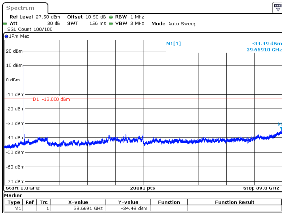
40MHz_30kHz_3720MHz_DFT-s-OFDM QPSK_RB1@0&-34.49 dBm
