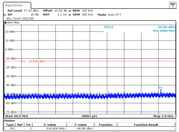
100MHz_30kHz_3840MHz_DFT-s-OFDM QPSK_RB1@0&-46.86 dBm
