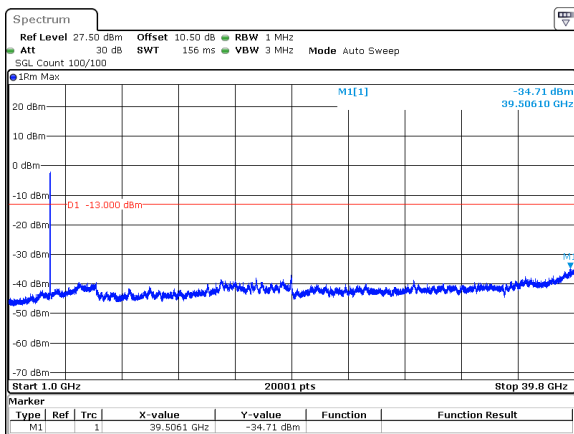
50MHz_15kHz_3840MHz_DFT-s-OFDM QPSK_RB270@0&-34.71 dBm
