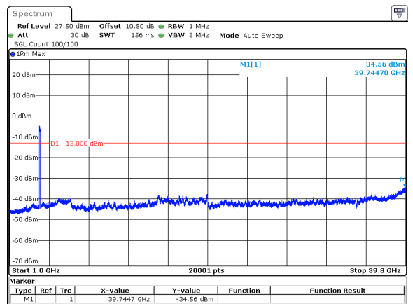
70MHz_30kHz_3945MHz_DFT-s-OFDM QPSK_RB180@0&-34.56 dBm
