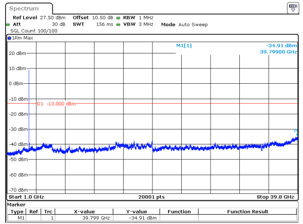
70MHz_30kHz_3945MHz_DFT-s-OFDM QPSK_RB1@0&-34.91 dBm
