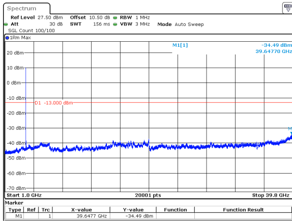
40MHz_15kHz_3840MHz_DFT-s-OFDM QPSK_RB1@0&-34.49 dBm
