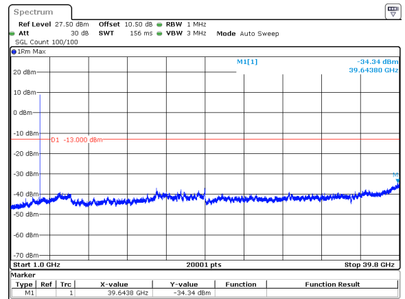
80MHz_30kHz_3840MHz_DFT-s-OFDM QPSK_RB1@216&-34.34 dBm
