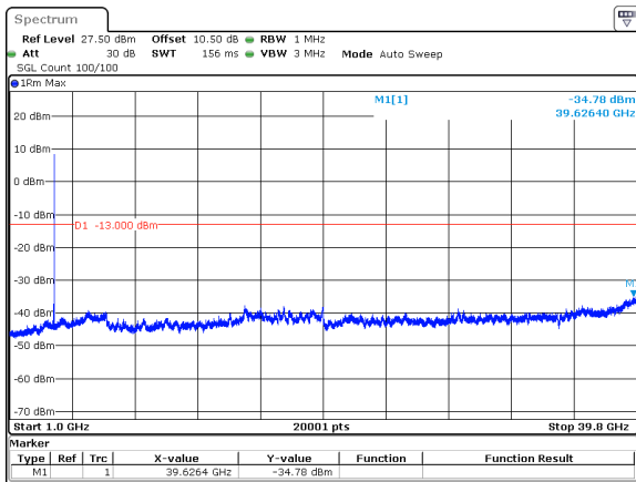
50MHz_30kHz_3725MHz_DFT-s-OFDM QPSK_RB1@132&-34.78 dBm
