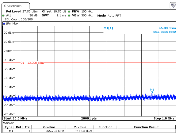
30MHz_15kHz_3840MHz_DFT-s-OFDM QPSK_RB160@0&-46.83 dBm
