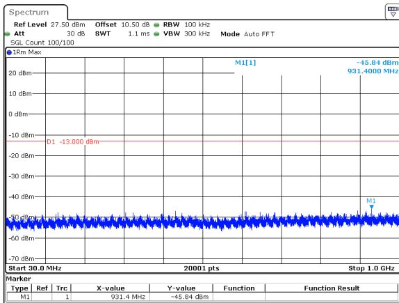
50MHz_15kHz_3840MHz_DFT-s-OFDM QPSK_RB1@269&-45.84 dBm
