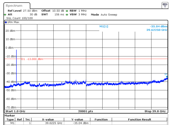
50MHz_30kHz_3840MHz_DFT-s-OFDM QPSK_RB128@0&-35.04 dBm
