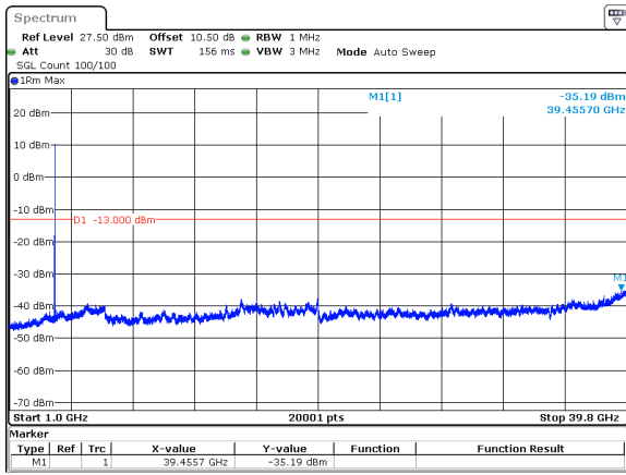
30MHz_15kHz_3840MHz_DFT-s-OFDM QPSK_RB1@0&-35.19 dBm
