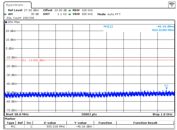
40MHz_30kHz_3840MHz_DFT-s-OFDM QPSK_RB1@0&-46.16 dBm
