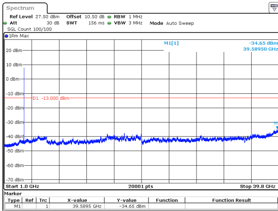
100MHz_30kHz_3750MHz_DFT-s-OFDM QPSK_RB1@272&-34.65 dBm
