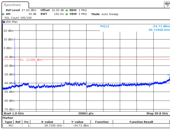
50MHz_15kHz_3840MHz_DFT-s-OFDM QPSK_RB1@0&-34.71 dBm
