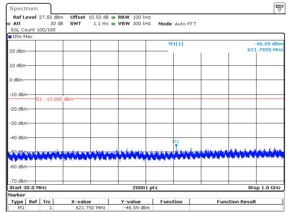
60MHz_30kHz_3730MHz_DFT-s-OFDM QPSK_RB1@161&-46.59 dBm
