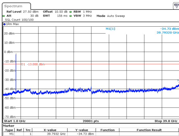
40MHz_15kHz_3840MHz_DFT-s-OFDM QPSK_RB216@0&-34.73 dBm
