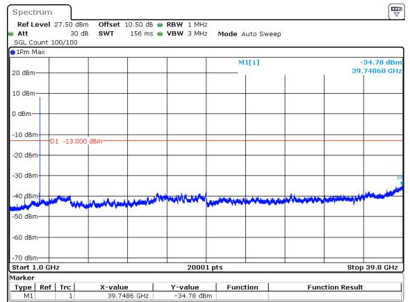
70MHz_30kHz_3945MHz_DFT-s-OFDM QPSK_RB1@188&-34.78 dBm
