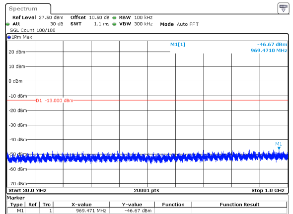
70MHz_30kHz_3840MHz_DFT-s-OFDM QPSK_RB180@0&-46.67 dBm
