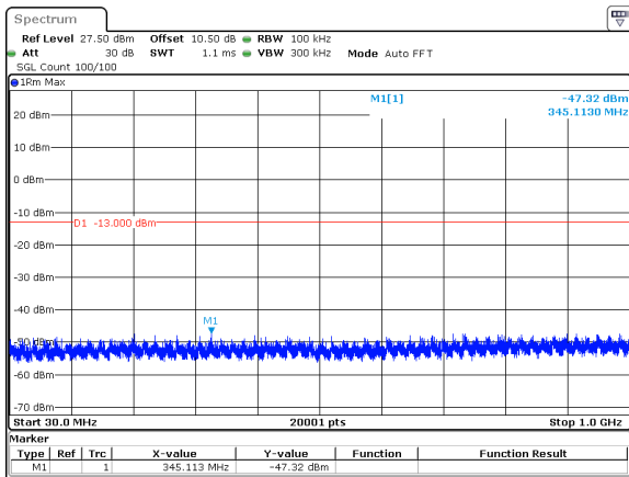
40MHz_30kHz_3960MHz_DFT-s-OFDM QPSK_RB1@105&-47.32 dBm
