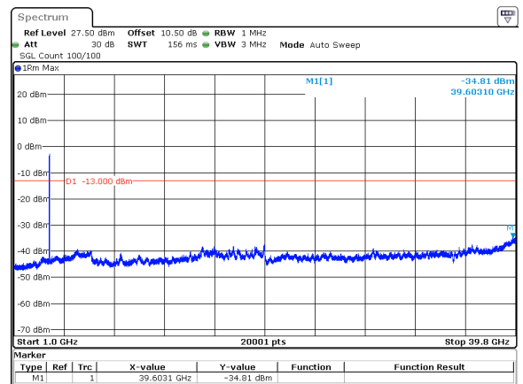
60MHz_30kHz_3730MHz_DFT-s-OFDM QPSK_RB162@0&-34.81 dBm
