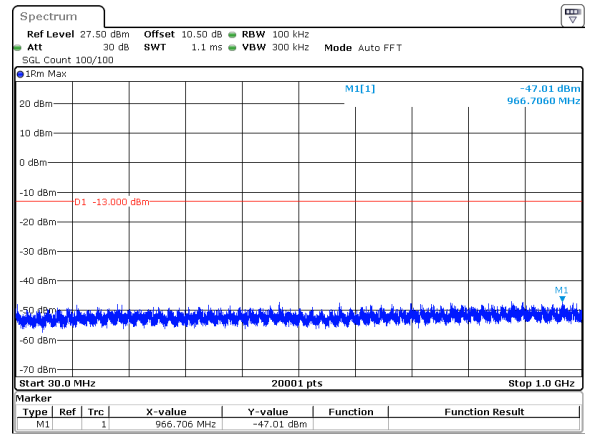
10MHz_30kHz_3545MHz_DFT-s-OFDM QPSK_RB1@0&-47.01 dBm
