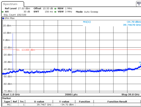
40MHz_15kHz_3960MHz_DFT-s-OFDM QPSK_RB1@0&-34.70 dBm
