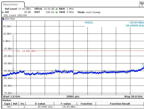
50MHz_15kHz_3955MHz_DFT-s-OFDM QPSK_RB1@269&-35.04 dBm
