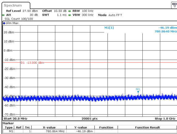
80MHz_30kHz_3740MHz_DFT-s-OFDM QPSK_RB1@216&-46.19 dBm
