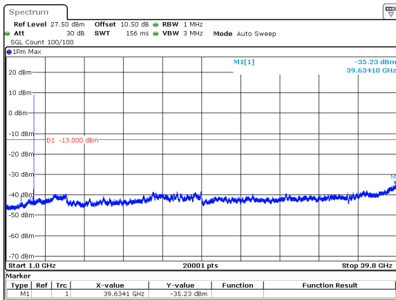
30MHz_15kHz_3715MHz_DFT-s-OFDM QPSK_RB1@159&-35.23 dBm
