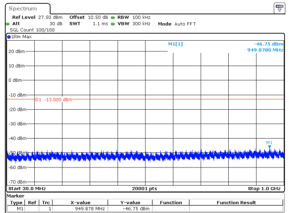
70MHz_30kHz_3840MHz_DFT-s-OFDM QPSK_RB1@188&-46.75 dBm
