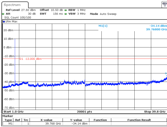
60MHz_30kHz_3950MHz_DFT-s-OFDM QPSK_RB1@0&-34.14 dBm
