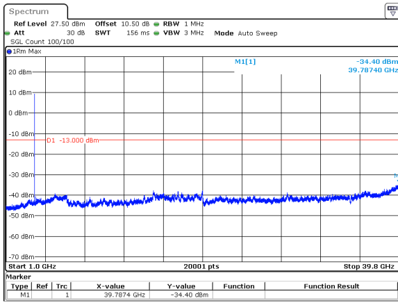
90MHz_30kHz_3840MHz_DFT-s-OFDM QPSK_RB1@0&-34.40 dBm
