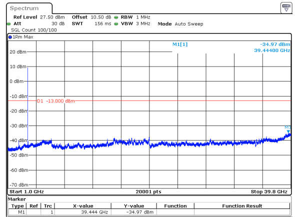
80MHz_30kHz_3740MHz_DFT-s-OFDM QPSK_RB1@0&-34.97 dBm
