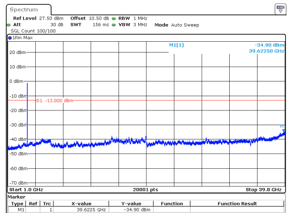
40MHz_15kHz_3720MHz_DFT-s-OFDM QPSK_RB216@0&-34.90 dBm
