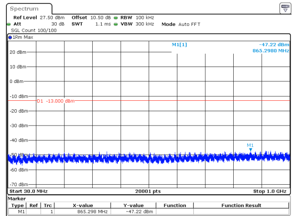
40MHz_30kHz_3840MHz_DFT-s-OFDM QPSK_RB1@105&-47.22 dBm
