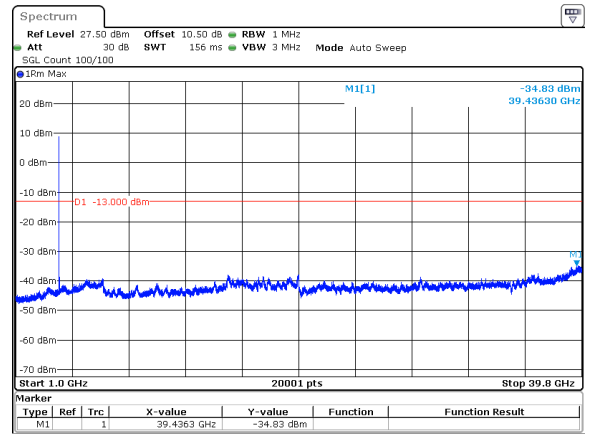
50MHz_30kHz_3955MHz_DFT-s-OFDM QPSK_RB1@0&-34.83 dBm
