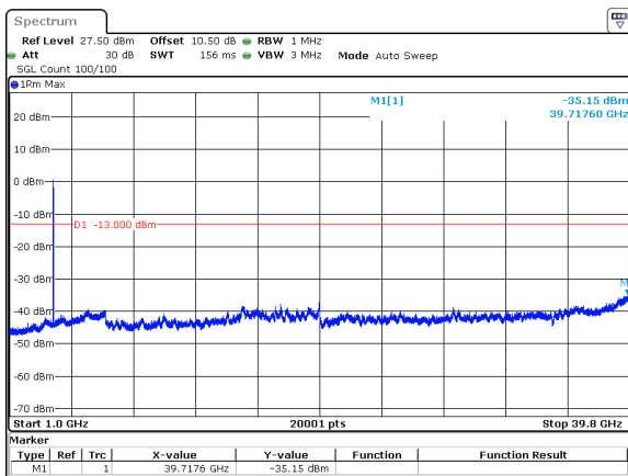
30MHz_15kHz_3715MHz_DFT-s-OFDM QPSK_RB160@0&-35.15 dBm
