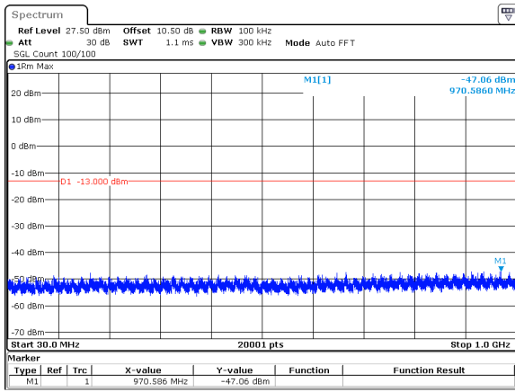
50MHz_30kHz_3840MHz_DFT-s-OFDM QPSK_RB1@0&-47.06 dBm
