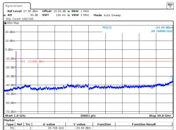
50MHz_15kHz_3725MHz_DFT-s-OFDM QPSK_RB270@0&-34.49 dBm
