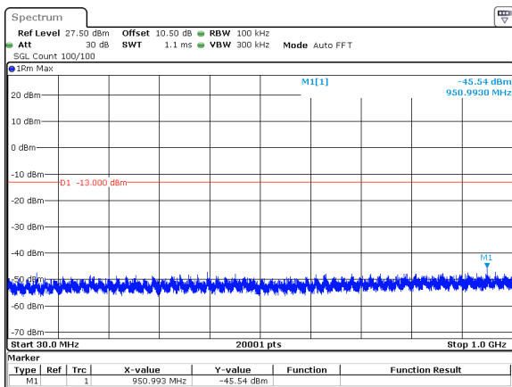
40MHz_30kHz_3840MHz_DFT-s-OFDM QPSK_RB100@0&-45.54 dBm
