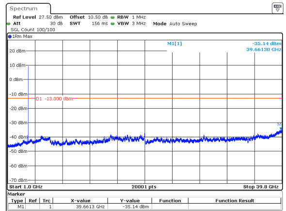
90MHz_30kHz_3840MHz_DFT-s-OFDM QPSK_RB1@244&-35.14 dBm
