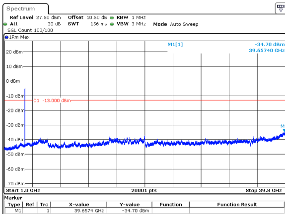
70MHz_30kHz_3840MHz_DFT-s-OFDM QPSK_RB180@0&-34.70 dBm
