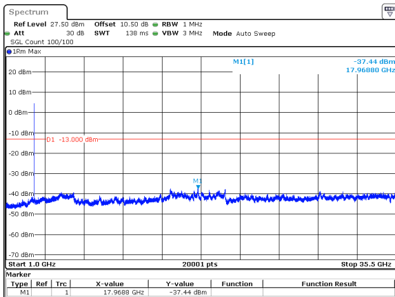
15MHz_15kHz_3500MHz_DFT-s-OFDM QPSK_RB75@0&-37.44 dBm
