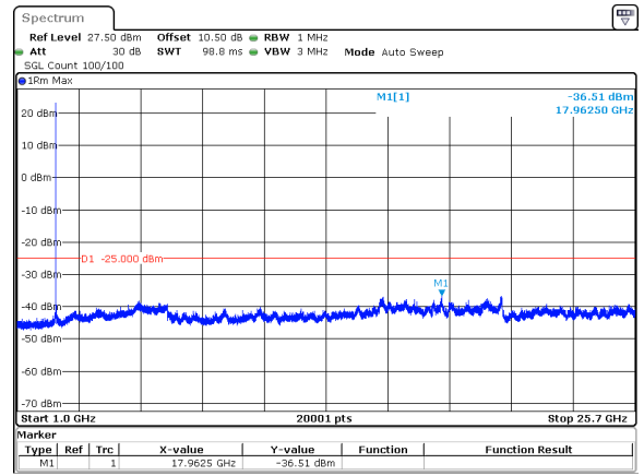
15MHz_15kHz_2535MHz_DFT-s-OFDM QPSK_RB1@0&-36.51 dBm
