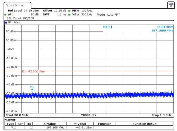
15MHz_15kHz_2507.5MHz_DFT-s-OFDM QPSK_RB1@0&-46.81 dBm
