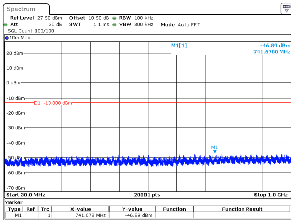
30MHz_15kHz_3465MHz_DFT-s-OFDM QPSK_RB1@159&-46.89 dBm
