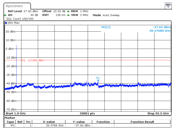
15MHz_30kHz_3457.5MHz_DFT-s-OFDM QPSK_RB36@0&-37.62 dBm
