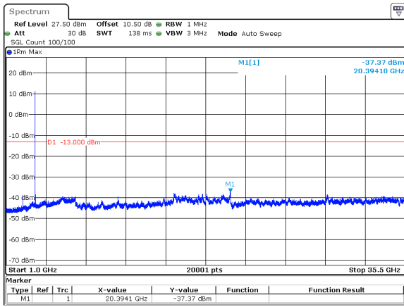
15MHz_30kHz_3500MHz_DFT-s-OFDM QPSK_RB1@0&-37.37 dBm
