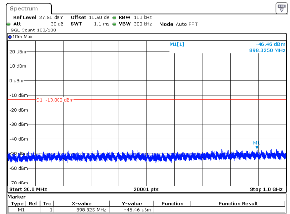
10MHz_15kHz_3500MHz_DFT-s-OFDM QPSK_RB1@51&-46.46 dBm
