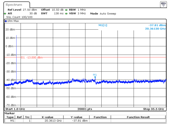
20MHz_15kHz_3540MHz_DFT-s-OFDM QPSK_RB1@0&-37.81 dBm
