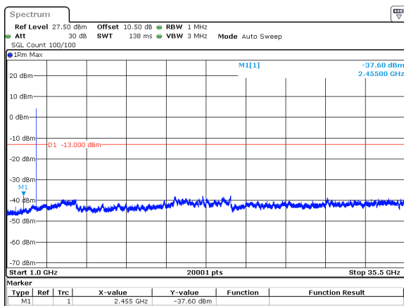
15MHz_30kHz_3542.5MHz_DFT-s-OFDM QPSK_RB36@0&-37.60 dBm
