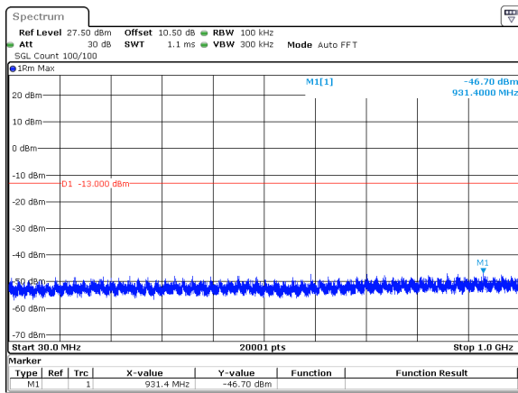
15MHz_30kHz_3457.5MHz_DFT-s-OFDM QPSK_RB1@37&-46.70 dBm
