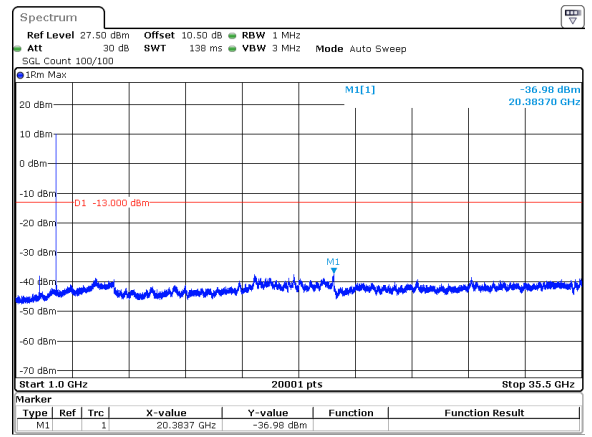
15MHz_30kHz_3457.5MHz_DFT-s-OFDM QPSK_RB1@0&-36.98 dBm
