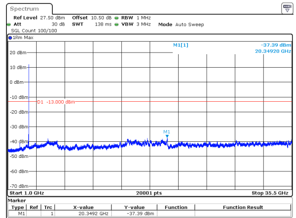
30MHz_15kHz_3500MHz_DFT-s-OFDM QPSK_RB1@159&-37.39 dBm
