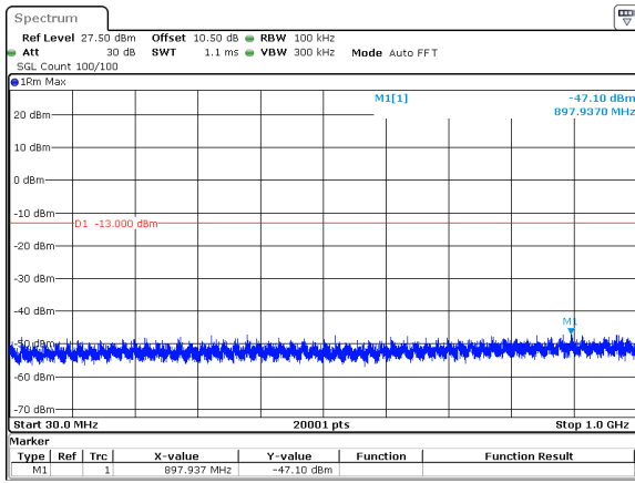
15MHz_15kHz_3500MHz_DFT-s-OFDM QPSK_RB1@0&-47.10 dBm
