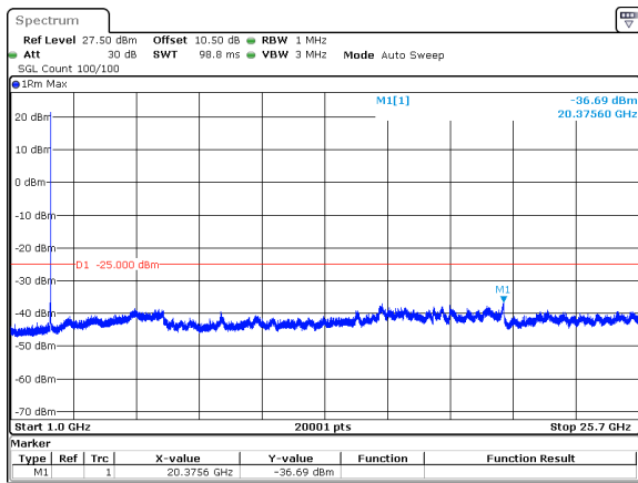
15MHz_15kHz_2562.5MHz_DFT-s-OFDM QPSK_RB1@78&-36.69 dBm
