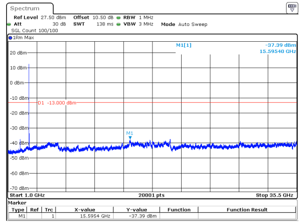
15MHz_15kHz_3500MHz_DFT-s-OFDM QPSK_RB1@0&-37.39 dBm
