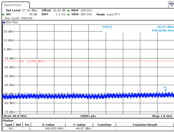
30MHz_15kHz_3535MHz_DFT-s-OFDM QPSK_RB1@0&-46.87 dBm
