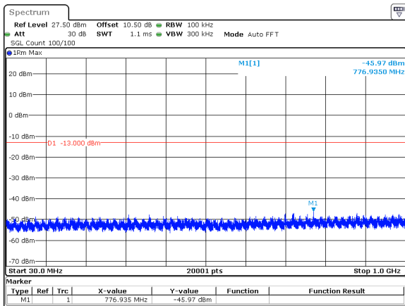
20MHz_15kHz_3460MHz_DFT-s-OFDM QPSK_RB1@105&-45.97 dBm
