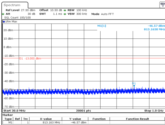
40MHz_30kHz_3530MHz_DFT-s-OFDM QPSK_RB1@105&-46.57 dBm
