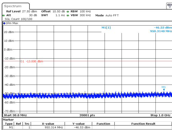
15MHz_15kHz_3457.5MHz_DFT-s-OFDM QPSK_RB75@0&-46.53 dBm
