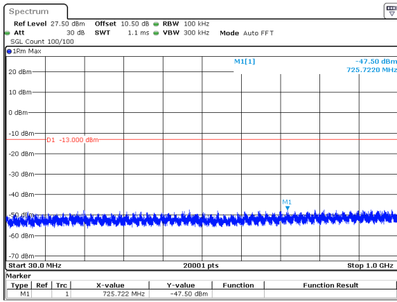
40MHz_15kHz_3500MHz_DFT-s-OFDM QPSK_RB1@0&-47.50 dBm
