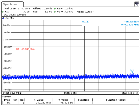
15MHz_30kHz_3500MHz_DFT-s-OFDM QPSK_RB1@37&-46.42 dBm
