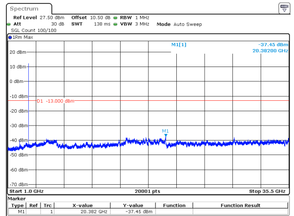
10MHz_15kHz_3545MHz_DFT-s-OFDM QPSK_RB1@51&-37.45 dBm
