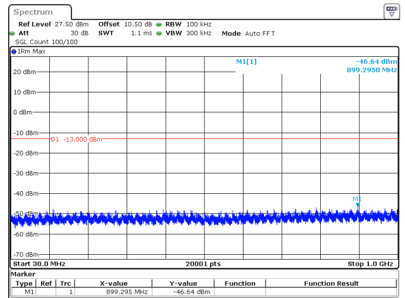
20MHz_15kHz_3540MHz_DFT-s-OFDM QPSK_RB1@105&-46.64 dBm
