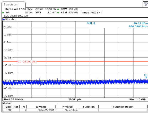
15MHz_15kHz_2562.5MHz_DFT-s-OFDM QPSK_RB1@0&-46.67 dBm
