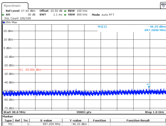
15MHz_15kHz_2535MHz_DFT-s-OFDM QPSK_RB75@0&-46.33 dBm
