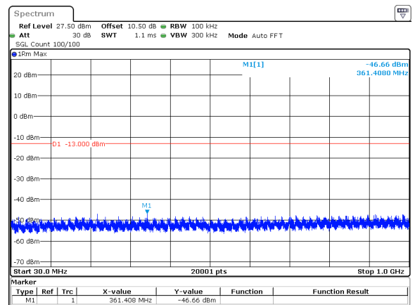
10MHz_30kHz_3545MHz_DFT-s-OFDM QPSK_RB24@0&-46.66 dBm
