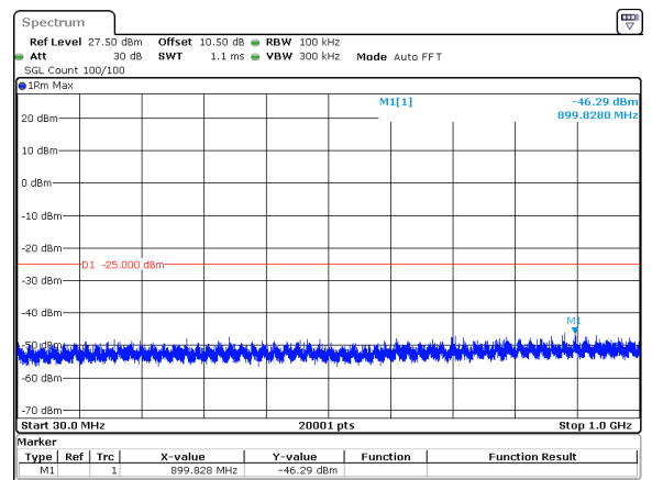
15MHz_15kHz_2562.5MHz_DFT-s-OFDM QPSK_RB75@0&-46.29 dBm
