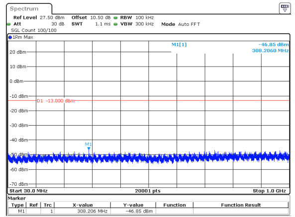
15MHz_15kHz_3457.5MHz_DFT-s-OFDM QPSK_RB1@0&-46.85 dBm
