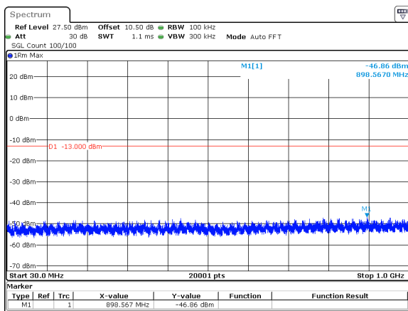
15MHz_30kHz_3457.5MHz_DFT-s-OFDM QPSK_RB36@0&-46.86 dBm
