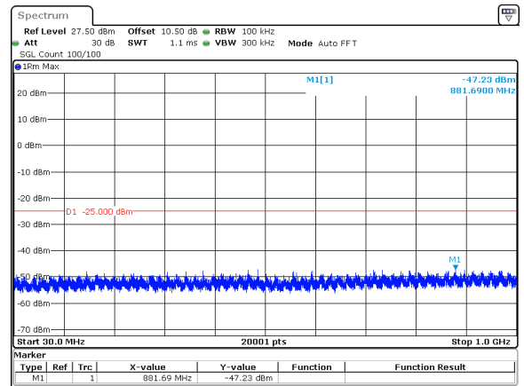
15MHz_15kHz_2535MHz_DFT-s-OFDM QPSK_RB1@78&-47.23 dBm
