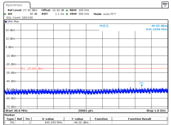
10MHz_15kHz_2565MHz_DFT-s-OFDM QPSK_RB1@51&-46.02 dBm
