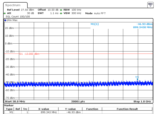
40MHz_15kHz_3500MHz_DFT-s-OFDM QPSK_RB216@0&-46.93 dBm
