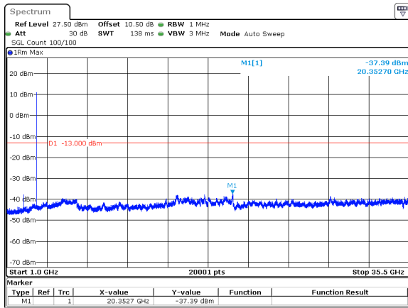
10MHz_30kHz_3545MHz_DFT-s-OFDM QPSK_RB1@0&-37.39 dBm
