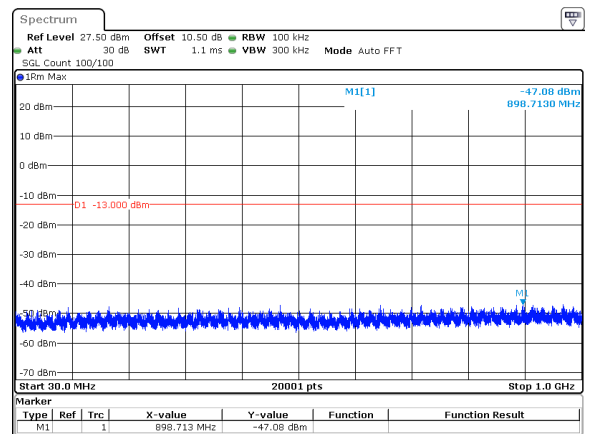
30MHz_15kHz_3465MHz_DFT-s-OFDM QPSK_RB160@0&-47.08 dBm
