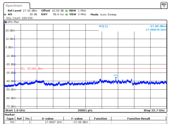
15MHz_15kHz_2535MHz_DFT-s-OFDM QPSK_RB75@0&-37.08 dBm
