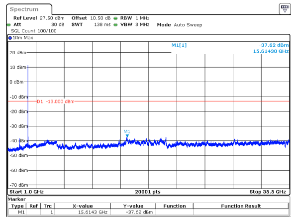
15MHz_15kHz_3457.5MHz_DFT-s-OFDM QPSK_RB1@78&-37.62 dBm
