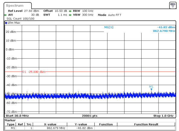
15MHz_15kHz_2562.5MHz_DFT-s-OFDM QPSK_RB1@78&-45.82 dBm
