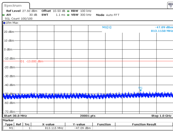
15MHz_15kHz_3457.5MHz_DFT-s-OFDM QPSK_RB1@78&-47.09 dBm
