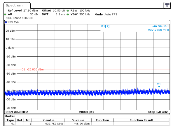
15MHz_15kHz_2507.5MHz_DFT-s-OFDM QPSK_RB1@78&-46.39 dBm
