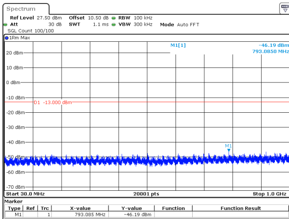
40MHz_30kHz_3500MHz_DFT-s-OFDM QPSK_RB1@105&-46.19 dBm
