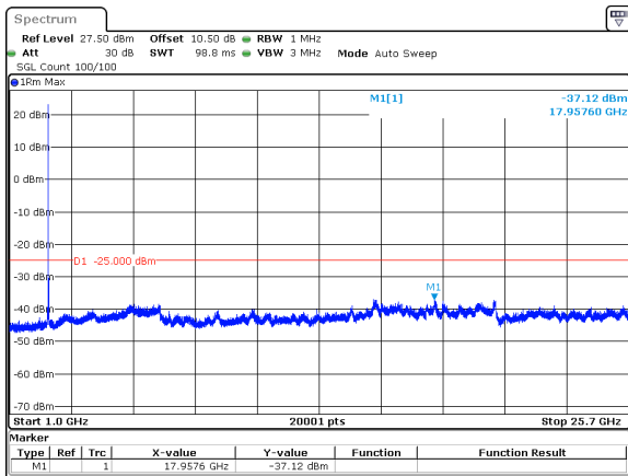
15MHz_15kHz_2535MHz_DFT-s-OFDM QPSK_RB1@78&-37.12 dBm
