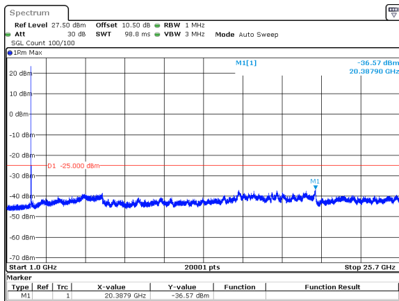
15MHz_15kHz_2507.5MHz_DFT-s-OFDM QPSK_RB1@78&-36.57 dBm
