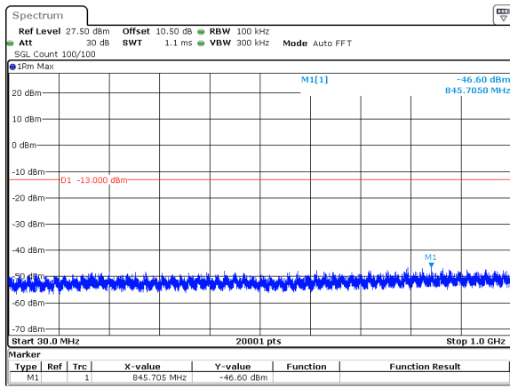
15MHz_15kHz_3542.5MHz_DFT-s-OFDM QPSK_RB1@0&-46.60 dBm
