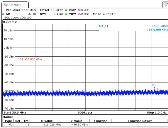
40MHz_30kHz_3500MHz_DFT-s-OFDM QPSK_RB1@0&-46.80 dBm
