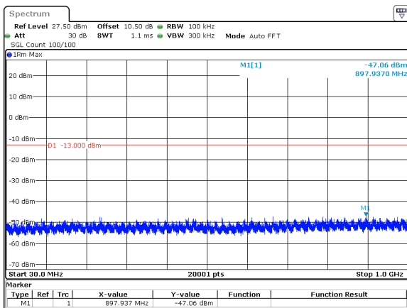
40MHz_30kHz_3530MHz_DFT-s-OFDM QPSK_RB100@0&-47.06 dBm
