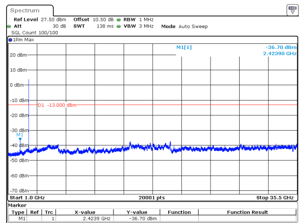
15MHz_15kHz_3457.5MHz_DFT-s-OFDM QPSK_RB75@0&-36.70 dBm
