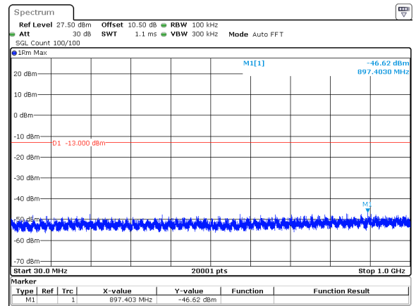
20MHz_15kHz_3500MHz_DFT-s-OFDM QPSK_RB1@105&-46.62 dBm
