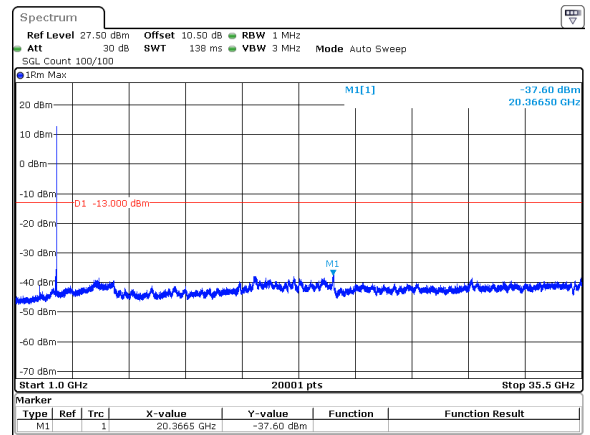
30MHz_15kHz_3465MHz_DFT-s-OFDM QPSK_RB1@159&-37.60 dBm
