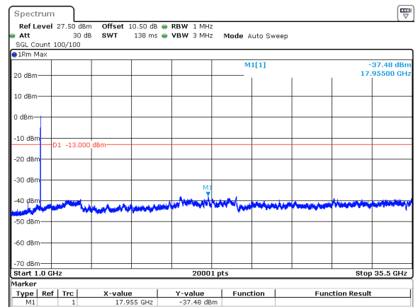
40MHz_30kHz_3530MHz_DFT-s-OFDM QPSK_RB100@0&-37.48 dBm
