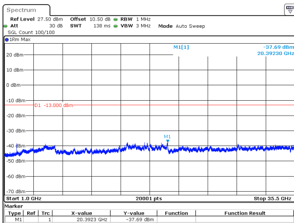
15MHz_30kHz_3500MHz_DFT-s-OFDM QPSK_RB36@0&-37.69 dBm
