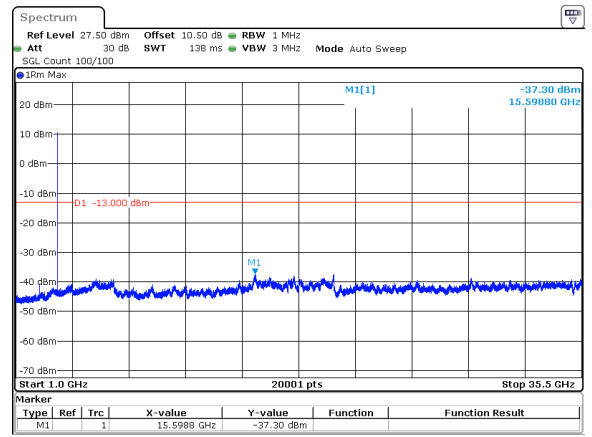
15MHz_15kHz_3542.5MHz_DFT-s-OFDM QPSK_RB1@0&-37.30 dBm
