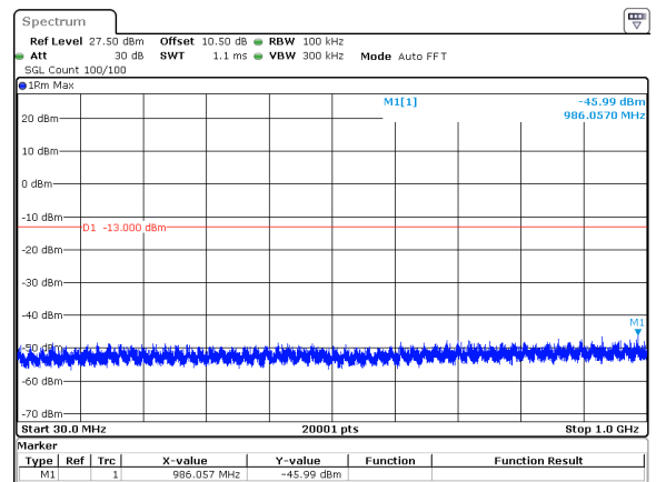
40MHz_30kHz_3470MHz_DFT-s-OFDM QPSK_RB100@0&-45.99 dBm
