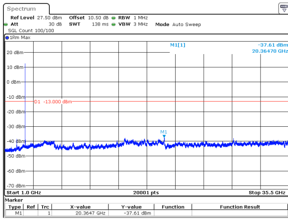
15MHz_15kHz_3457.5MHz_DFT-s-OFDM QPSK_RB1@0&-37.61 dBm
