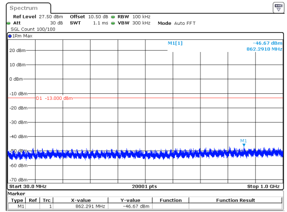
15MHz_30kHz_3500MHz_DFT-s-OFDM QPSK_RB1@0&-46.67 dBm
