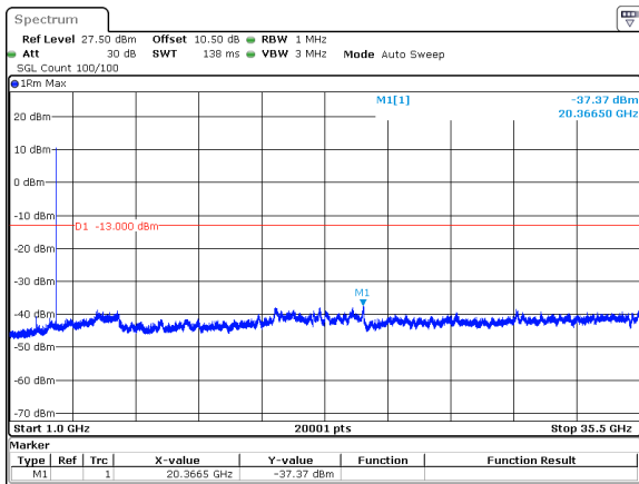
20MHz_15kHz_3540MHz_DFT-s-OFDM QPSK_RB1@105&-37.37 dBm
