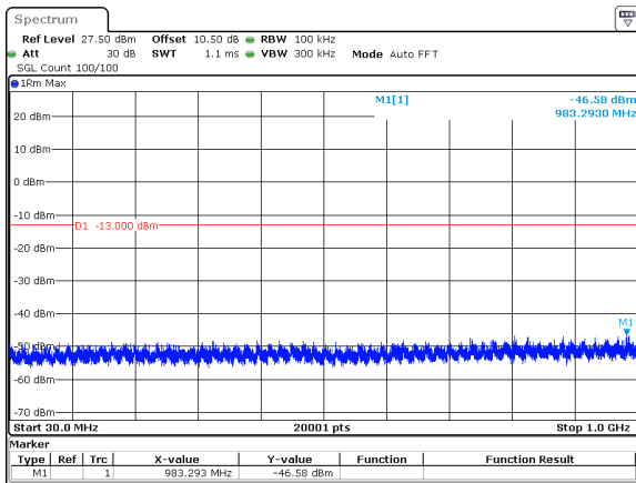
40MHz_30kHz_3470MHz_DFT-s-OFDM QPSK_RB1@105&-46.58 dBm
