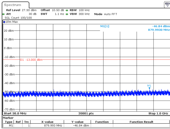
10MHz_15kHz_3545MHz_DFT-s-OFDM QPSK_RB1@0&-46.84 dBm
