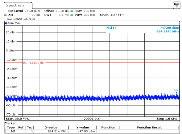
30MHz_15kHz_3535MHz_DFT-s-OFDM QPSK_RB1@159&-47.00 dBm
