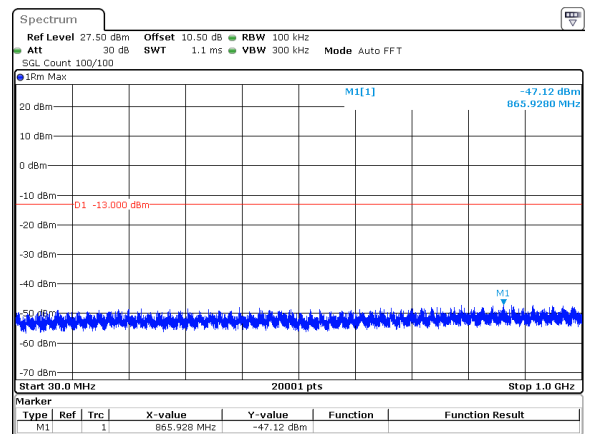
40MHz_30kHz_3500MHz_DFT-s-OFDM QPSK_RB100@0&-47.12 dBm
