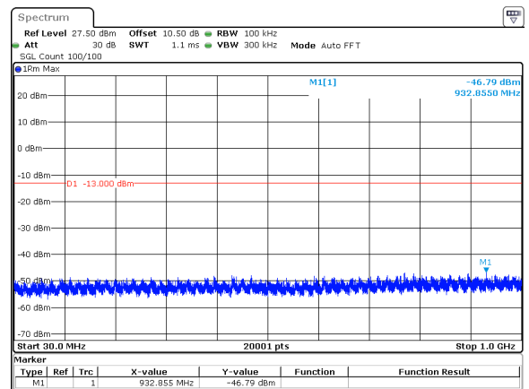
30MHz_15kHz_3535MHz_DFT-s-OFDM QPSK_RB160@0&-46.79 dBm
