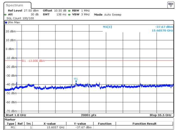
40MHz_30kHz_3470MHz_DFT-s-OFDM QPSK_RB1@105&-37.67 dBm
