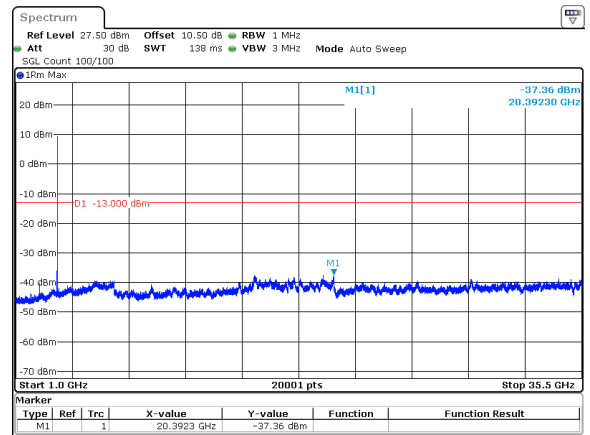
40MHz_30kHz_3530MHz_DFT-s-OFDM QPSK_RB1@105&-37.36 dBm
