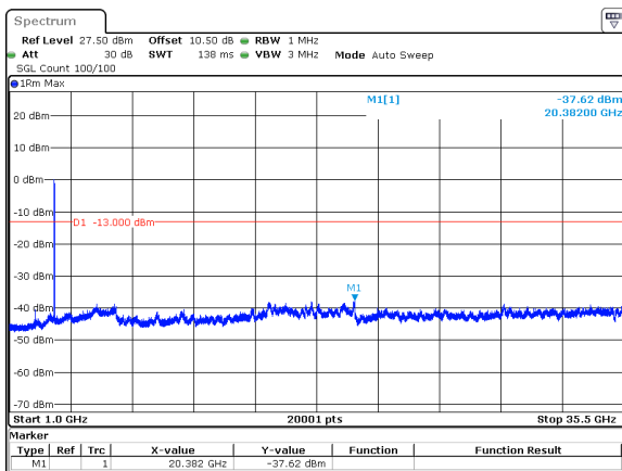
40MHz_30kHz_3500MHz_DFT-s-OFDM QPSK_RB100@0&-37.62 dBm
