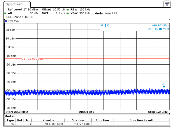
15MHz_15kHz_3500MHz_DFT-s-OFDM QPSK_RB1@78&-46.97 dBm
