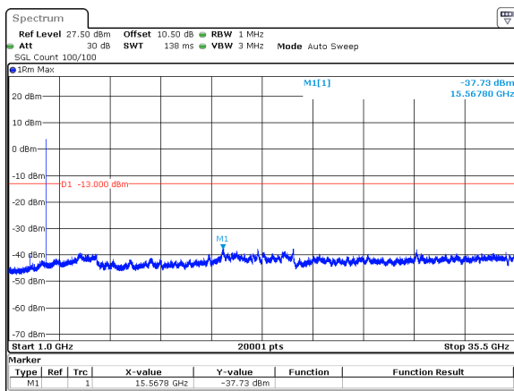
15MHz_15kHz_3542.5MHz_DFT-s-OFDM QPSK_RB75@0&-37.73 dBm
