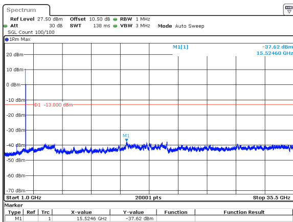
40MHz_15kHz_3500MHz_DFT-s-OFDM QPSK_RB216@0&-37.62 dBm
