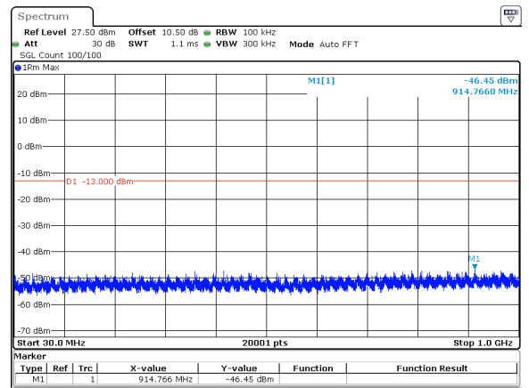
15MHz_30kHz_3542.5MHz_DFT-s-OFDM QPSK_RB1@37&-46.45 dBm
