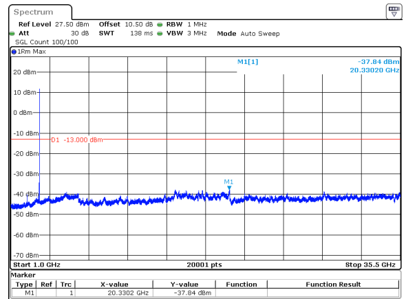
40MHz_15kHz_3500MHz_DFT-s-OFDM QPSK_RB1@215&-37.84 dBm
