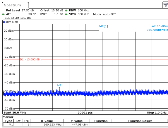
15MHz_30kHz_3457.5MHz_DFT-s-OFDM QPSK_RB1@0&-47.05 dBm
