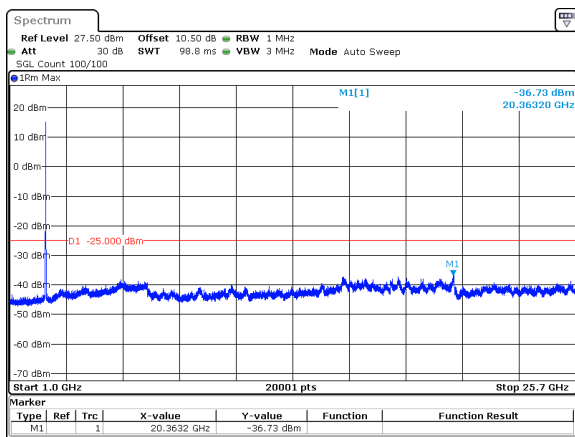
15MHz_15kHz_2562.5MHz_DFT-s-OFDM QPSK_RB75@0&-36.73 dBm
