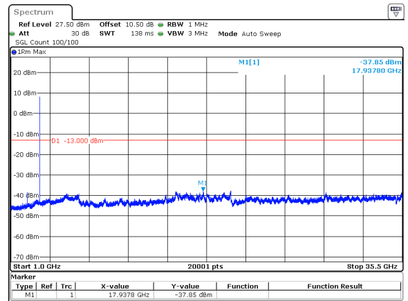
10MHz_30kHz_3545MHz_DFT-s-OFDM QPSK_RB1@23&-37.85 dBm
