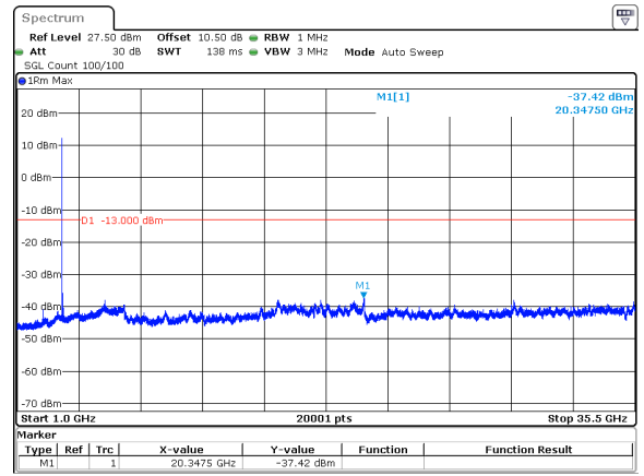
40MHz_15kHz_3500MHz_DFT-s-OFDM QPSK_RB1@0&-37.42 dBm
