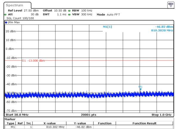
15MHz_15kHz_3500MHz_DFT-s-OFDM QPSK_RB75@0&-46.82 dBm
