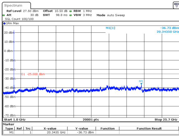
15MHz_15kHz_2507.5MHz_DFT-s-OFDM QPSK_RB1@0&-36.73 dBm
