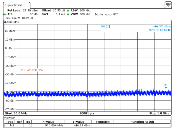
10MHz_15kHz_2535MHz_DFT-s-OFDM QPSK_RB1@51&-46.27 dBm
