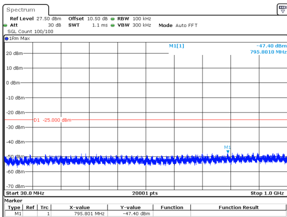
20MHz_15kHz_2535MHz_DFT-s-OFDM QPSK_RB100@0&-47.40 dBm
