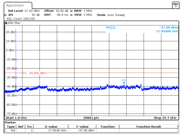
15MHz_15kHz_2562.5MHz_DFT-s-OFDM QPSK_RB1@0&-37.08 dBm
