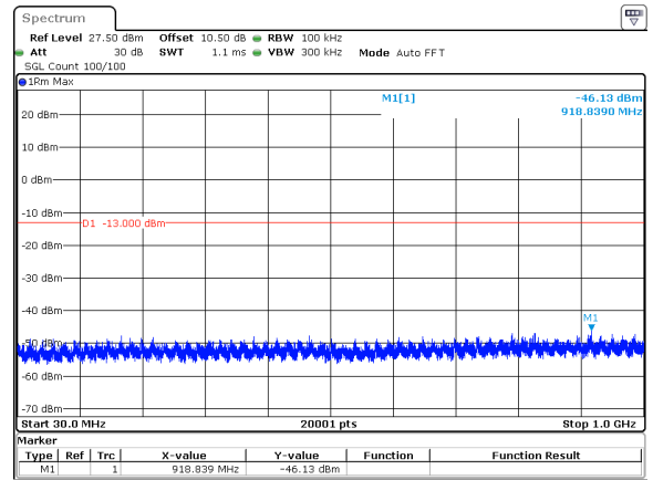
30MHz_15kHz_3500MHz_DFT-s-OFDM QPSK_RB1@0&-46.13 dBm
