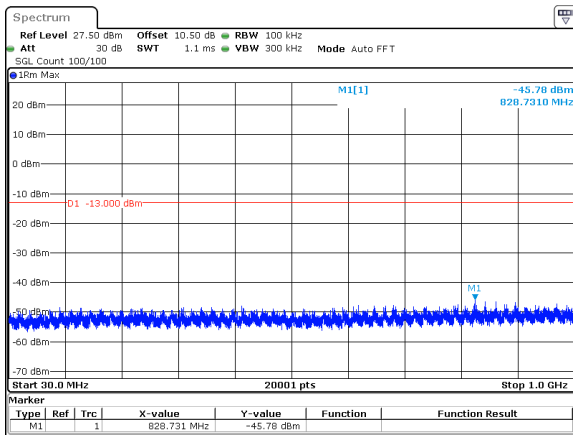
30MHz_15kHz_3500MHz_DFT-s-OFDM QPSK_RB1@159&-45.78 dBm
