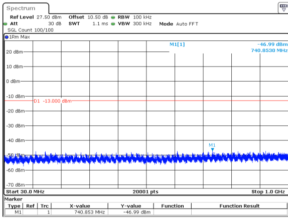
20MHz_15kHz_3540MHz_DFT-s-OFDM QPSK_RB1@0&-46.99 dBm
