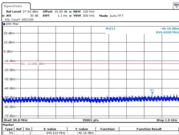
40MHz_15kHz_3530MHz_DFT-s-OFDM QPSK_RB216@0&-46.16 dBm
