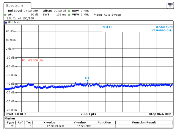
15MHz_15kHz_3542.5MHz_DFT-s-OFDM QPSK_RB1@78&-37.58 dBm
