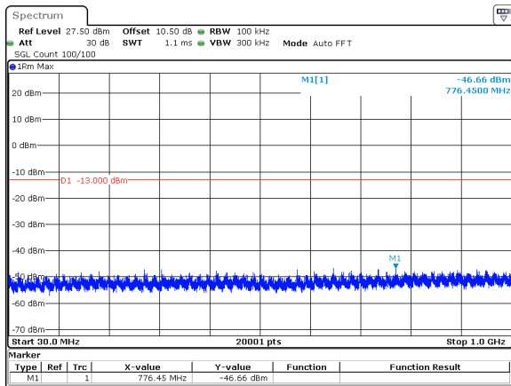
10MHz_15kHz_3545MHz_DFT-s-OFDM QPSK_RB1@51&-46.66 dBm
