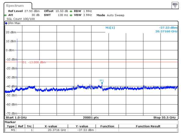
15MHz_30kHz_3457.5MHz_DFT-s-OFDM QPSK_RB1@37&-37.53 dBm
