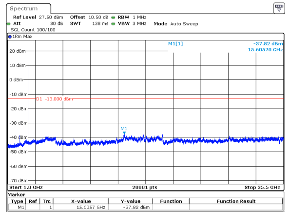
15MHz_30kHz_3542.5MHz_DFT-s-OFDM QPSK_RB1@0&-37.82 dBm
