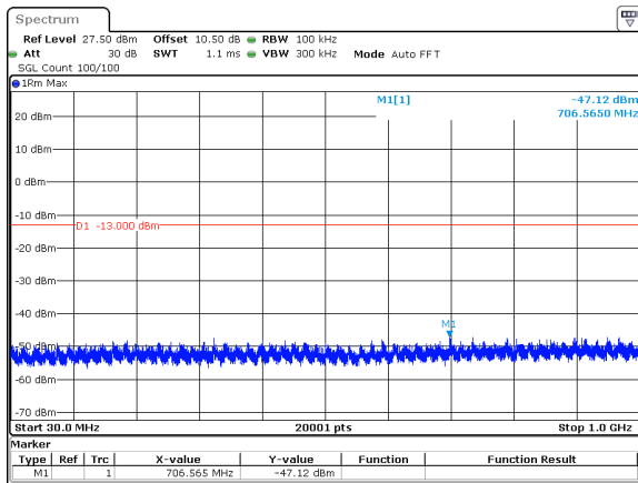
10MHz_30kHz_3545MHz_DFT-s-OFDM QPSK_RB1@23&-47.12 dBm
