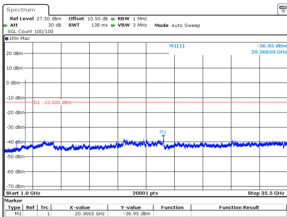
30MHz_15kHz_3535MHz_DFT-s-OFDM QPSK_RB160@0&-36.95 dBm
