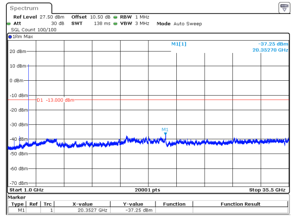
10MHz_15kHz_3545MHz_DFT-s-OFDM QPSK_RB1@0&-37.25 dBm
