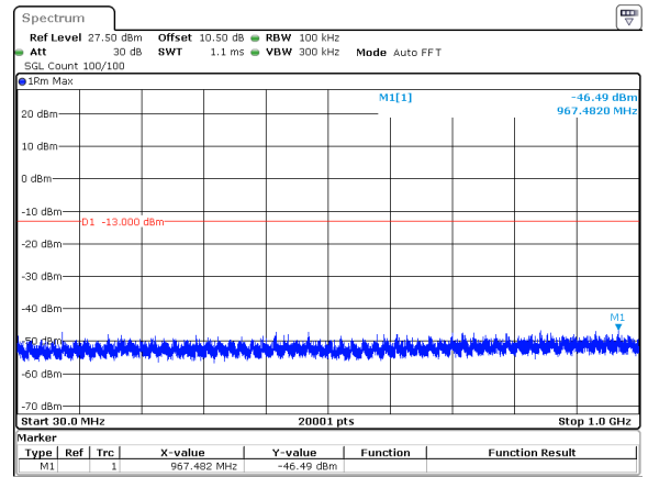
10MHz_30kHz_3545MHz_DFT-s-OFDM QPSK_RB1@0&-46.49 dBm
