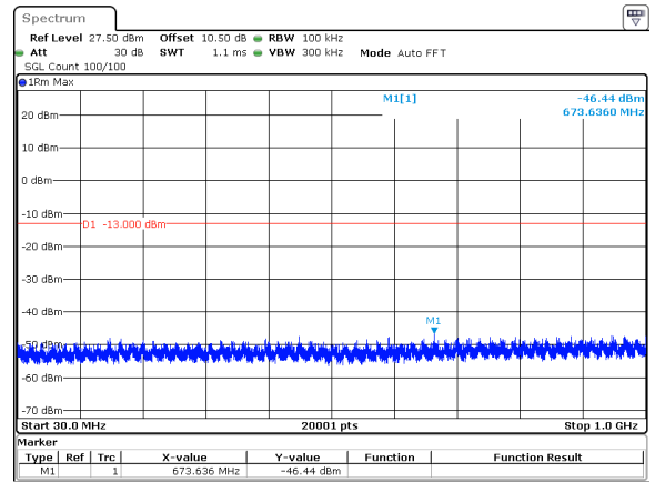
40MHz_15kHz_3530MHz_DFT-s-OFDM QPSK_RB1@0&-46.44 dBm
