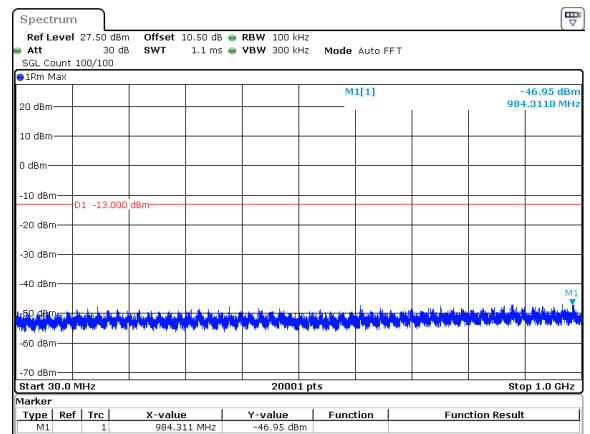
15MHz_30kHz_3500MHz_DFT-s-OFDM QPSK_RB36@0&-46.95 dBm
