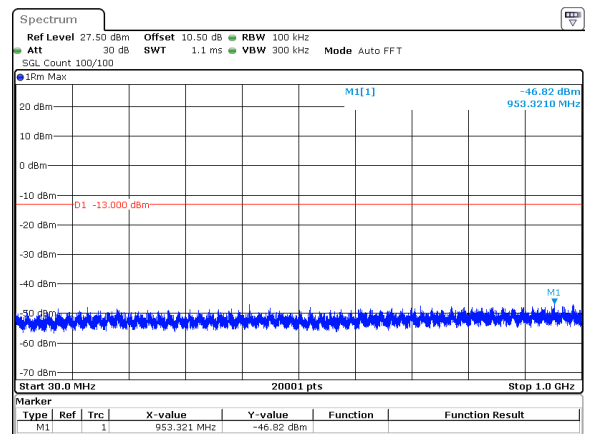
30MHz_15kHz_3500MHz_DFT-s-OFDM QPSK_RB160@0&-46.82 dBm
