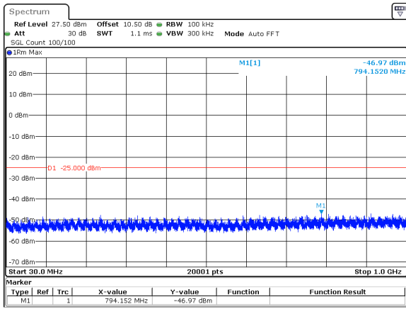
15MHz_15kHz_2535MHz_DFT-s-OFDM QPSK_RB1@0&-46.97 dBm
