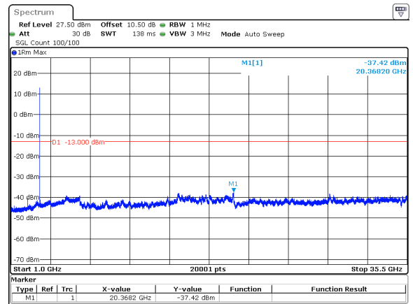
15MHz_30kHz_3500MHz_DFT-s-OFDM QPSK_RB1@37&-37.42 dBm
