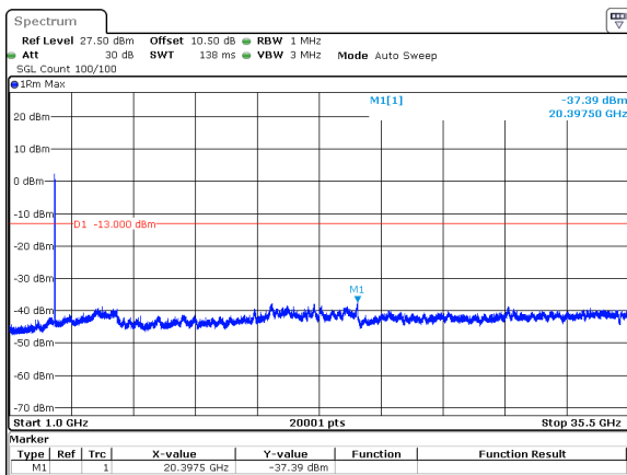
30MHz_15kHz_3500MHz_DFT-s-OFDM QPSK_RB160@0&-37.39 dBm
