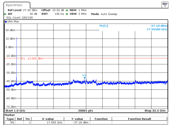
40MHz_30kHz_3500MHz_DFT-s-OFDM QPSK_RB1@105&-37.18 dBm
