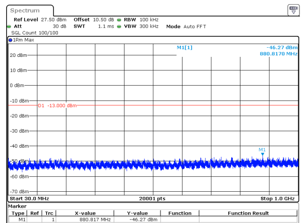
15MHz_30kHz_3542.5MHz_DFT-s-OFDM QPSK_RB36@0&-46.27 dBm
