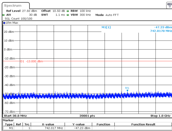
15MHz_15kHz_3542.5MHz_DFT-s-OFDM QPSK_RB1@78&-47.23 dBm
