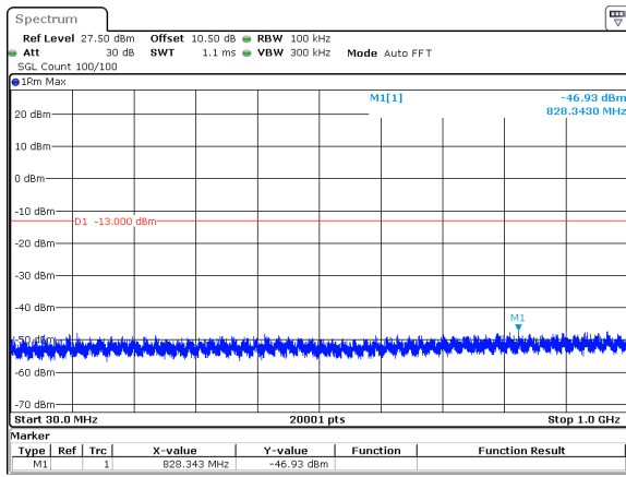
15MHz_30kHz_3542.5MHz_DFT-s-OFDM QPSK_RB1@0&-46.93 dBm
