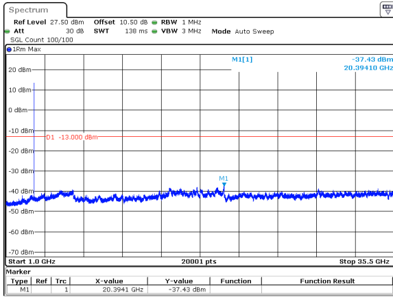
15MHz_15kHz_3500MHz_DFT-s-OFDM QPSK_RB1@78&-37.43 dBm
