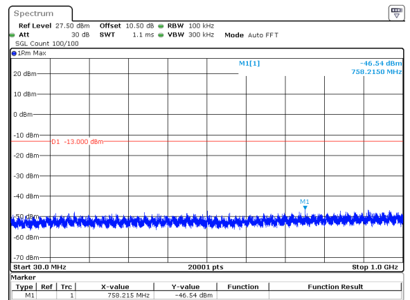
20MHz_15kHz_3540MHz_DFT-s-OFDM QPSK_RB100@0&-46.54 dBm
