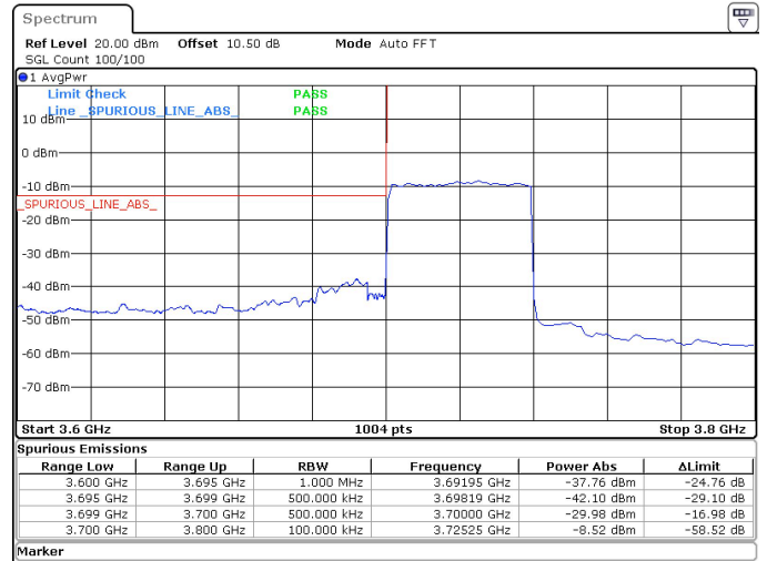
40MHz_15kHz_3720MHz_DFT-s-OFDM QPSK_RB216@0 -29.98 dBm
