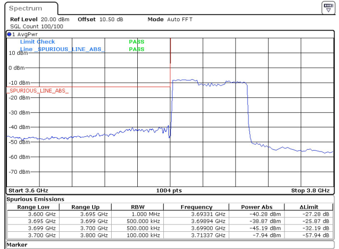
50MHz_30kHz_3725MHz_DFT-s-OFDM QPSK_RB128@0 -38.87 dBm
