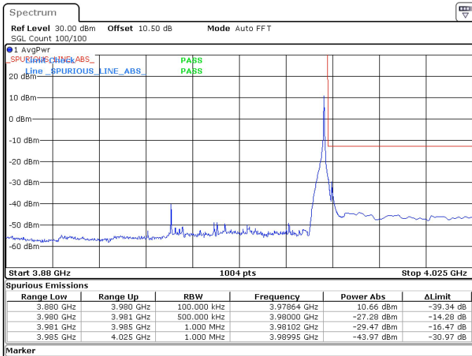
50MHz_30kHz_3955MHz_DFT-s-OFDM QPSK_RB1@132 -27.28 dBm
