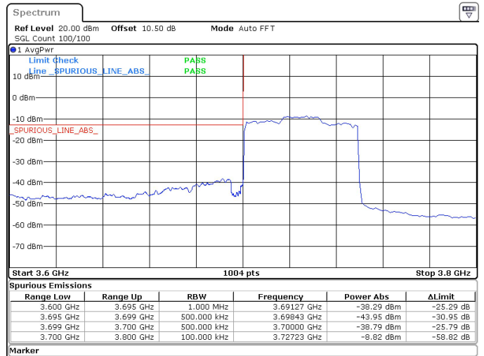
50MHz_15kHz_3725MHz_DFT-s-OFDM QPSK_RB270@0 -38.29 dBm
