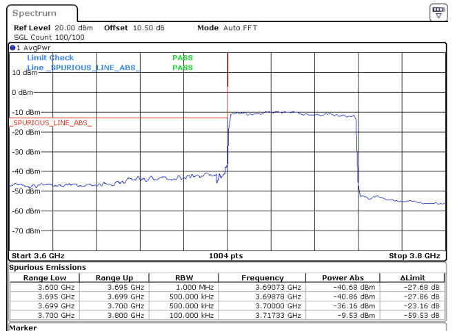
60MHz_30kHz_3730MHz_DFT-s-OFDM QPSK_RB162@0 -36.16 dBm
